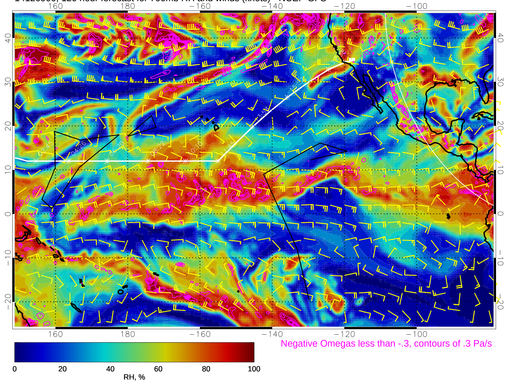
14120900, 120 hour forecast for 700mb RH and winds (knots) - NCEP GFS
