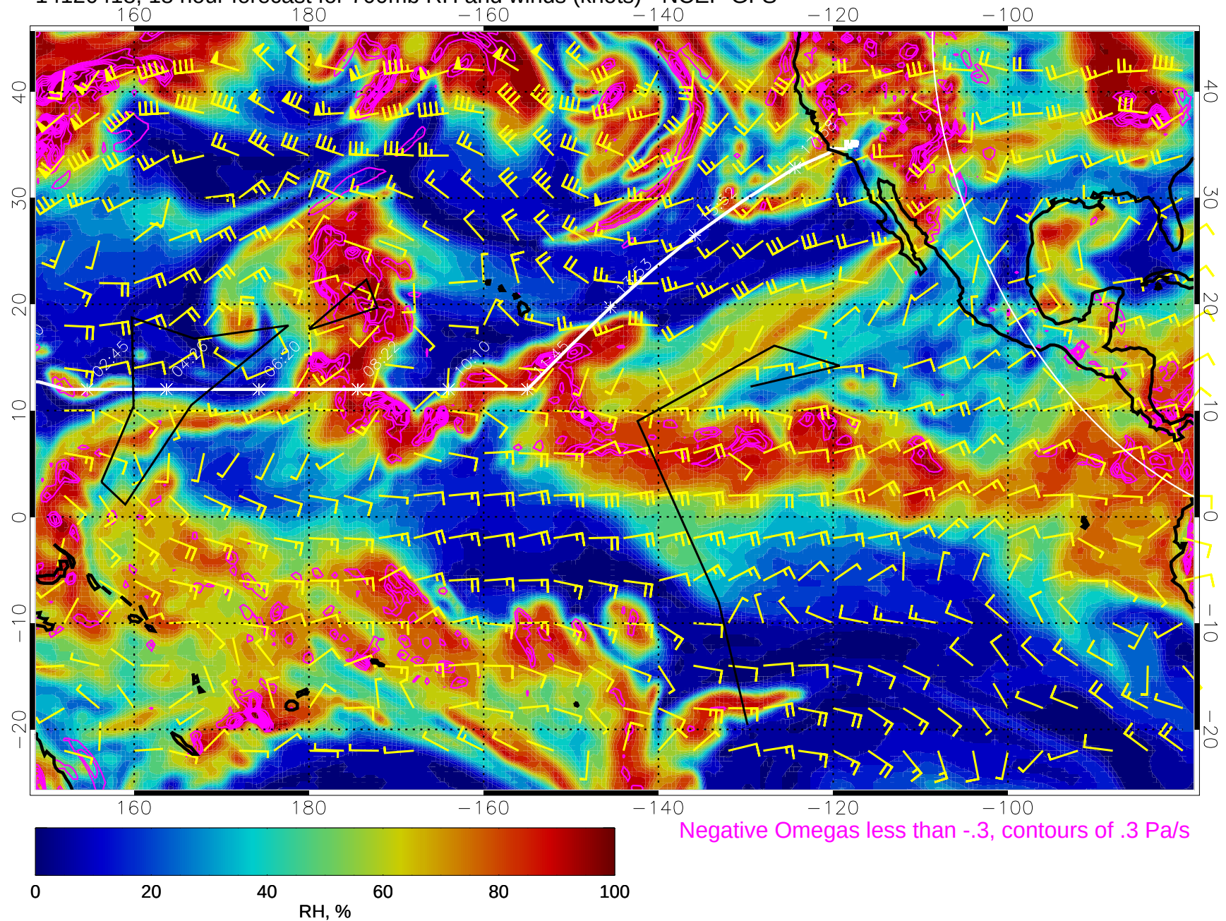
14120418, 18 hour forecast for 700mb RH and winds (knots) - NCEP GFS
