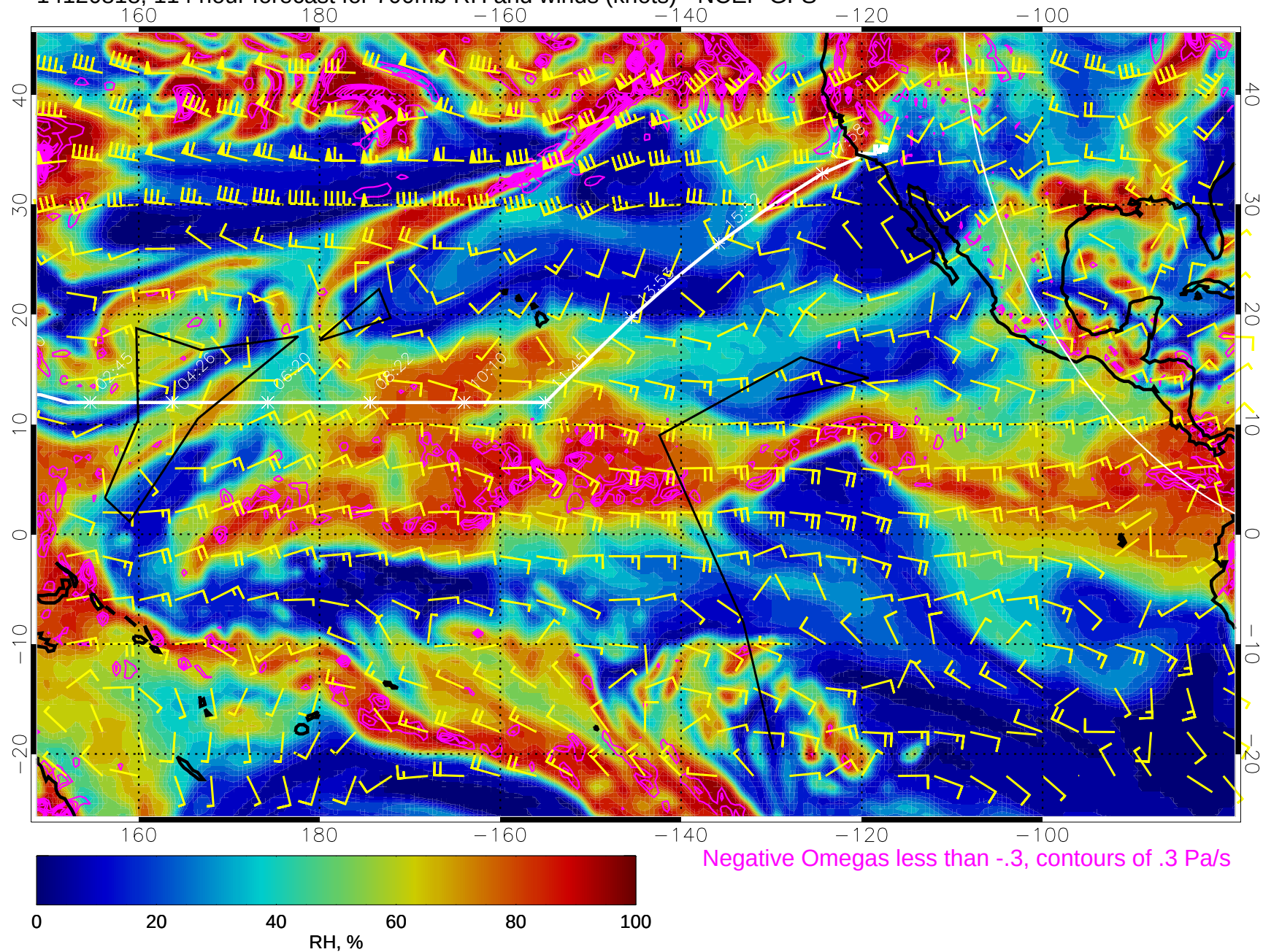
14120818, 114 hour forecast for 700mb RH and winds (knots) - NCEP GFS
