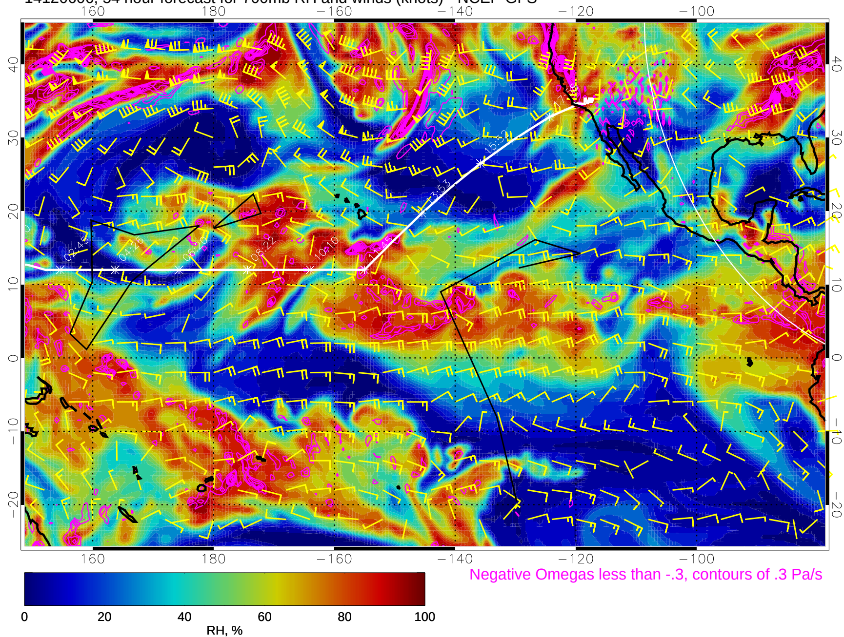
14120606, 54 hour forecast for 700mb RH and winds (knots) - NCEP GFS
