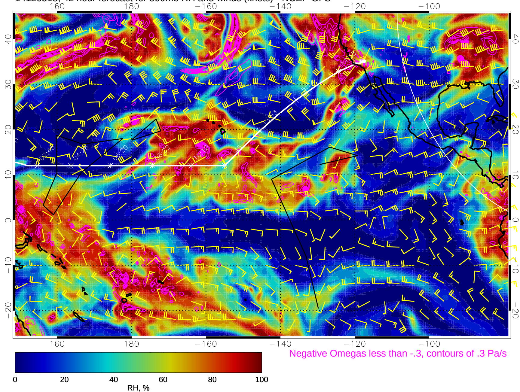
14120518, 42 hour forecast for 500mb RH and winds (knots) - NCEP GFS
