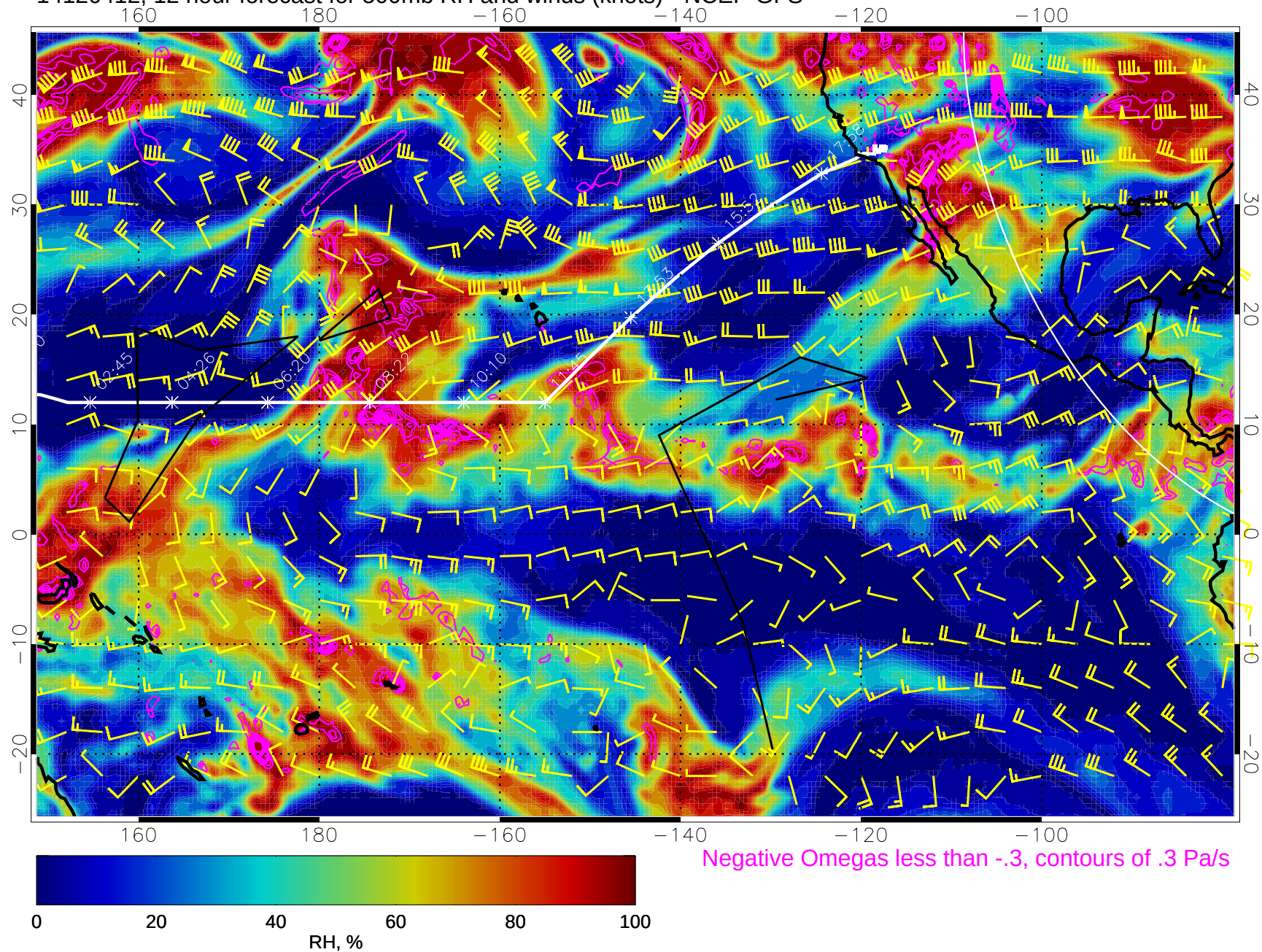
14120412, 12 hour forecast for 500mb RH and winds (knots) - NCEP GFS
