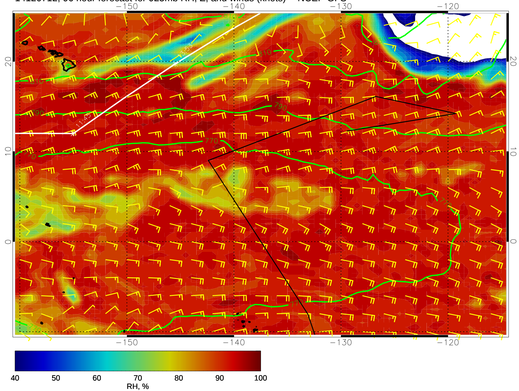
14120712, 96 hour forecast for 925mb RH, Z, and winds (knots) -- NCEP GFS
