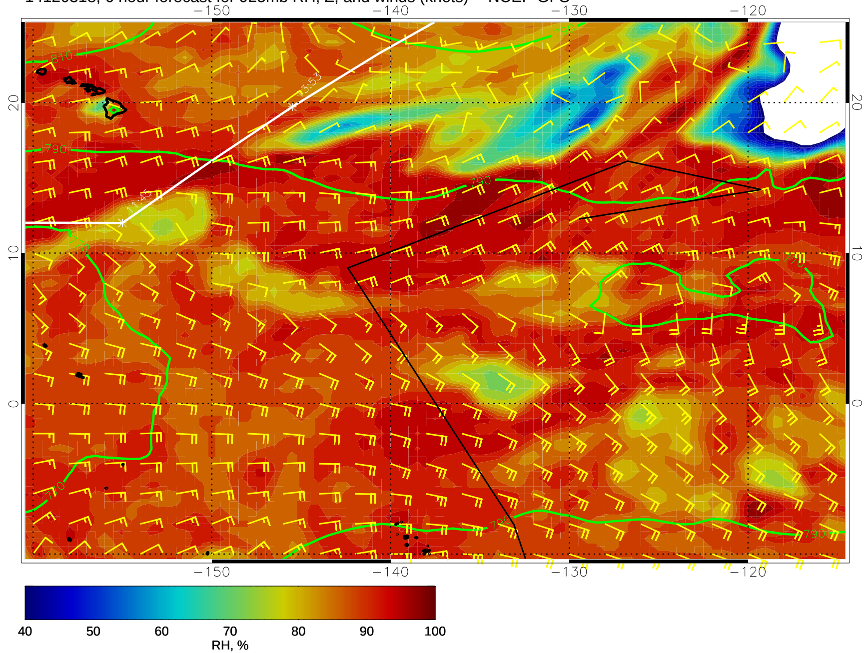
14120318, 6 hour forecast for 925mb RH, Z, and winds (knots) -- NCEP GFS
