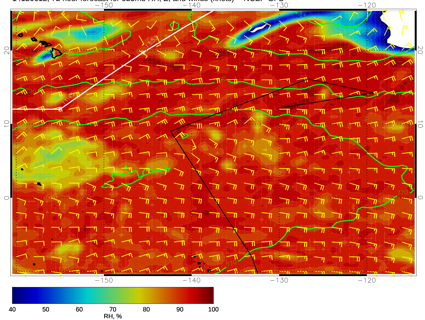
14120612, 72 hour forecast for 925mb RH, Z, and winds (knots) -- NCEP GFS
