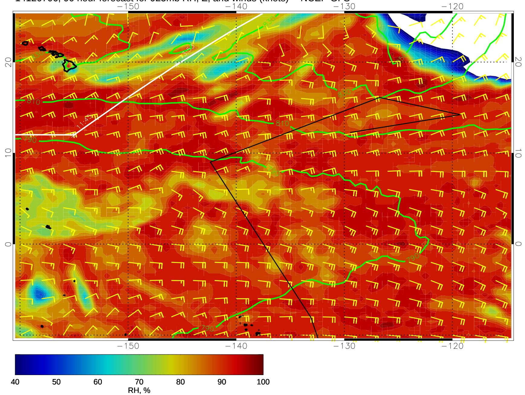
14120706, 90 hour forecast for 925mb RH, Z, and winds (knots) -- NCEP GFS
