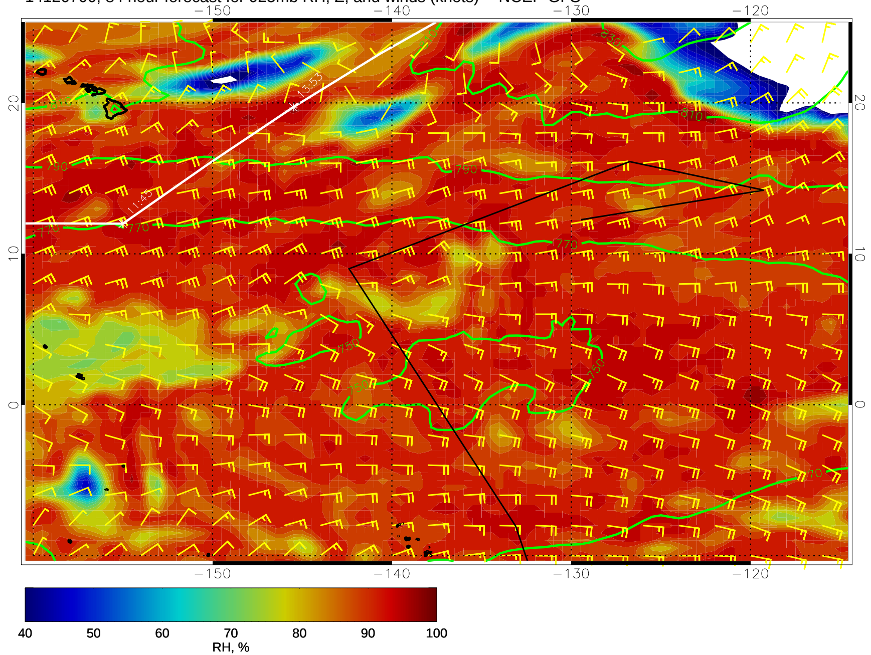
14120700, 84 hour forecast for 925mb RH, Z, and winds (knots) -- NCEP GFS
