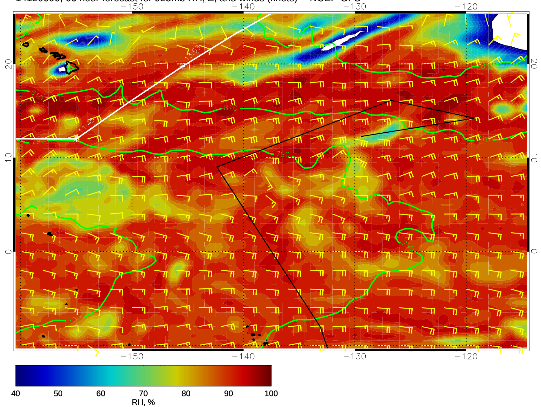
14120606, 66 hour forecast for 925mb RH, Z, and winds (knots) -- NCEP GFS
