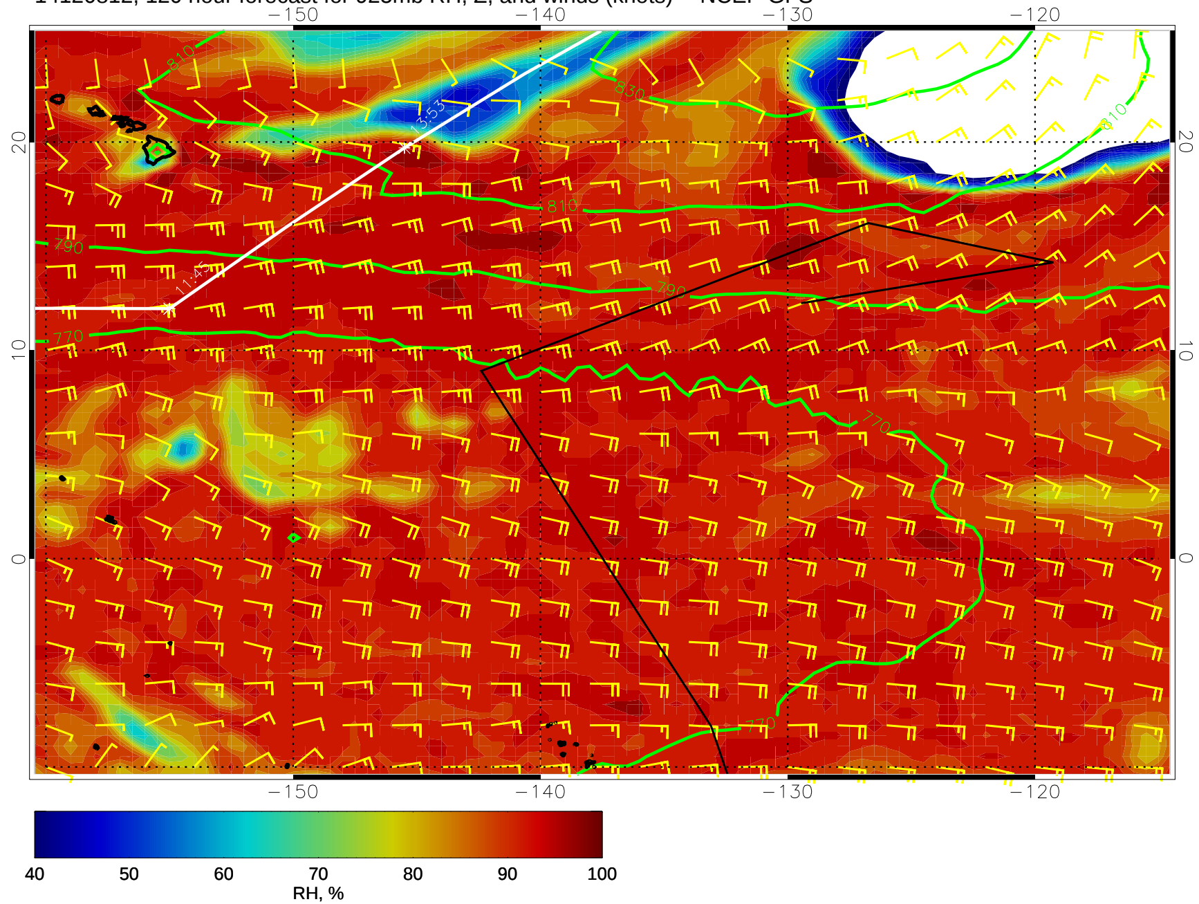
14120812, 120 hour forecast for 925mb RH, Z, and winds (knots) -- NCEP GFS
