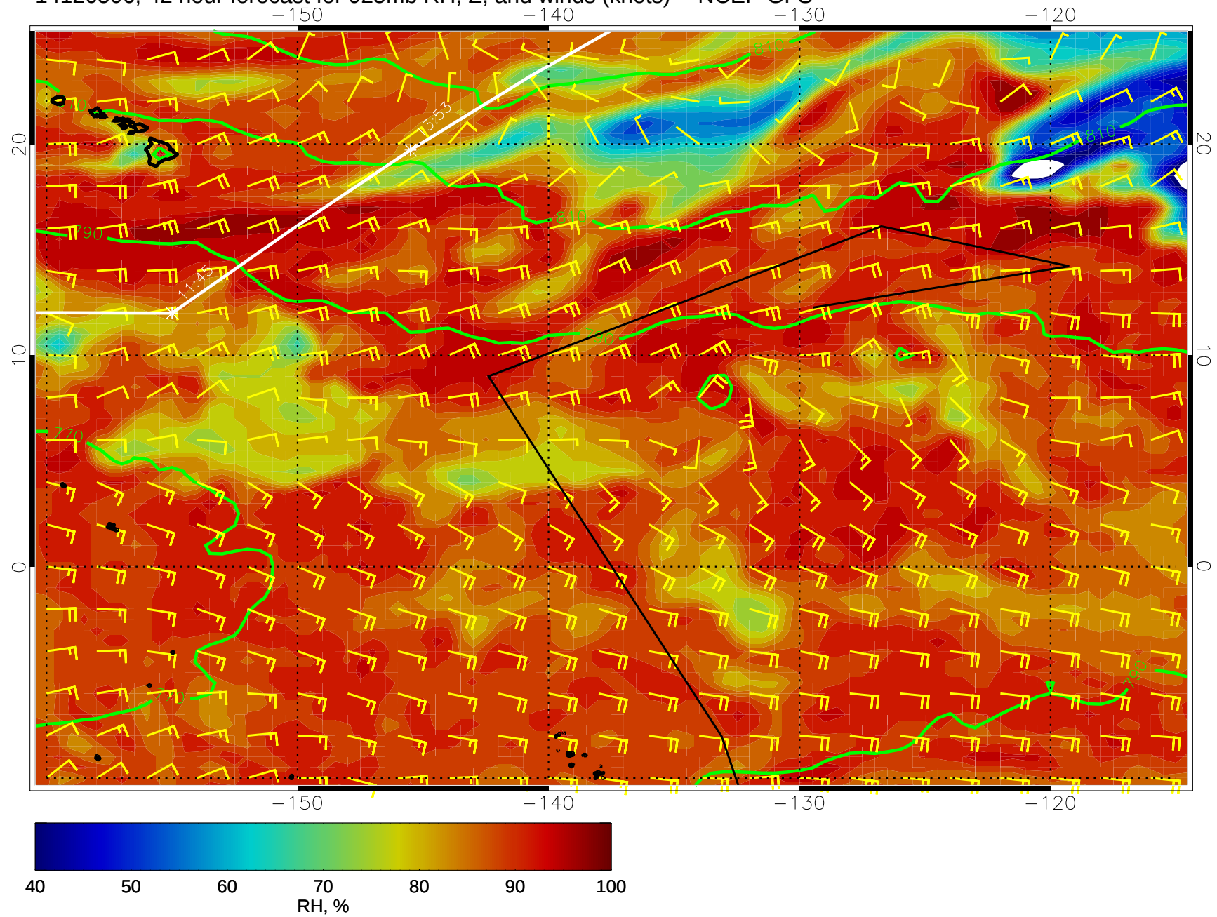
14120506, 42 hour forecast for 925mb RH, Z, and winds (knots) -- NCEP GFS
