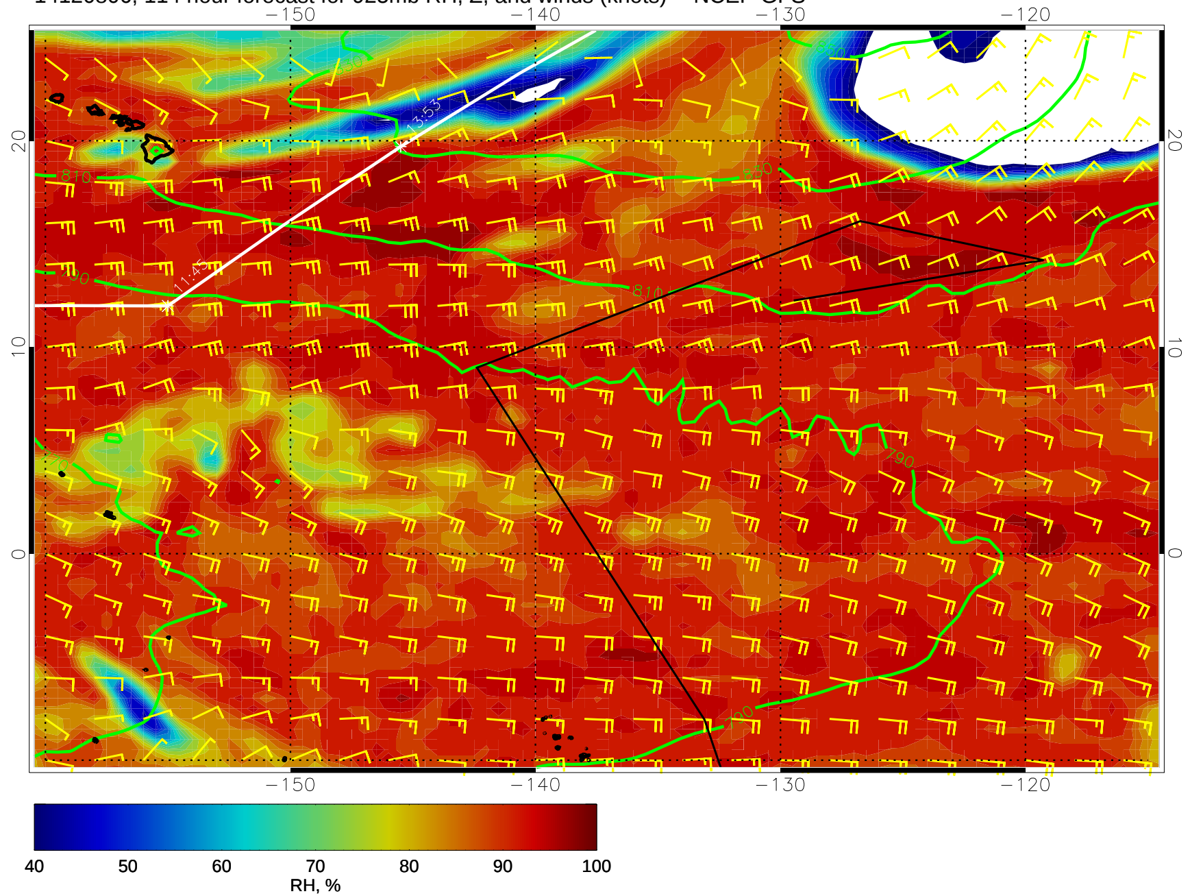
14120806, 114 hour forecast for 925mb RH, Z, and winds (knots) -- NCEP GFS
