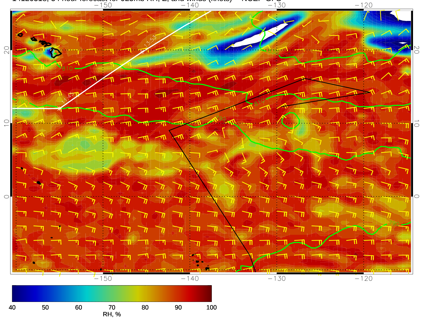
14120518, 54 hour forecast for 925mb RH, Z, and winds (knots) -- NCEP GFS
