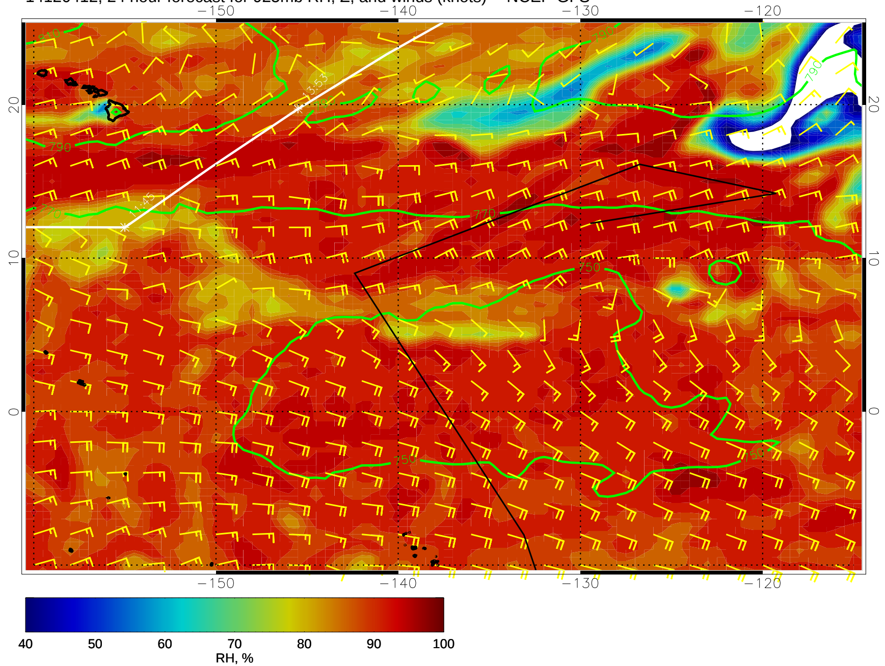
14120412, 24 hour forecast for 925mb RH, Z, and winds (knots) -- NCEP GFS
