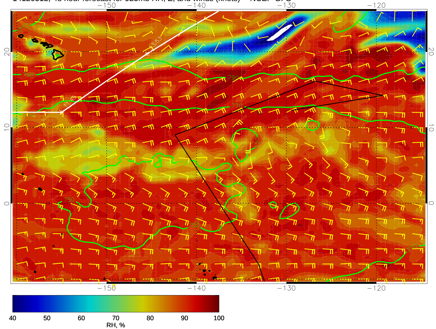
14120512, 48 hour forecast for 925mb RH, Z, and winds (knots) -- NCEP GFS
