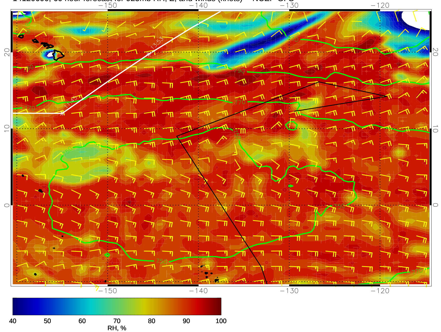
14120600, 60 hour forecast for 925mb RH, Z, and winds (knots) -- NCEP GFS
