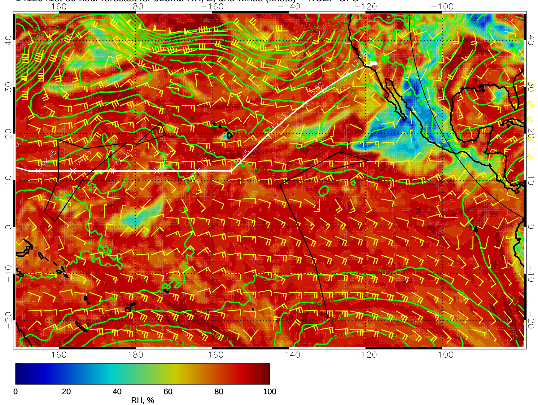
14120418, 30 hour forecast for 925mb RH, Z, and winds (knots) -- NCEP GFS
