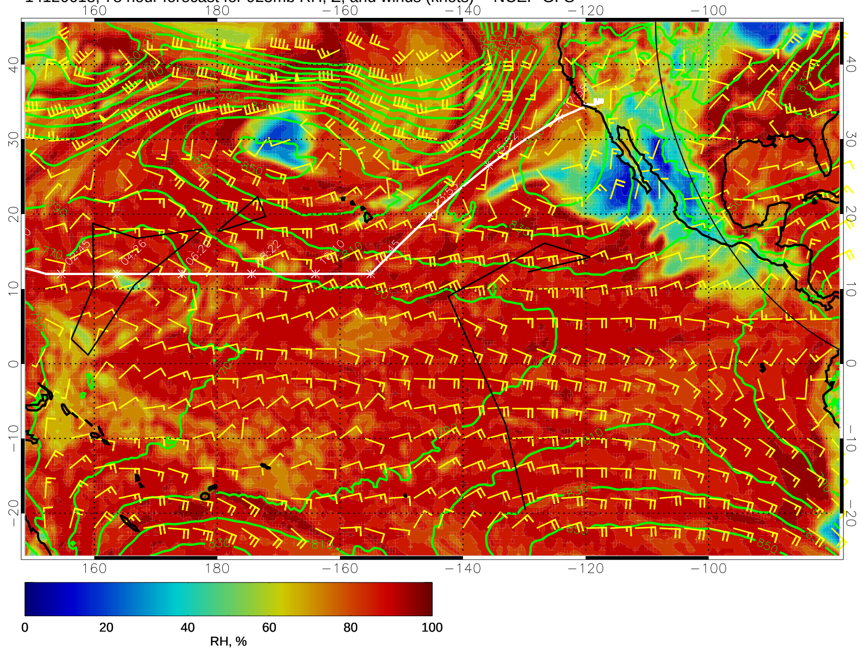
14120618, 78 hour forecast for 925mb RH, Z, and winds (knots) -- NCEP GFS
