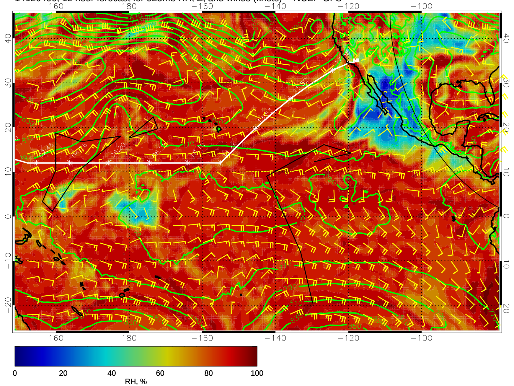
14120400, 12 hour forecast for 925mb RH, Z, and winds (knots) -- NCEP GFS
