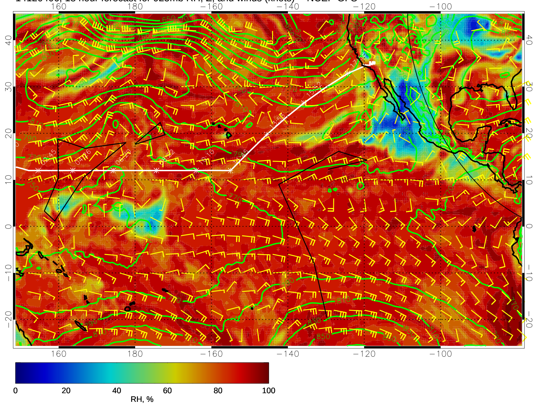
14120406, 18 hour forecast for 925mb RH, Z, and winds (knots) -- NCEP GFS
