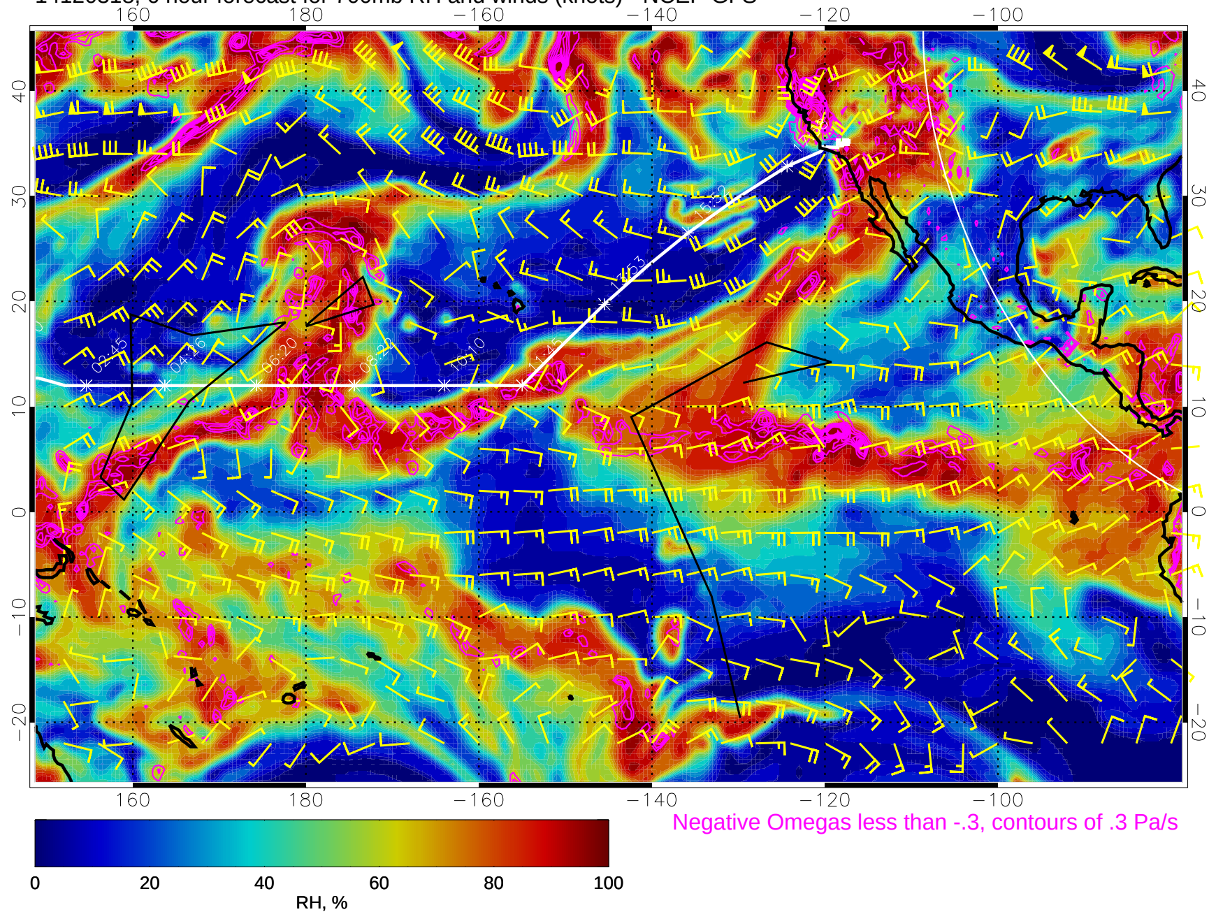
14120318, 6 hour forecast for 700mb RH and winds (knots) - NCEP GFS
