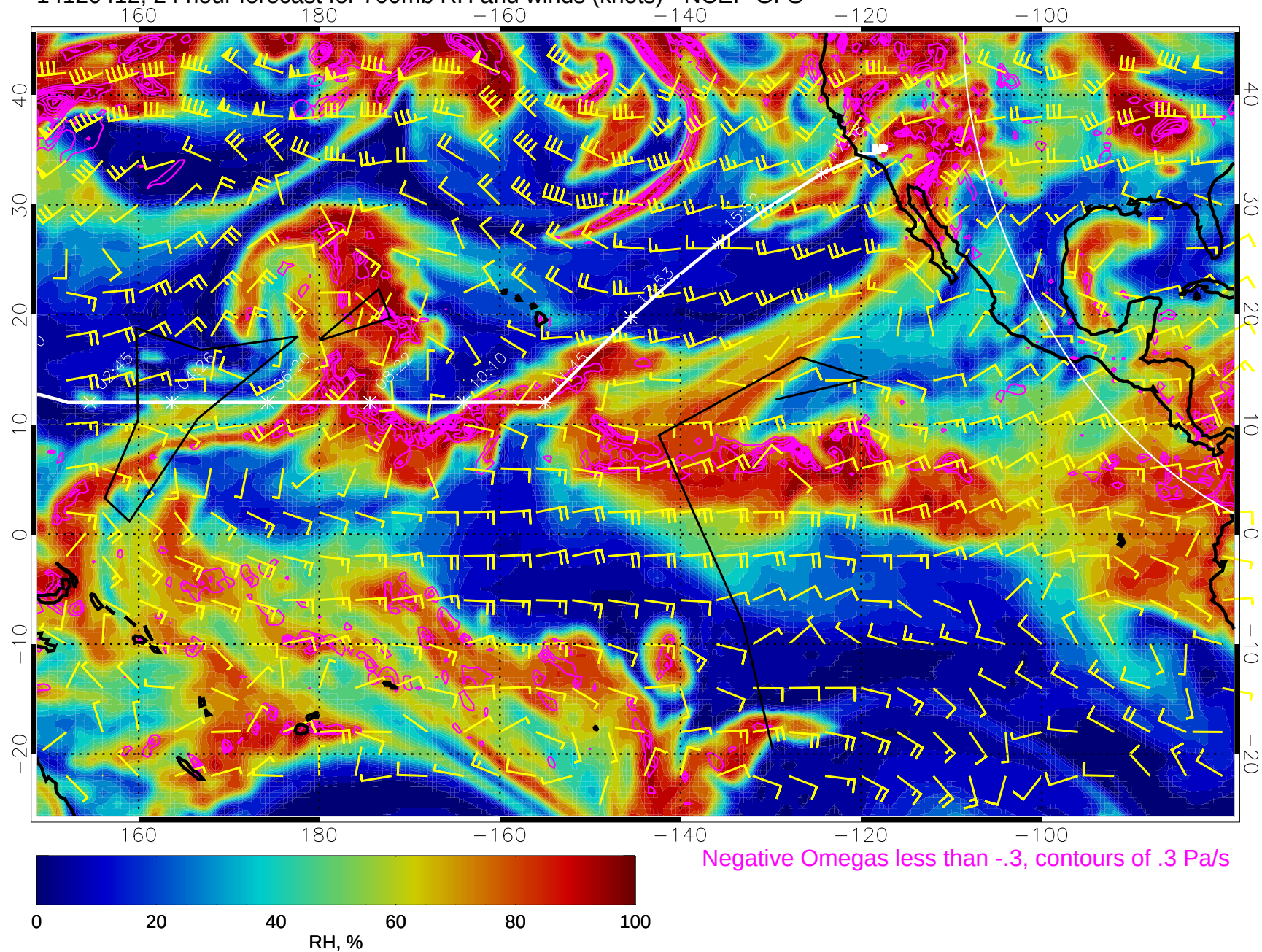
14120412, 24 hour forecast for 700mb RH and winds (knots) - NCEP GFS
