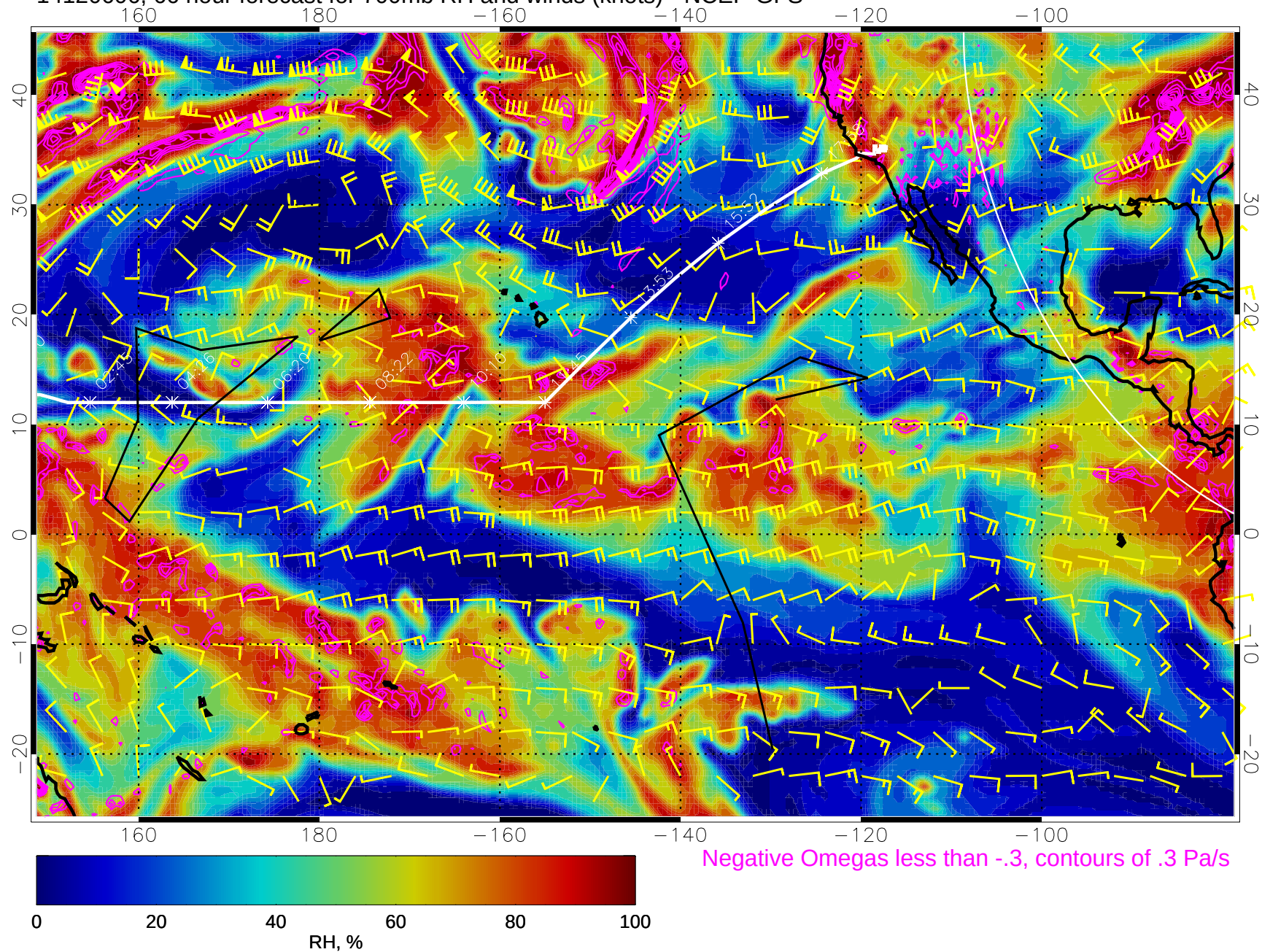
14120606, 66 hour forecast for 700mb RH and winds (knots) - NCEP GFS
