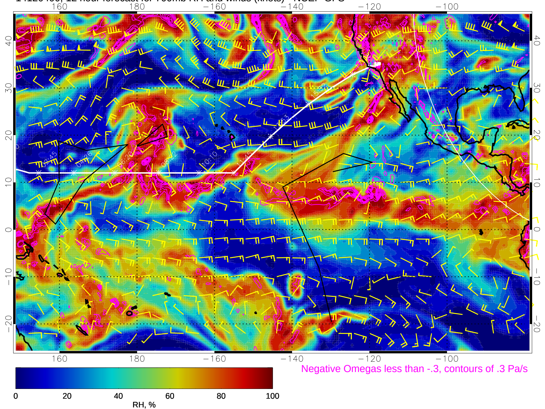
14120400, 12 hour forecast for 700mb RH and winds (knots) - NCEP GFS
