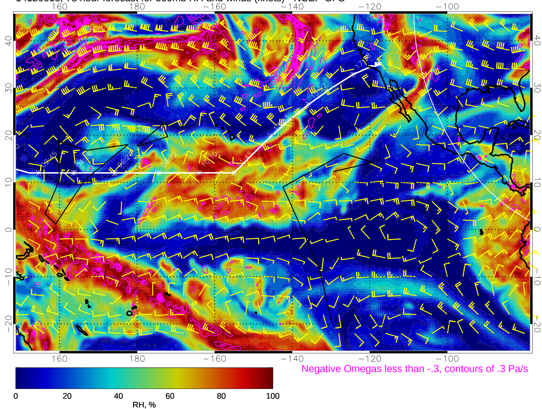
14120618, 78 hour forecast for 500mb RH and winds (knots) - NCEP GFS
