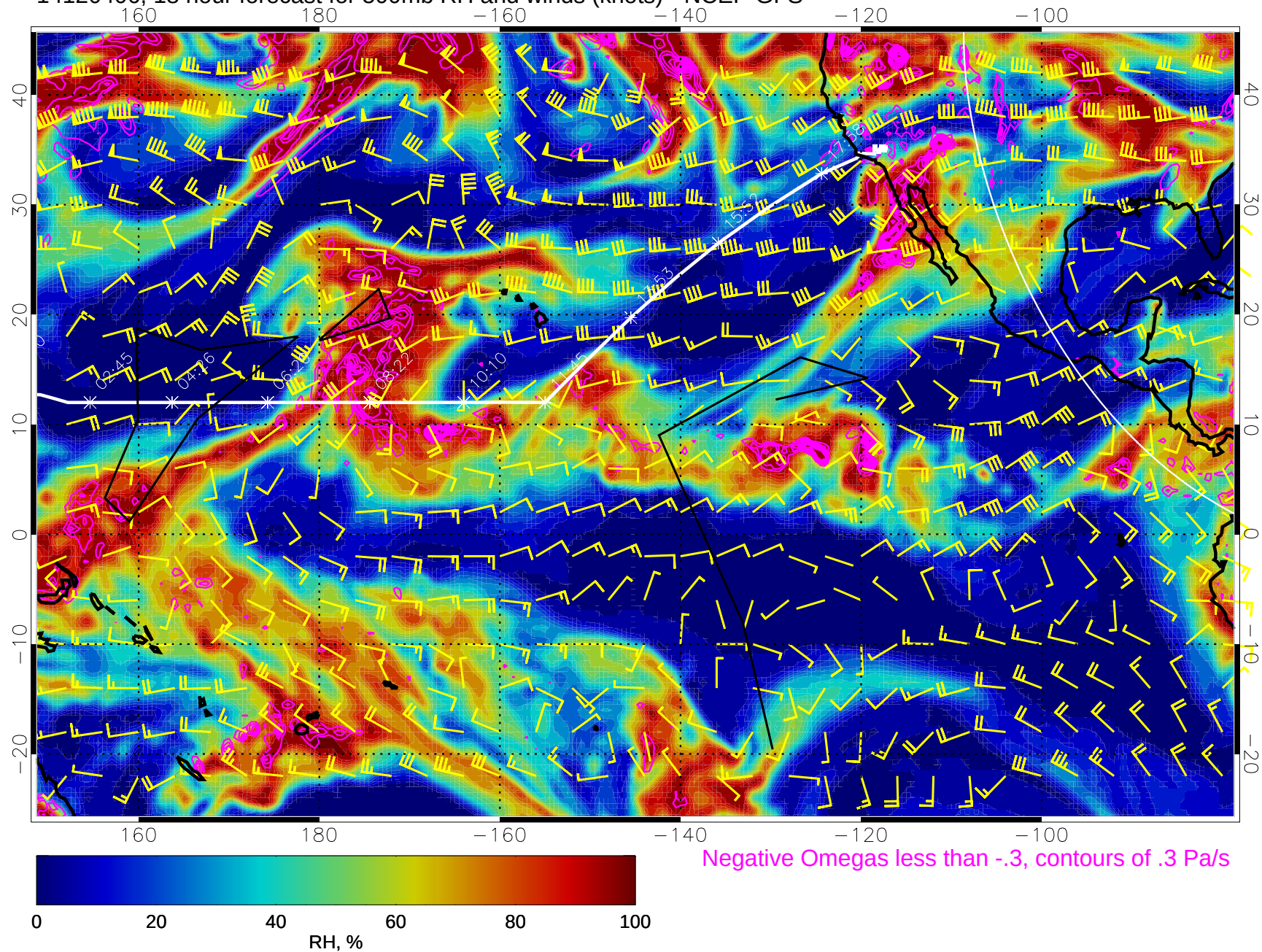
14120406, 18 hour forecast for 500mb RH and winds (knots) - NCEP GFS
