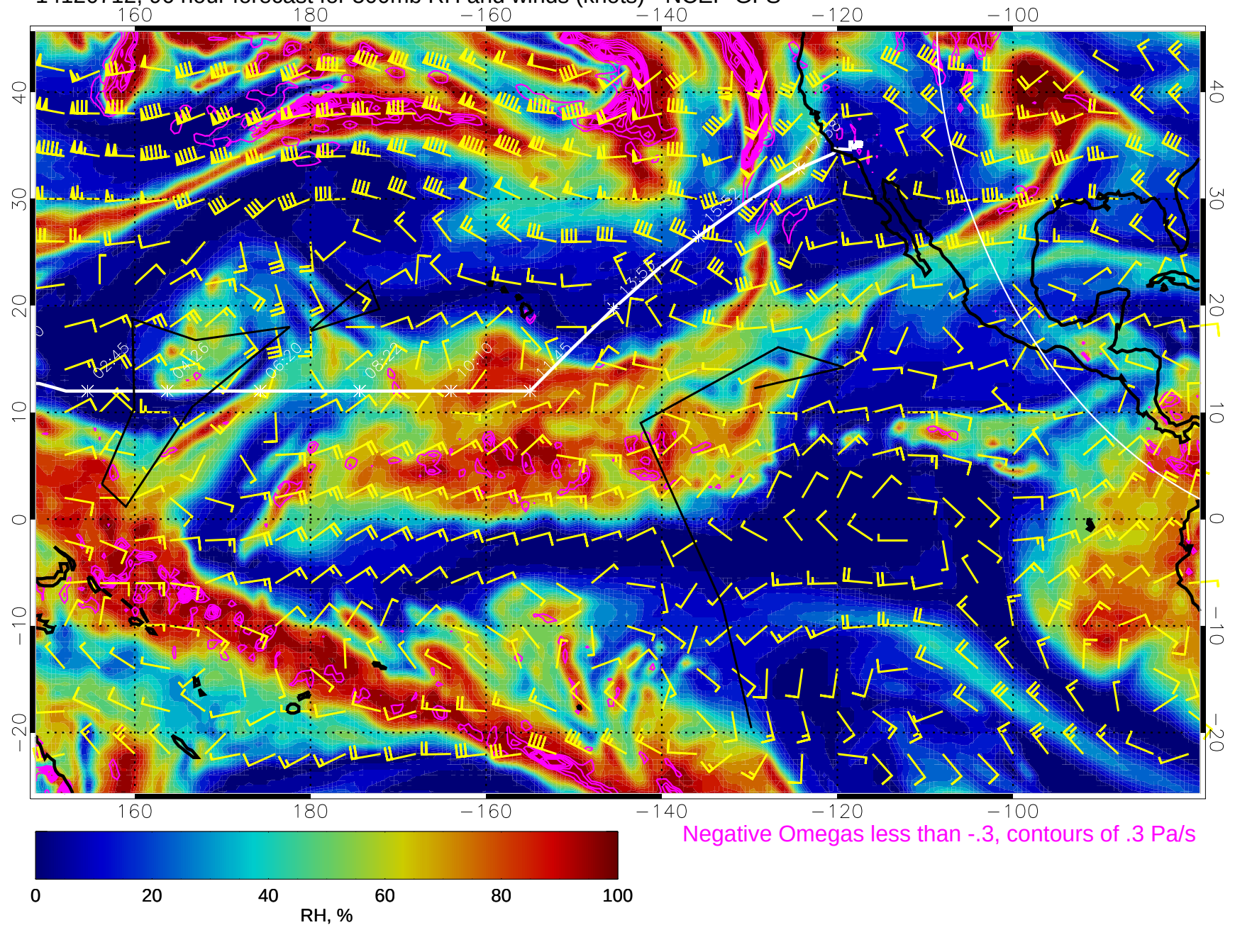
14120712, 96 hour forecast for 500mb RH and winds (knots) - NCEP GFS
