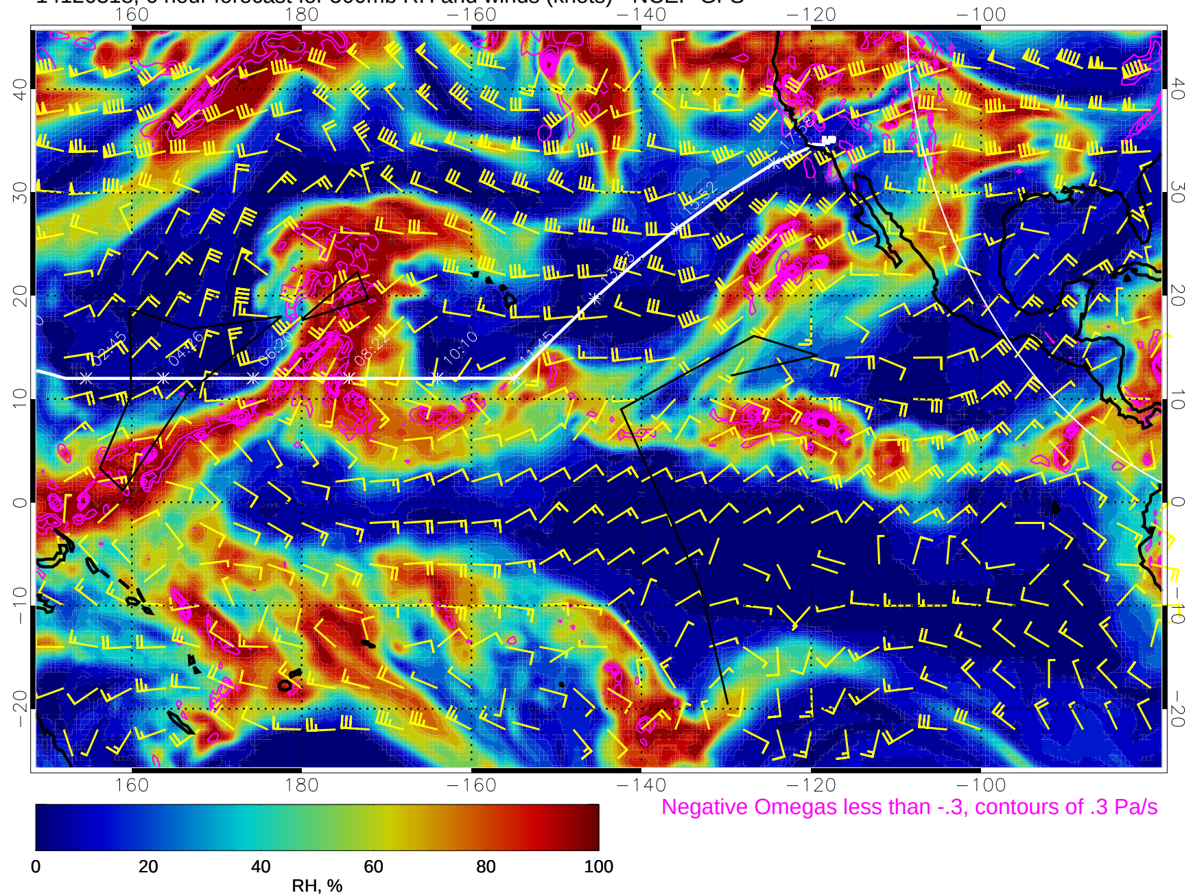
14120318, 6 hour forecast for 500mb RH and winds (knots) - NCEP GFS
