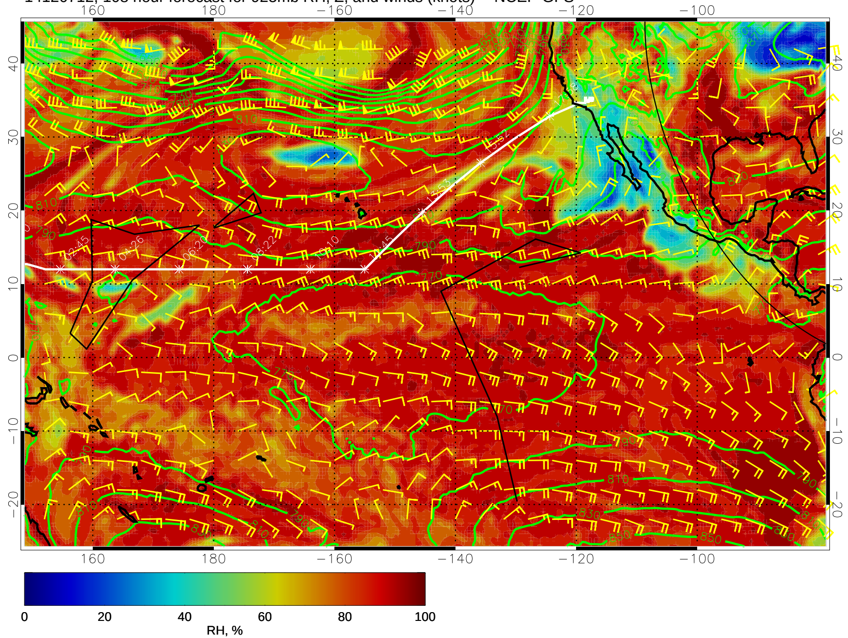
14120712, 108 hour forecast for 925mb RH, Z, and winds (knots) -- NCEP GFS
