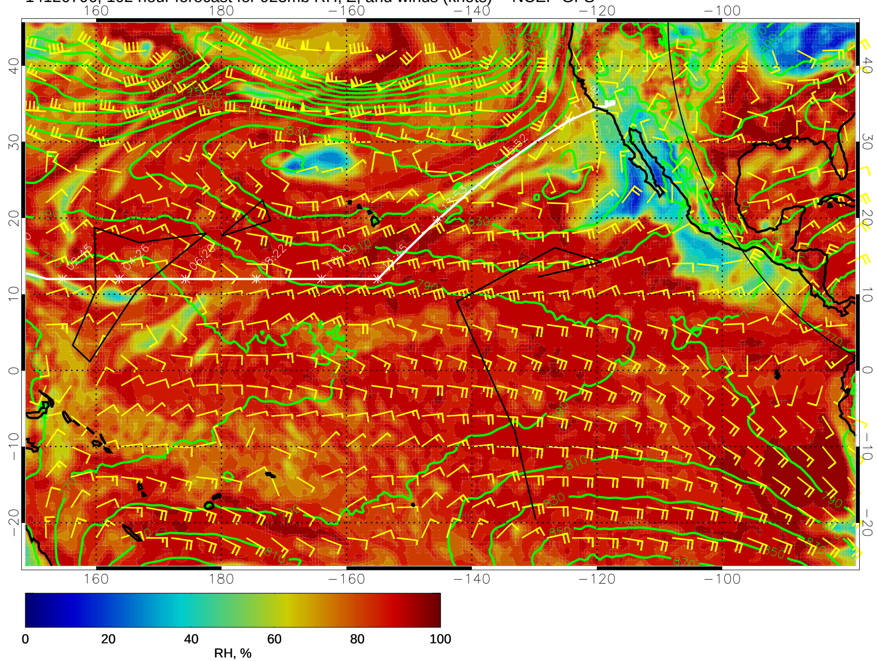
14120706, 102 hour forecast for 925mb RH, Z, and winds (knots) -- NCEP GFS
