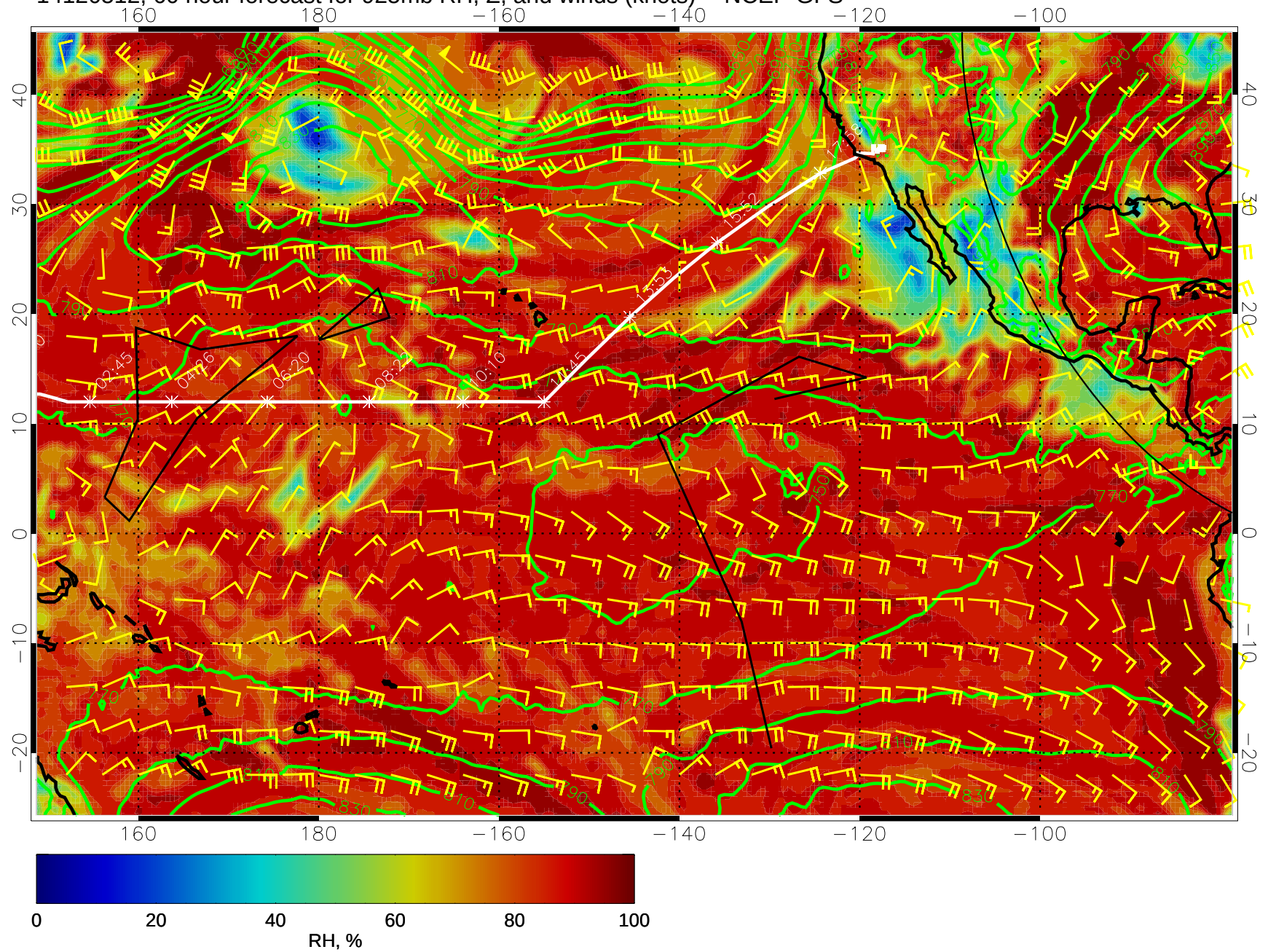
14120512, 60 hour forecast for 925mb RH, Z, and winds (knots) -- NCEP GFS
