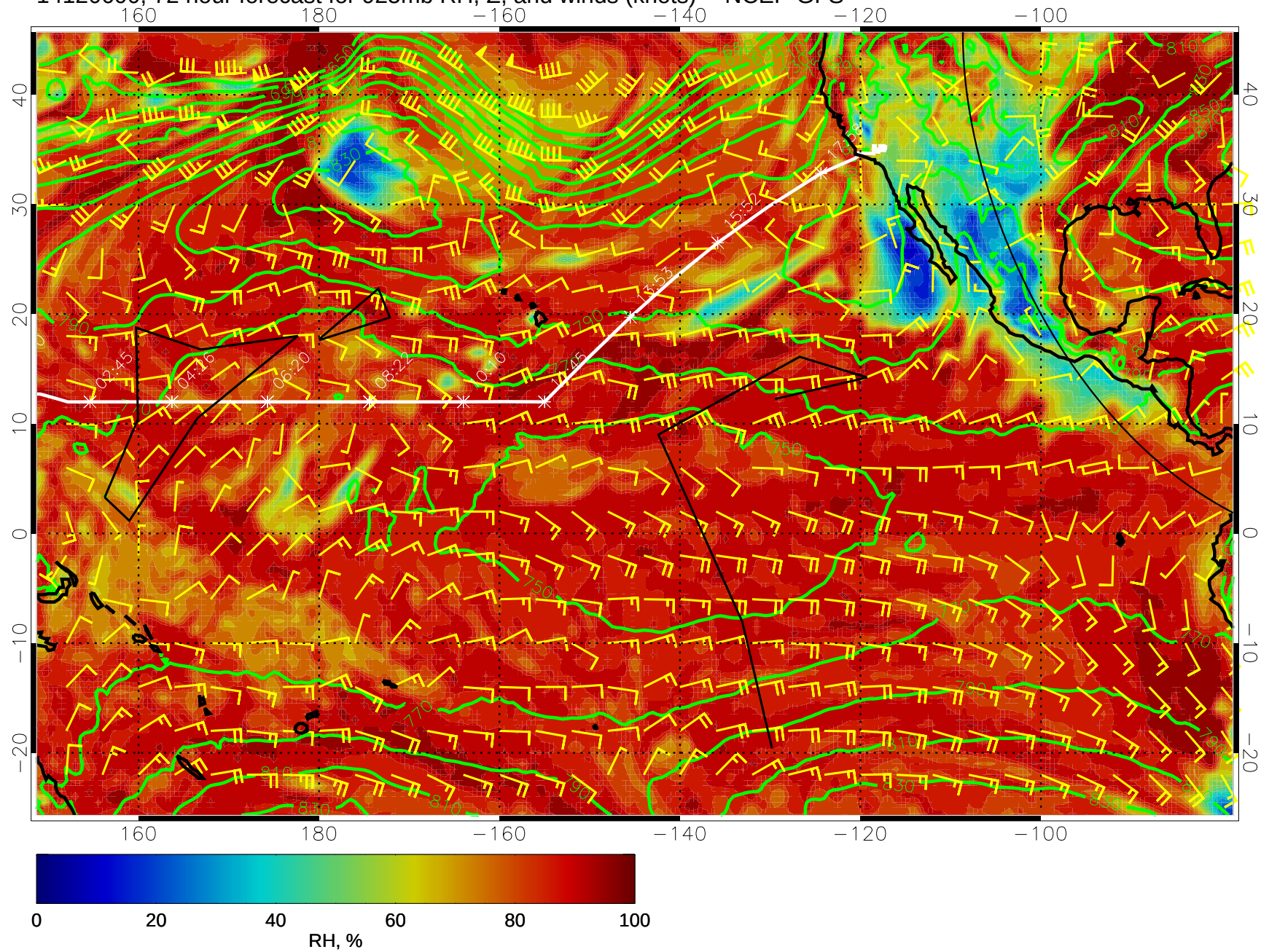
14120600, 72 hour forecast for 925mb RH, Z, and winds (knots) -- NCEP GFS
