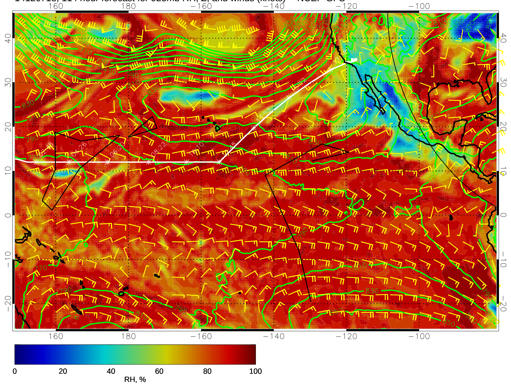
14120718, 114 hour forecast for 925mb RH, Z, and winds (knots) -- NCEP GFS
