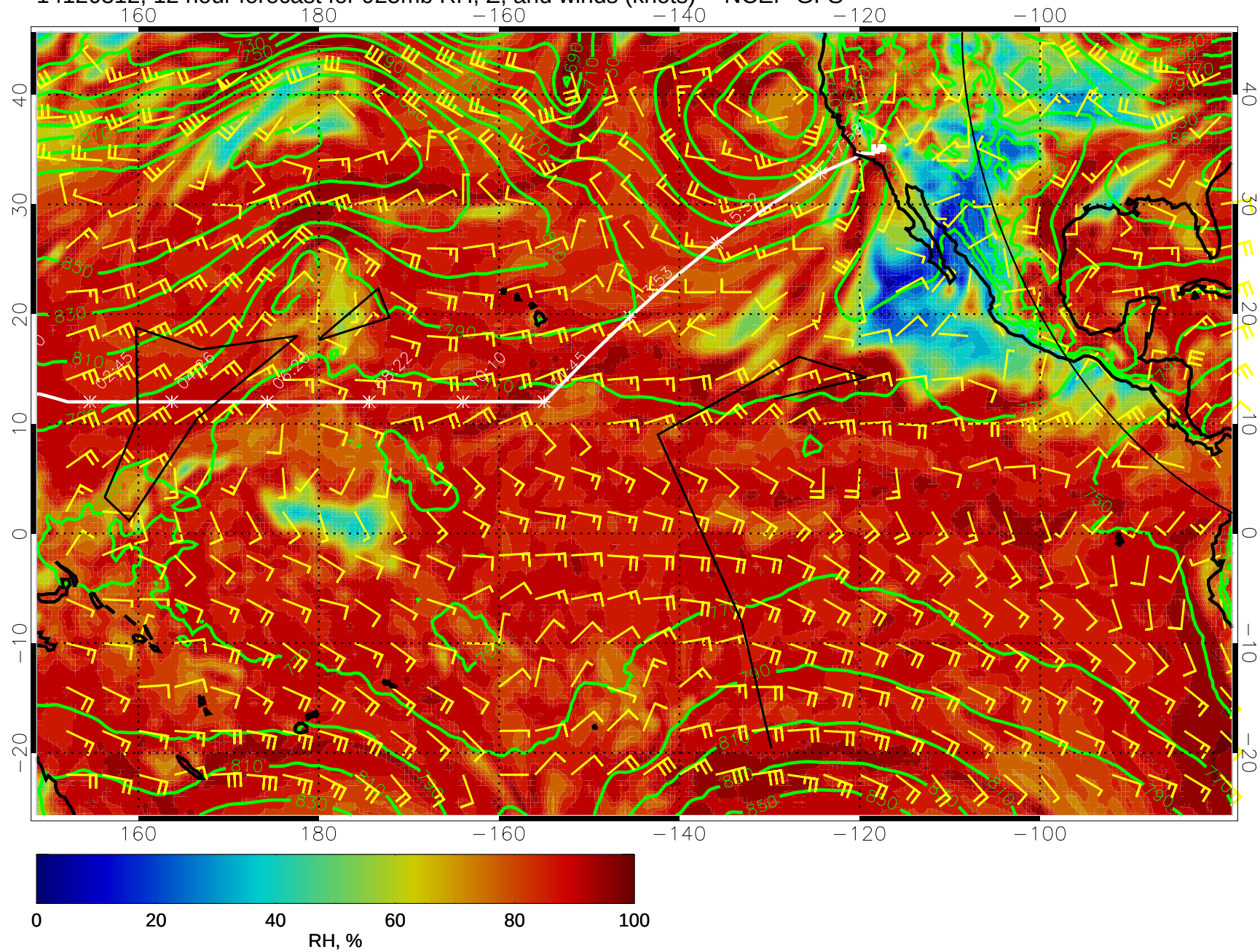
14120312, 12 hour forecast for 925mb RH, Z, and winds (knots) -- NCEP GFS
