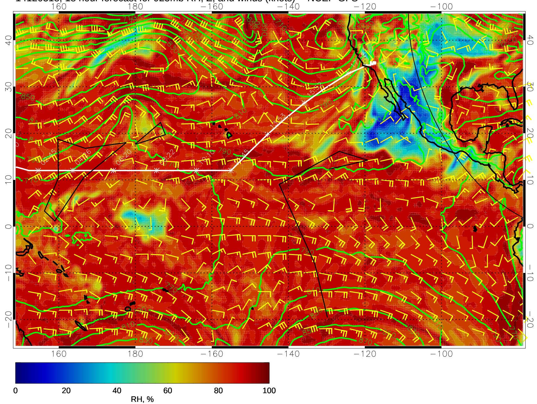
14120318, 18 hour forecast for 925mb RH, Z, and winds (knots) -- NCEP GFS
