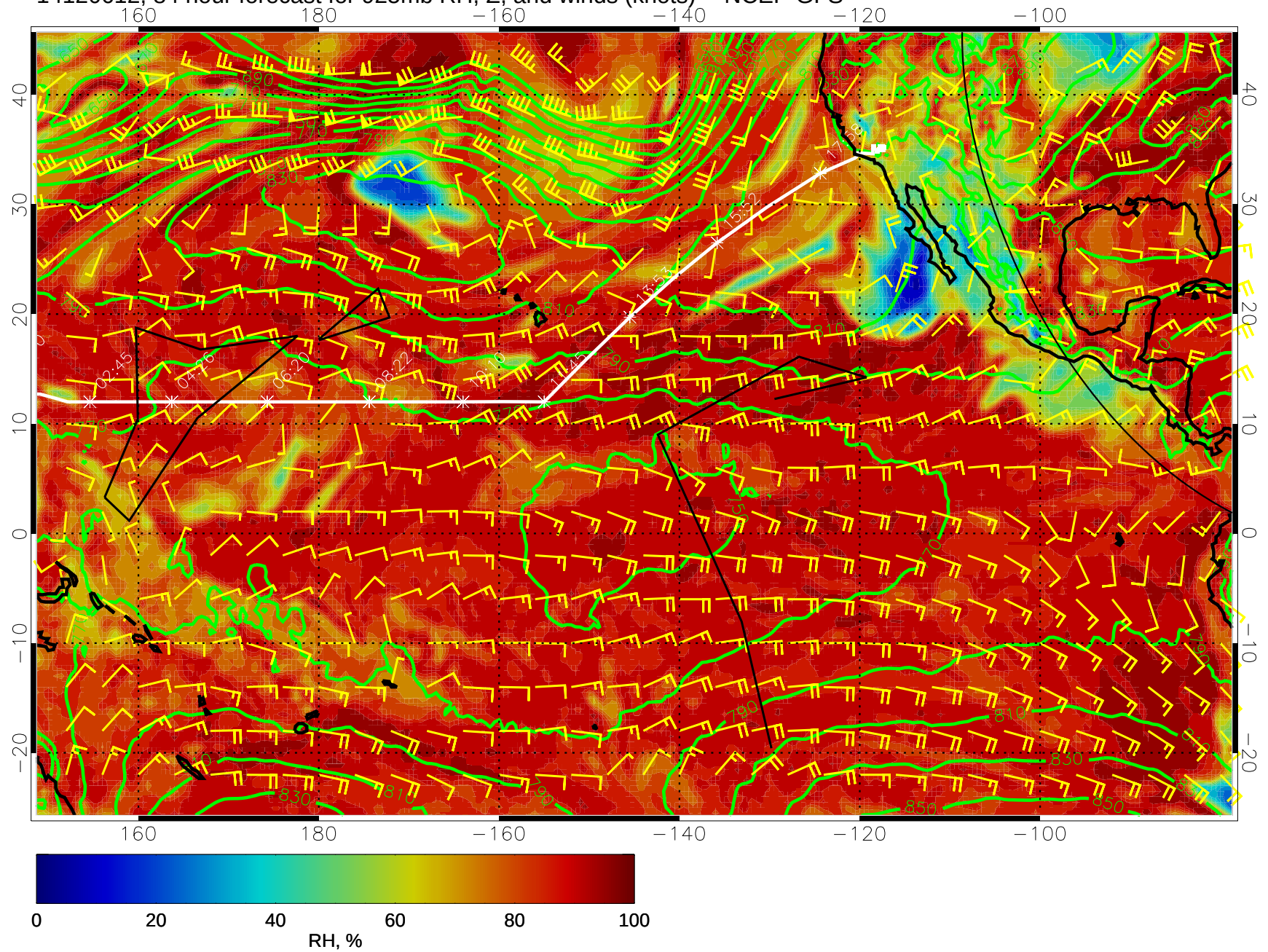
14120612, 84 hour forecast for 925mb RH, Z, and winds (knots) -- NCEP GFS
