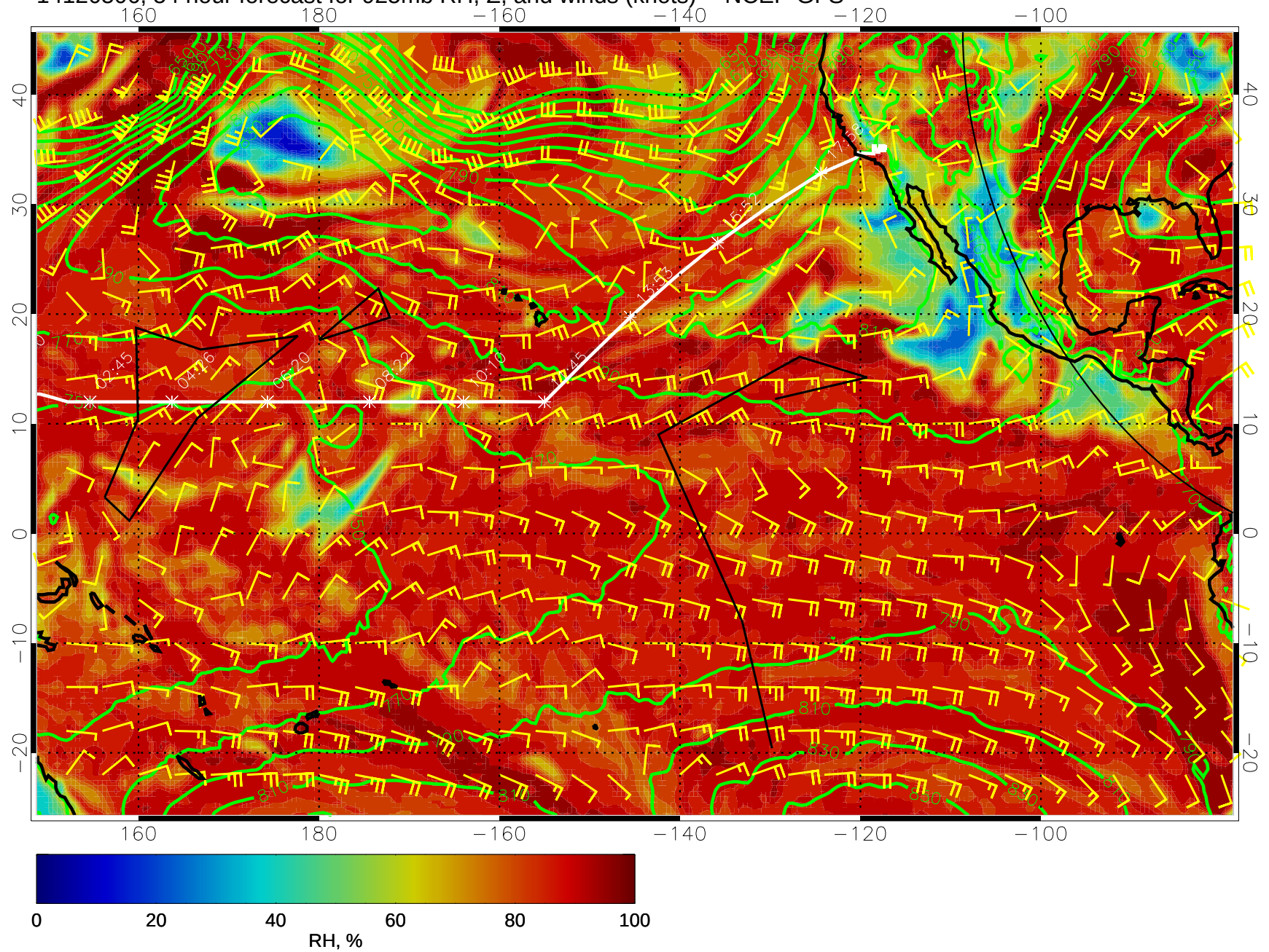
14120506, 54 hour forecast for 925mb RH, Z, and winds (knots) -- NCEP GFS
