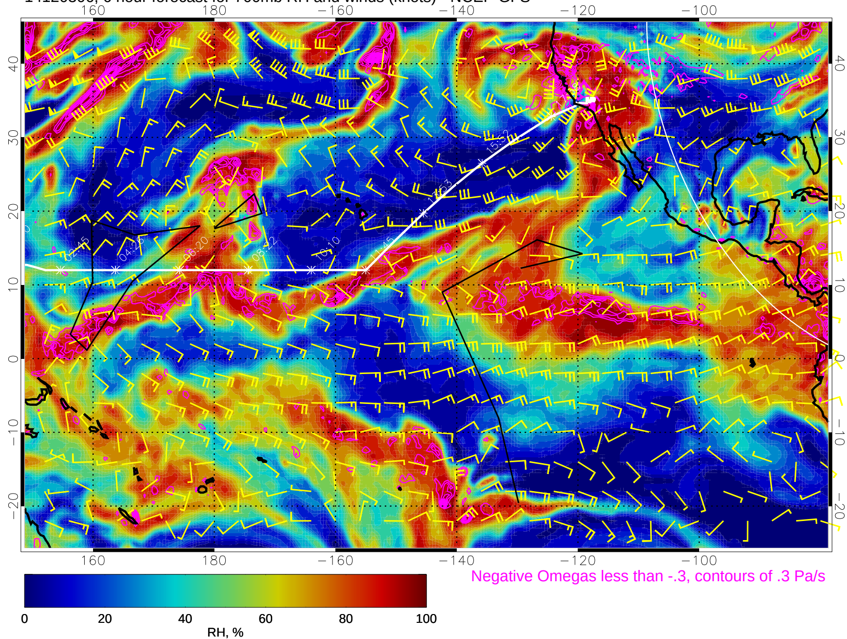
14120306, 6 hour forecast for 700mb RH and winds (knots) - NCEP GFS
