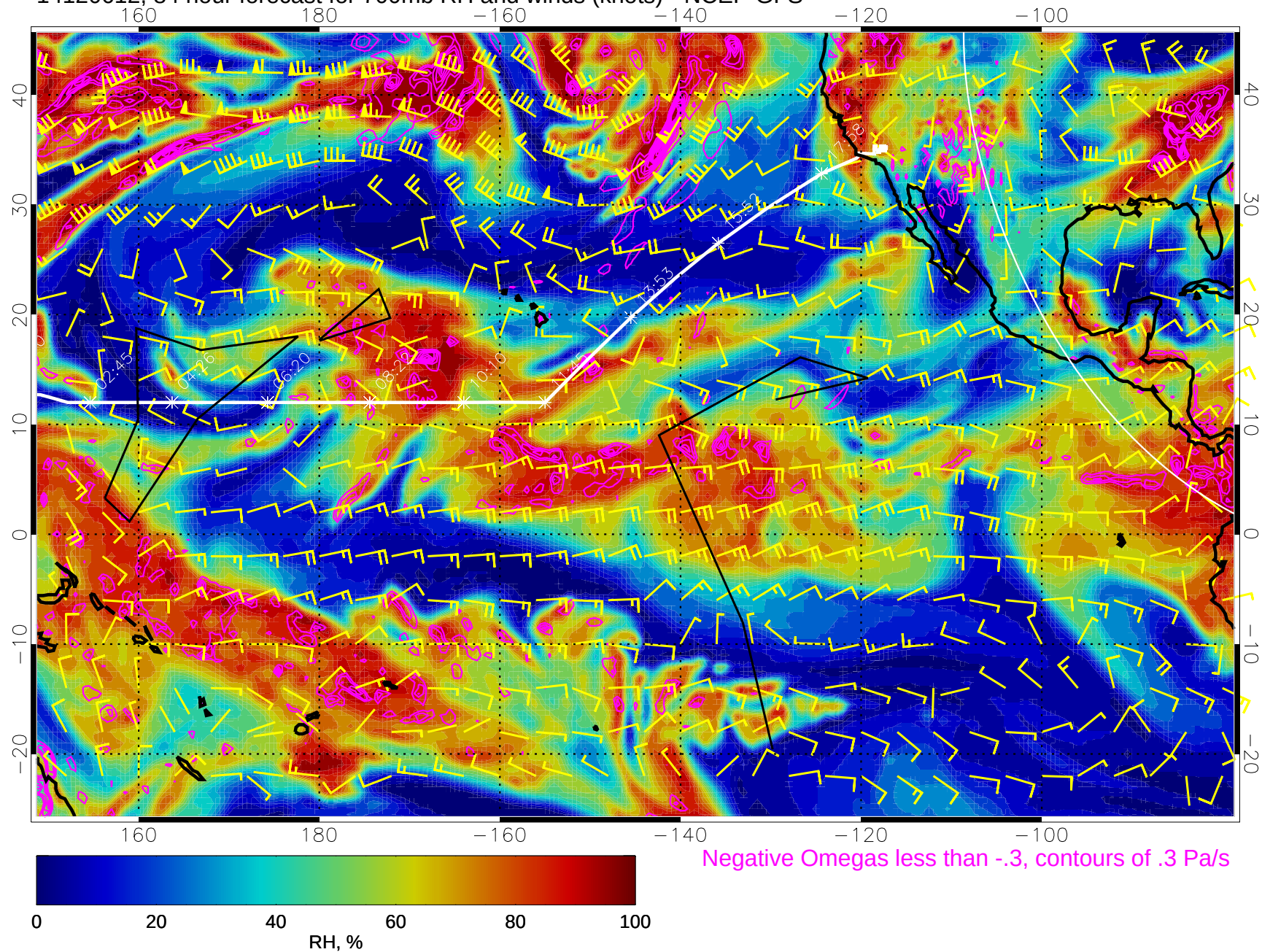
14120612, 84 hour forecast for 700mb RH and winds (knots) - NCEP GFS
