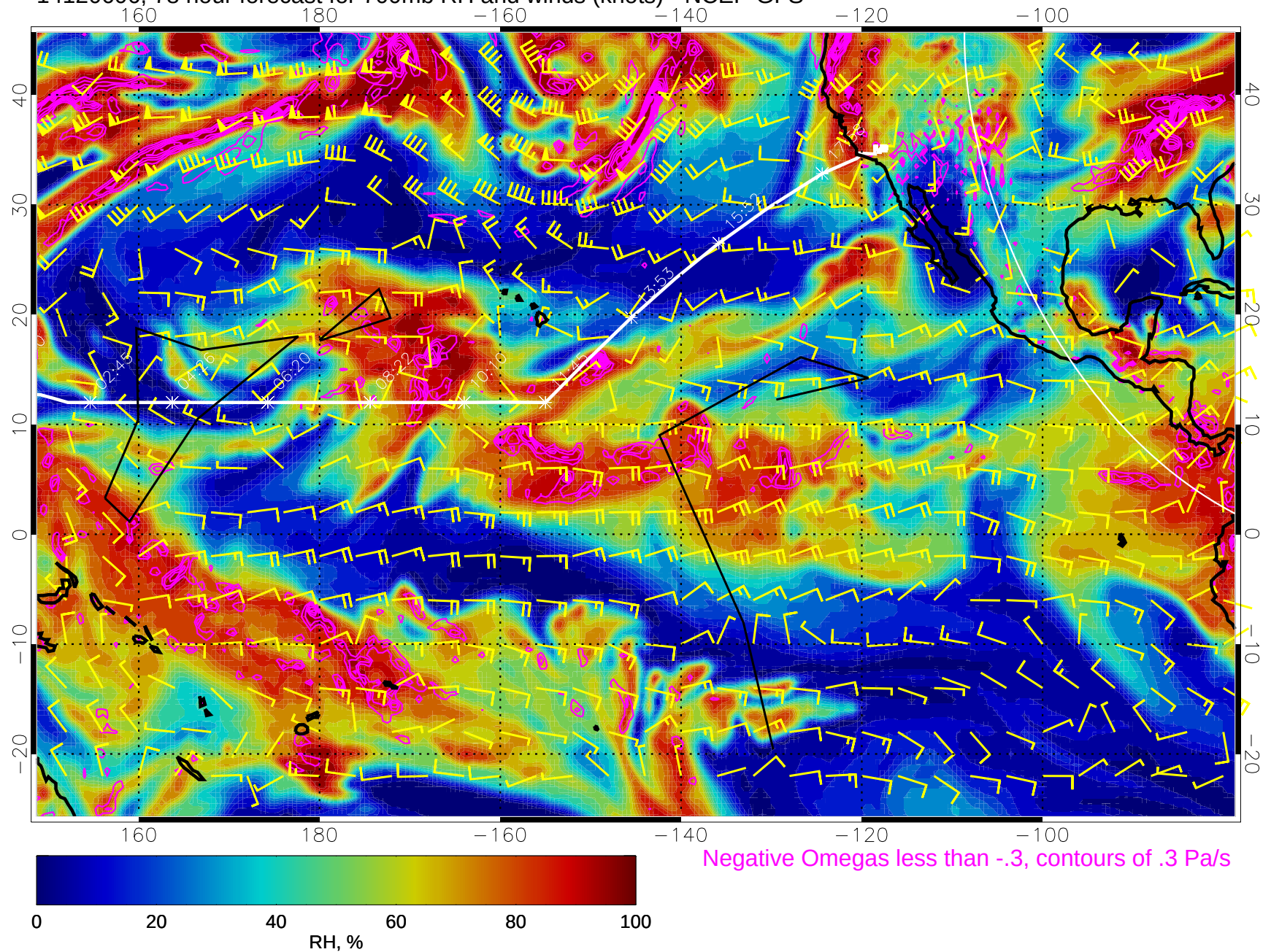
14120606, 78 hour forecast for 700mb RH and winds (knots) - NCEP GFS
