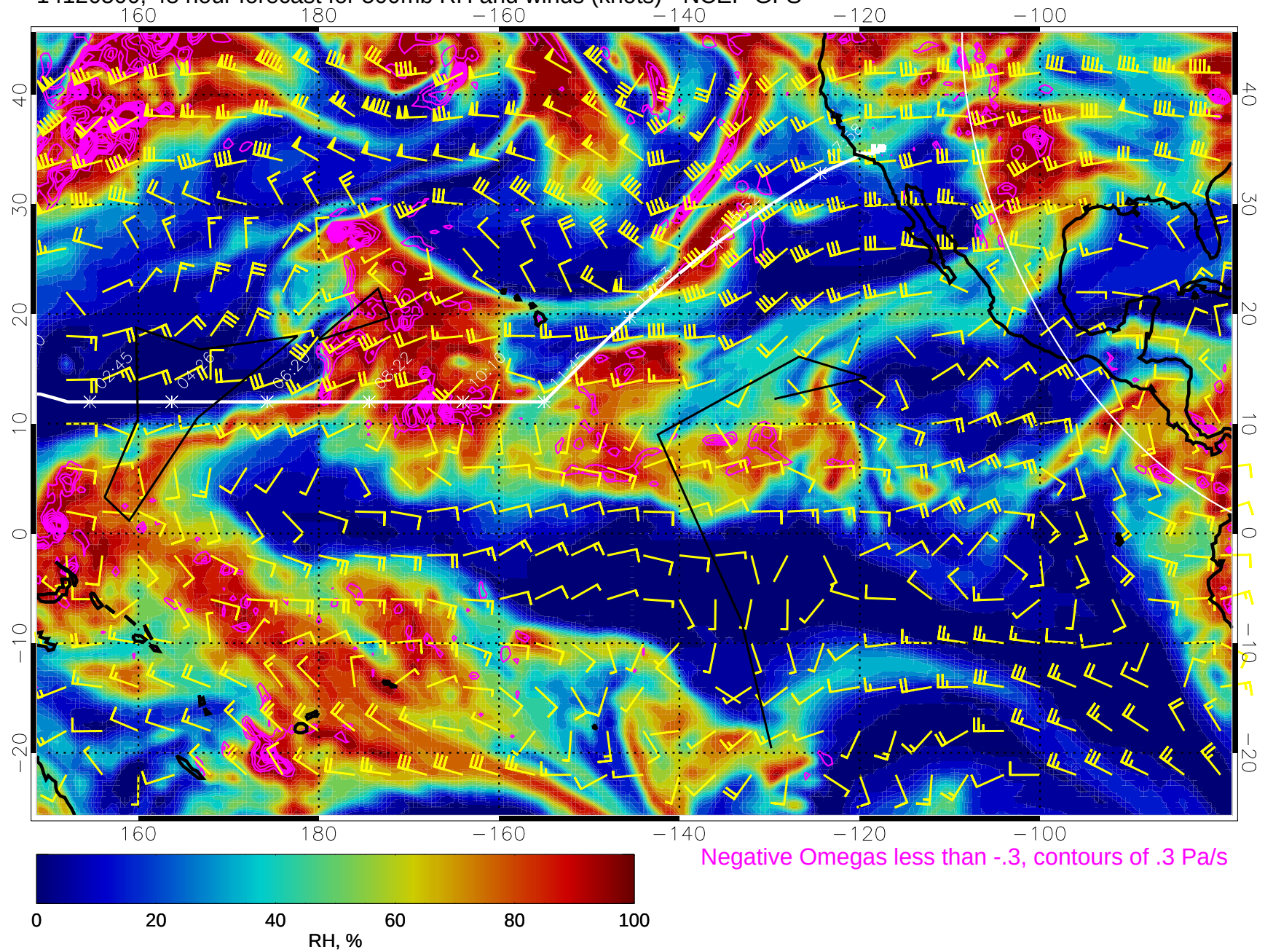
14120500, 48 hour forecast for 500mb RH and winds (knots) - NCEP GFS
