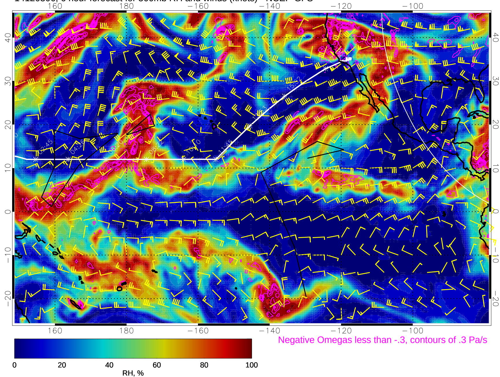
14120306, 6 hour forecast for 500mb RH and winds (knots) - NCEP GFS
