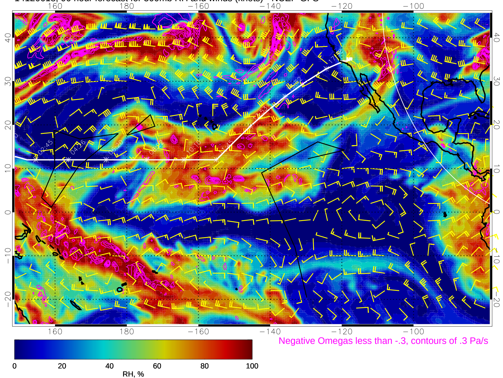
14120618, 90 hour forecast for 500mb RH and winds (knots) - NCEP GFS
