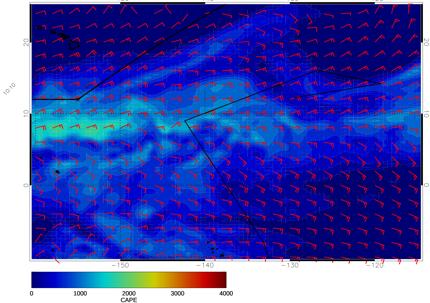
14120712, 108 hour forecast for CAPE and surface winds (knots) -- NCEP GFS
