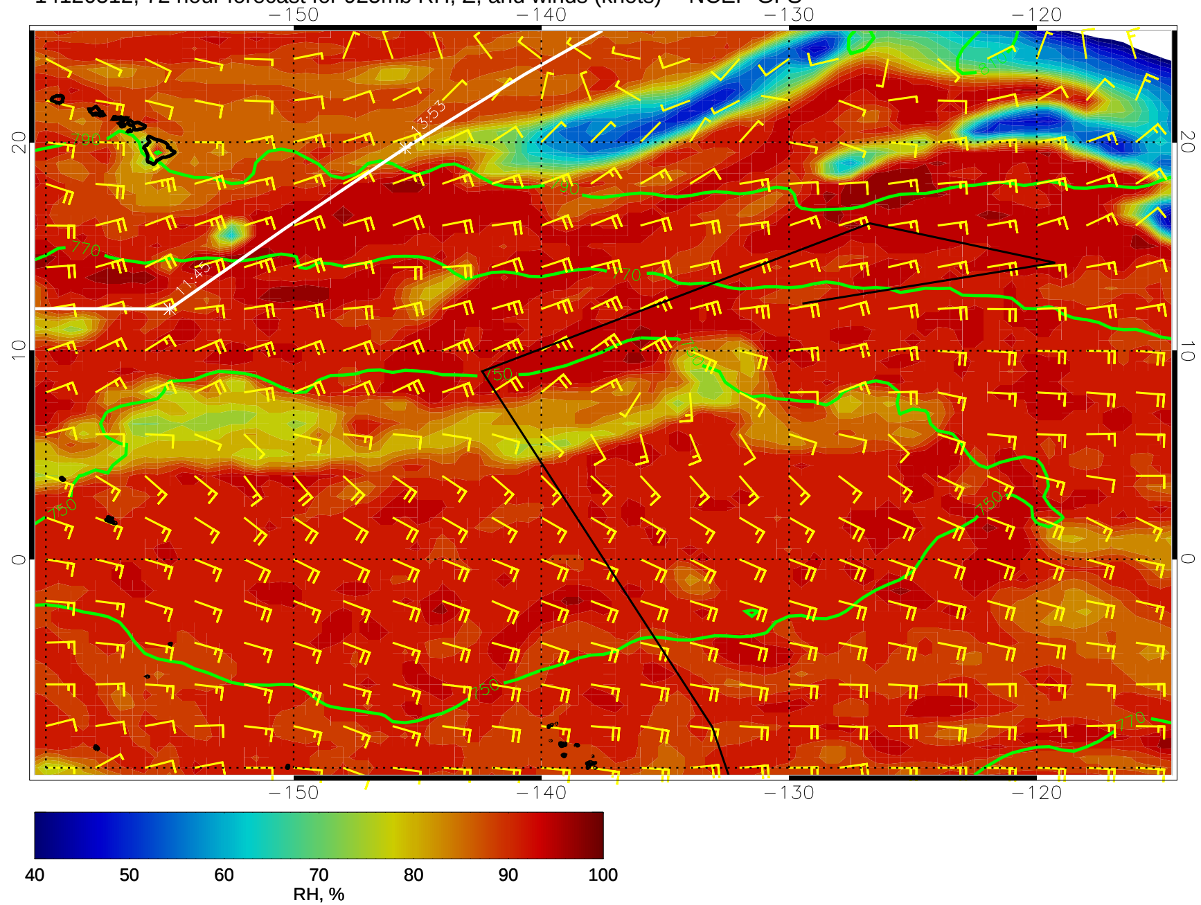
14120512, 72 hour forecast for 925mb RH, Z, and winds (knots) -- NCEP GFS
