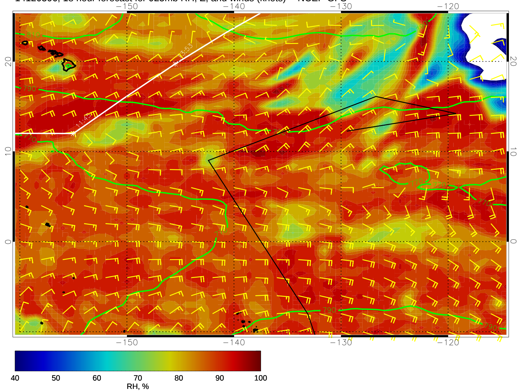
14120306, 18 hour forecast for 925mb RH, Z, and winds (knots) -- NCEP GFS
