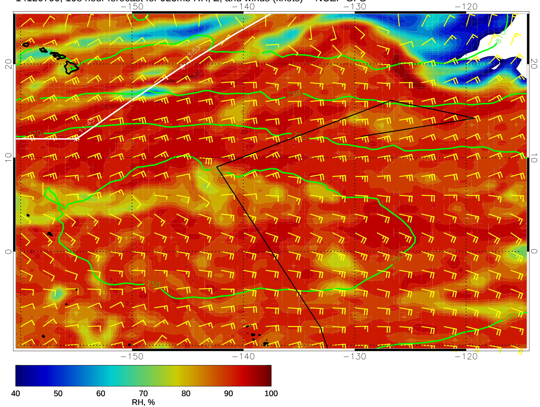
14120700, 108 hour forecast for 925mb RH, Z, and winds (knots) -- NCEP GFS
