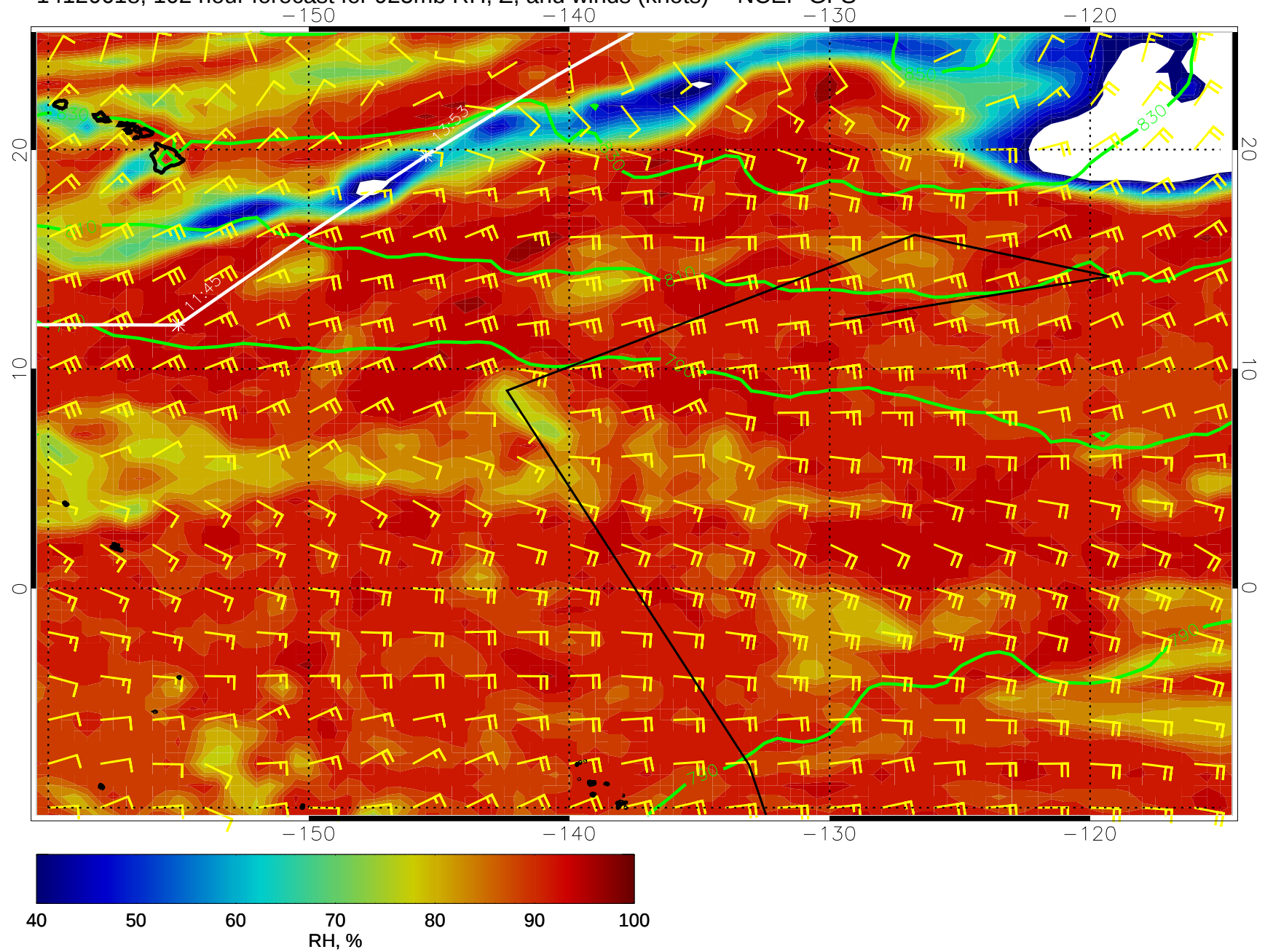
14120618, 102 hour forecast for 925mb RH, Z, and winds (knots) -- NCEP GFS
