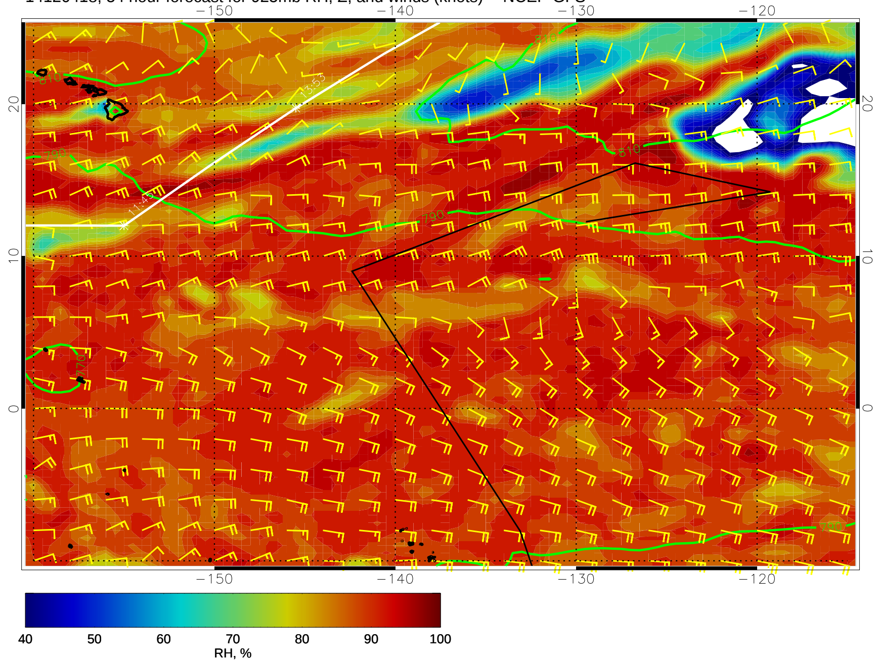
14120418, 54 hour forecast for 925mb RH, Z, and winds (knots) -- NCEP GFS
