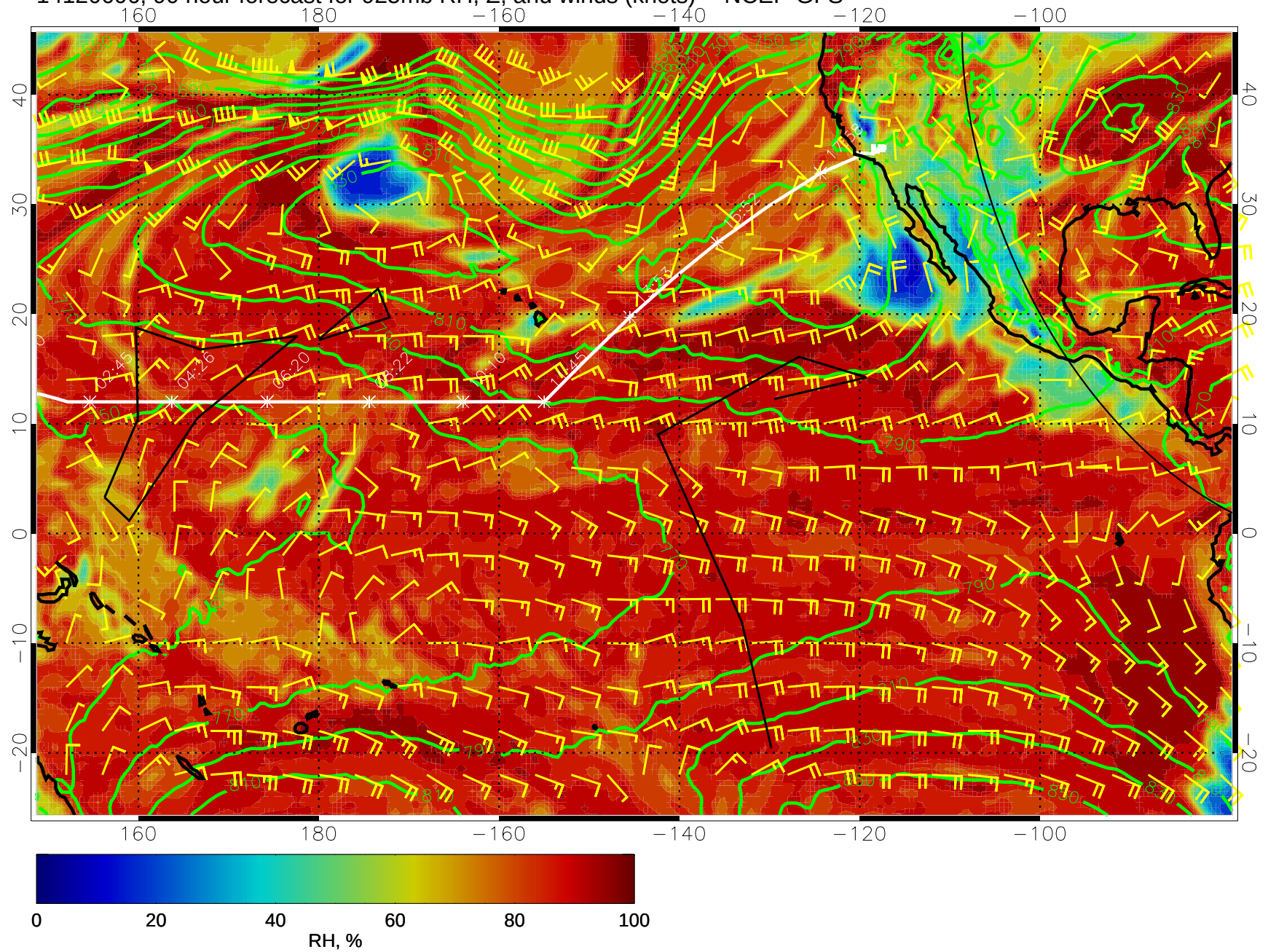
14120606, 90 hour forecast for 925mb RH, Z, and winds (knots) -- NCEP GFS
