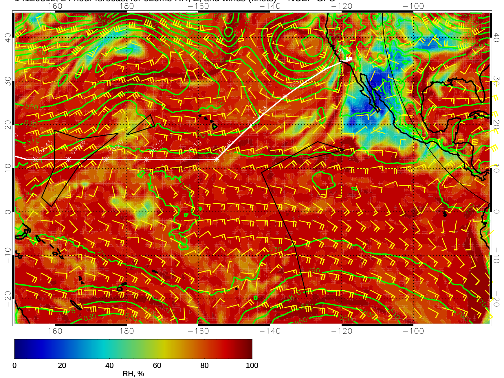
14120312, 24 hour forecast for 925mb RH, Z, and winds (knots) -- NCEP GFS
