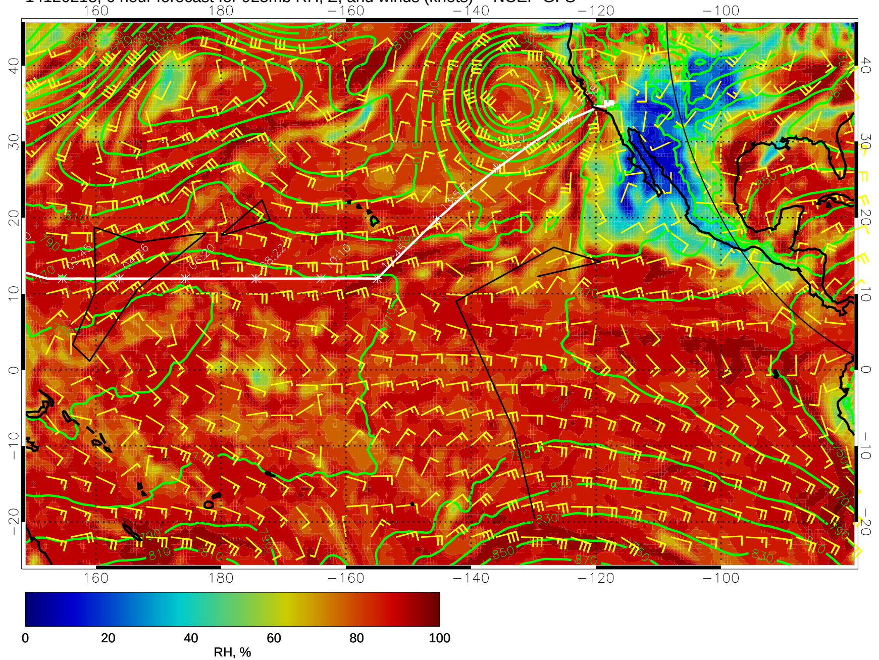
14120218, 6 hour forecast for 925mb RH, Z, and winds (knots) -- NCEP GFS
