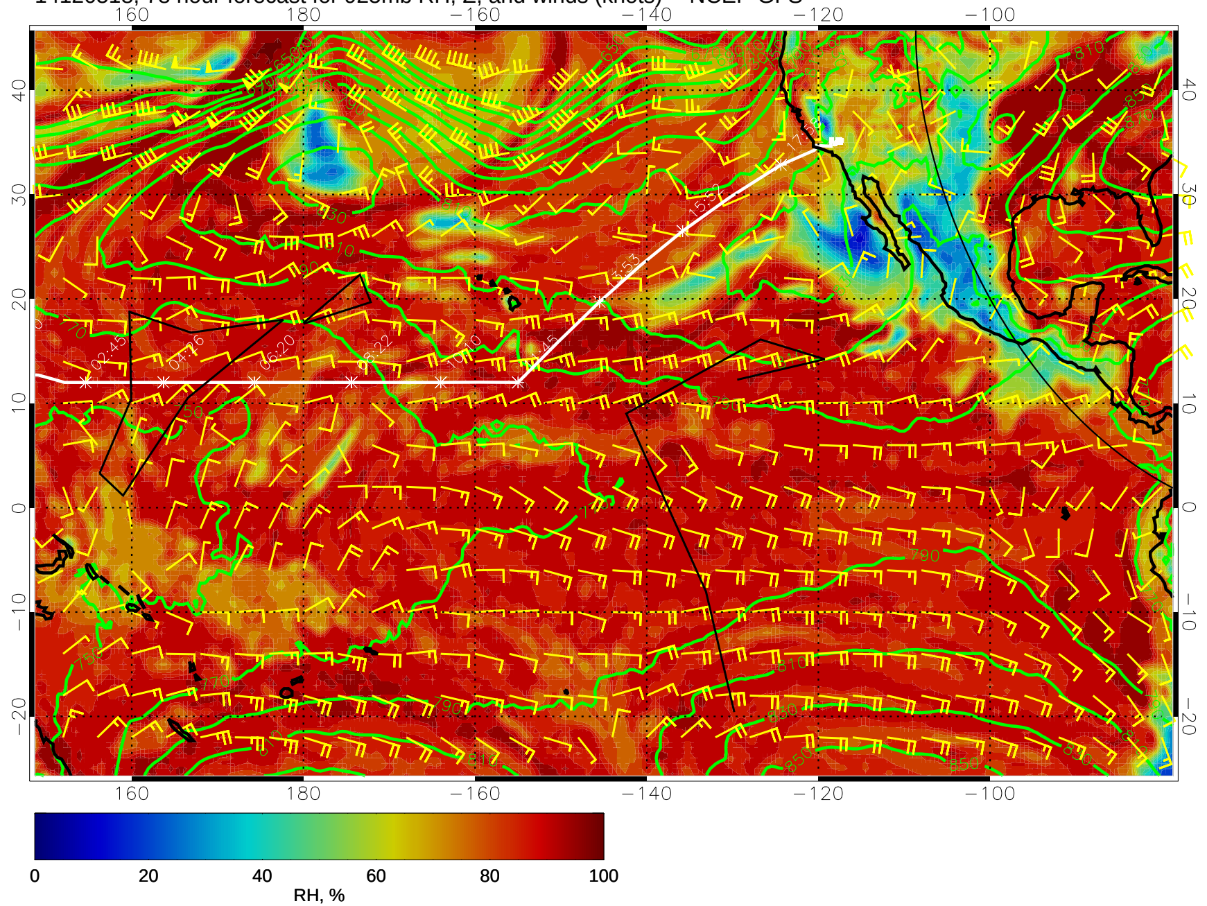
14120518, 78 hour forecast for 925mb RH, Z, and winds (knots) -- NCEP GFS
