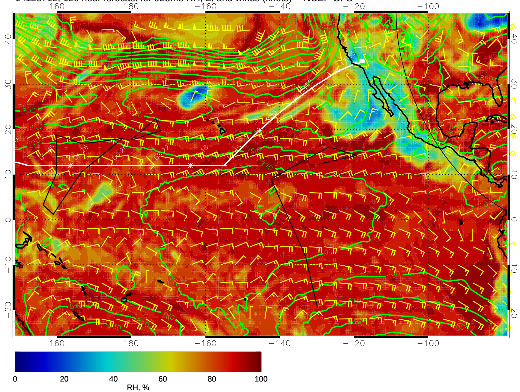
14120712, 120 hour forecast for 925mb RH, Z, and winds (knots) -- NCEP GFS
