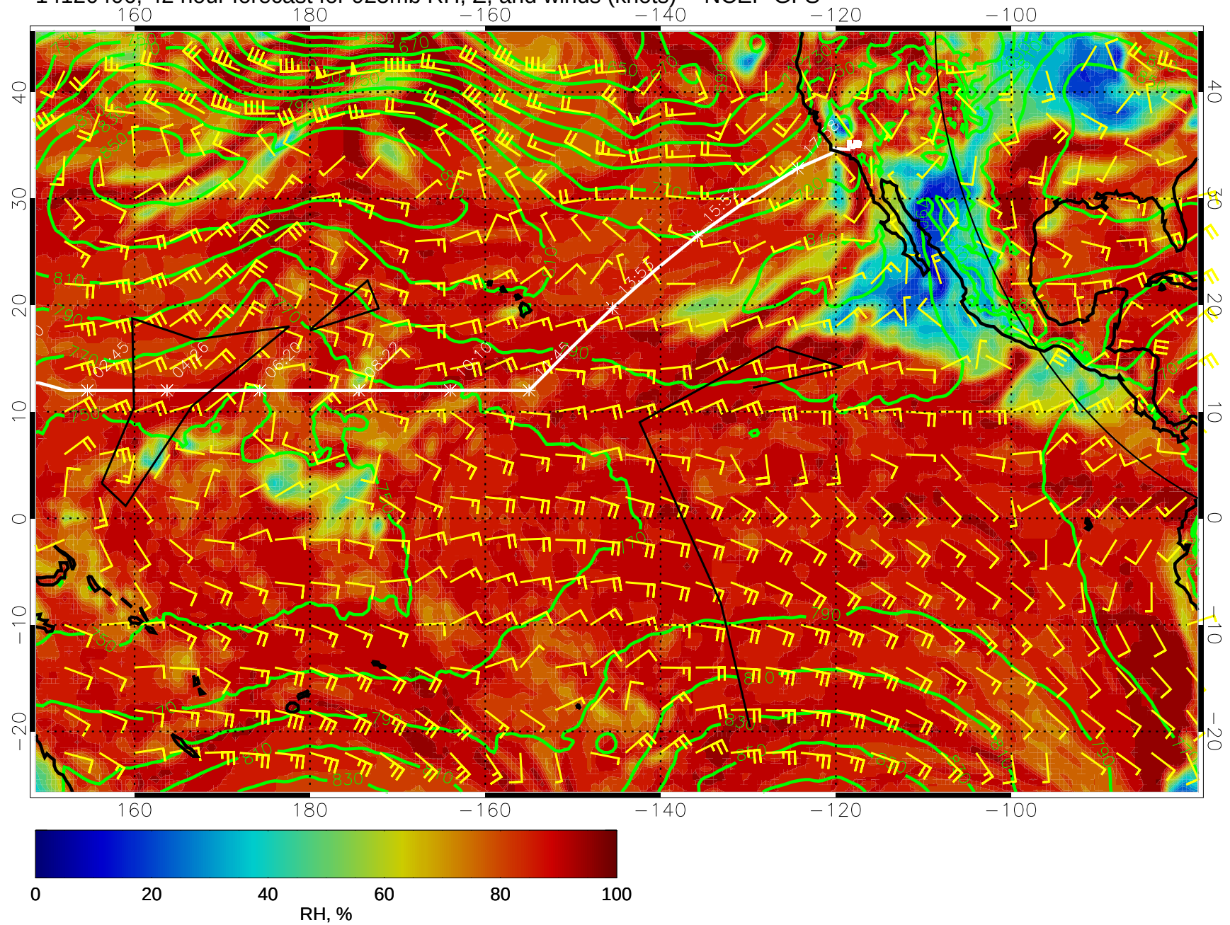
14120406, 42 hour forecast for 925mb RH, Z, and winds (knots) -- NCEP GFS
