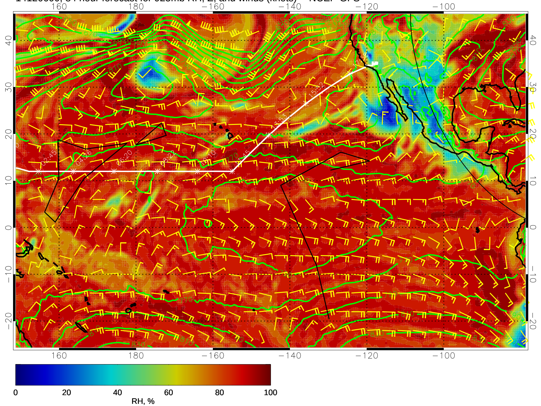
14120600, 84 hour forecast for 925mb RH, Z, and winds (knots) -- NCEP GFS
