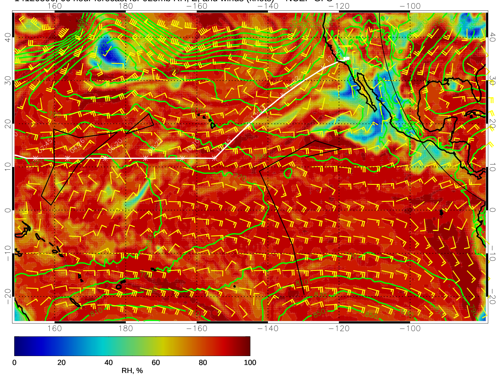
14120506, 66 hour forecast for 925mb RH, Z, and winds (knots) -- NCEP GFS
