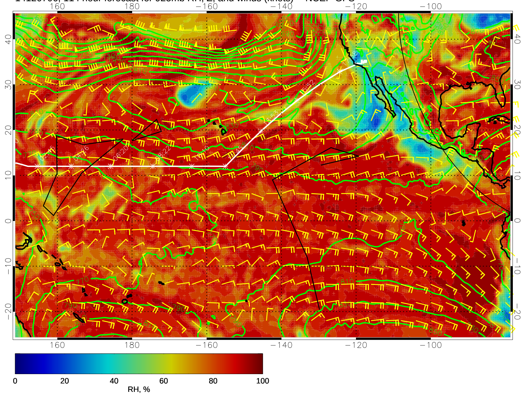
14120706, 114 hour forecast for 925mb RH, Z, and winds (knots) -- NCEP GFS
