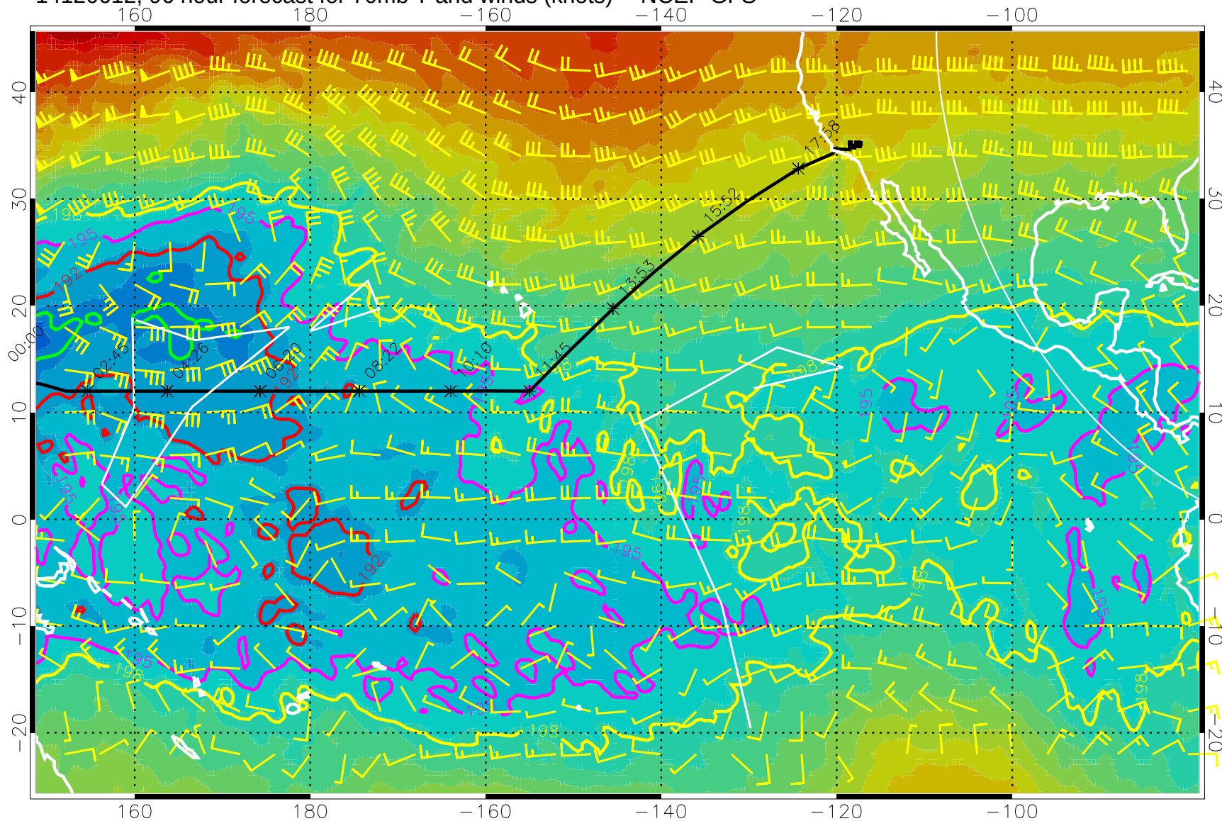
14120612, 96 hour forecast for 70mb T and winds (knots) -- NCEP GFS
