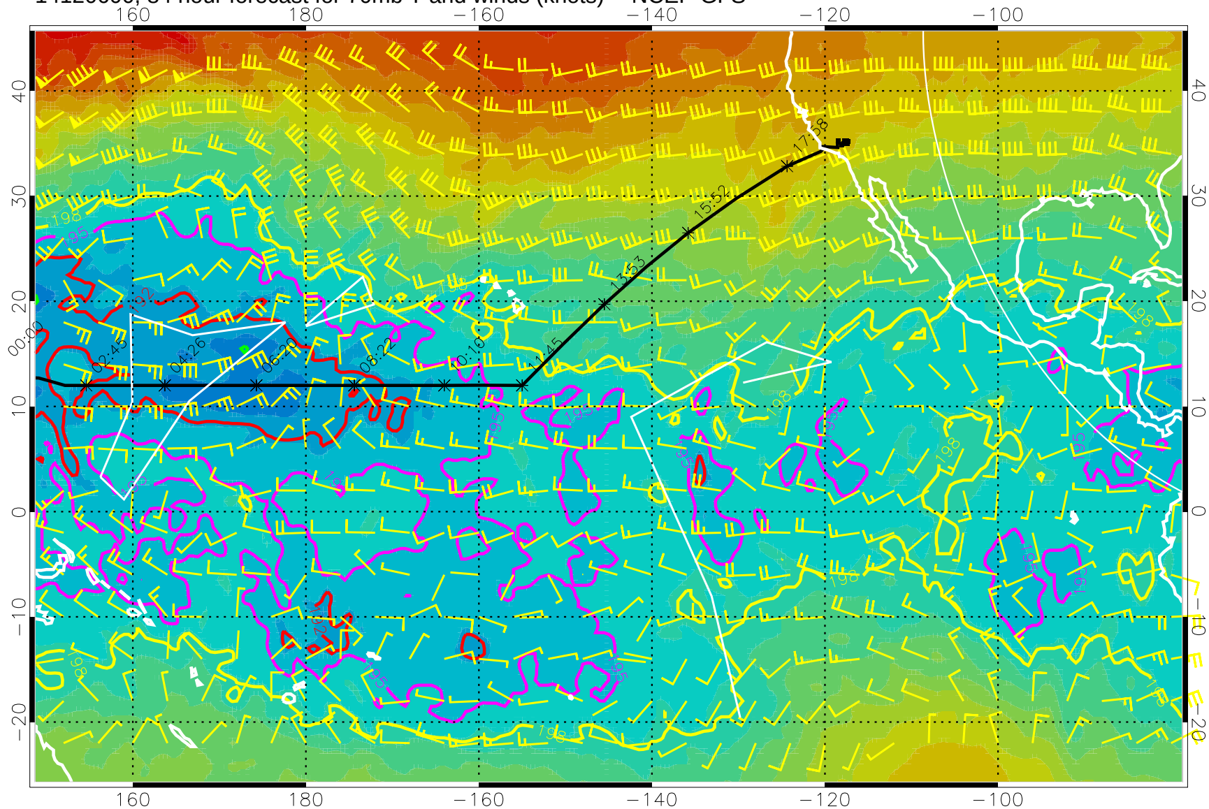
14120600, 84 hour forecast for 70mb T and winds (knots) -- NCEP GFS
