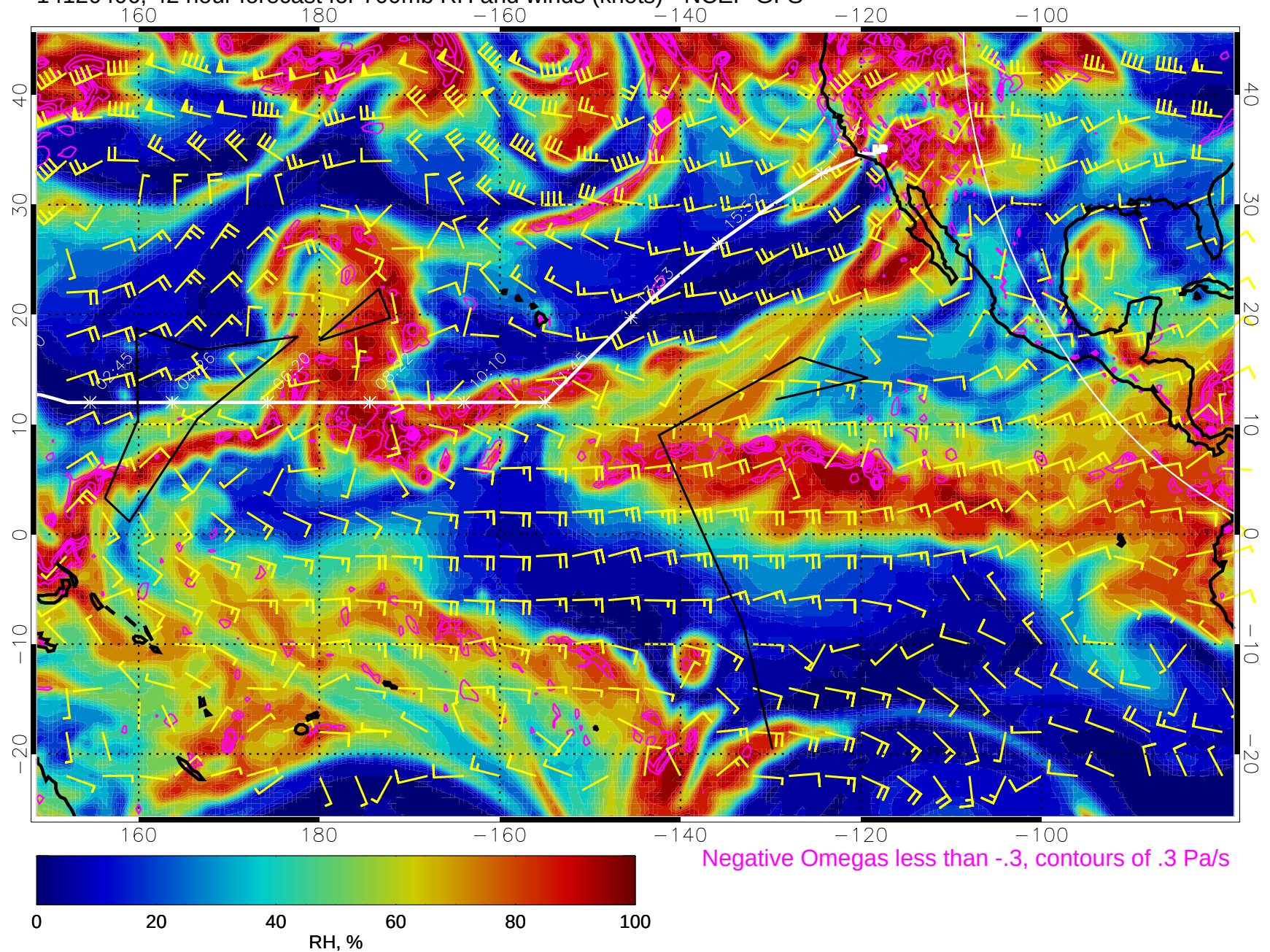
14120406, 42 hour forecast for 700mb RH and winds (knots) - NCEP GFS
