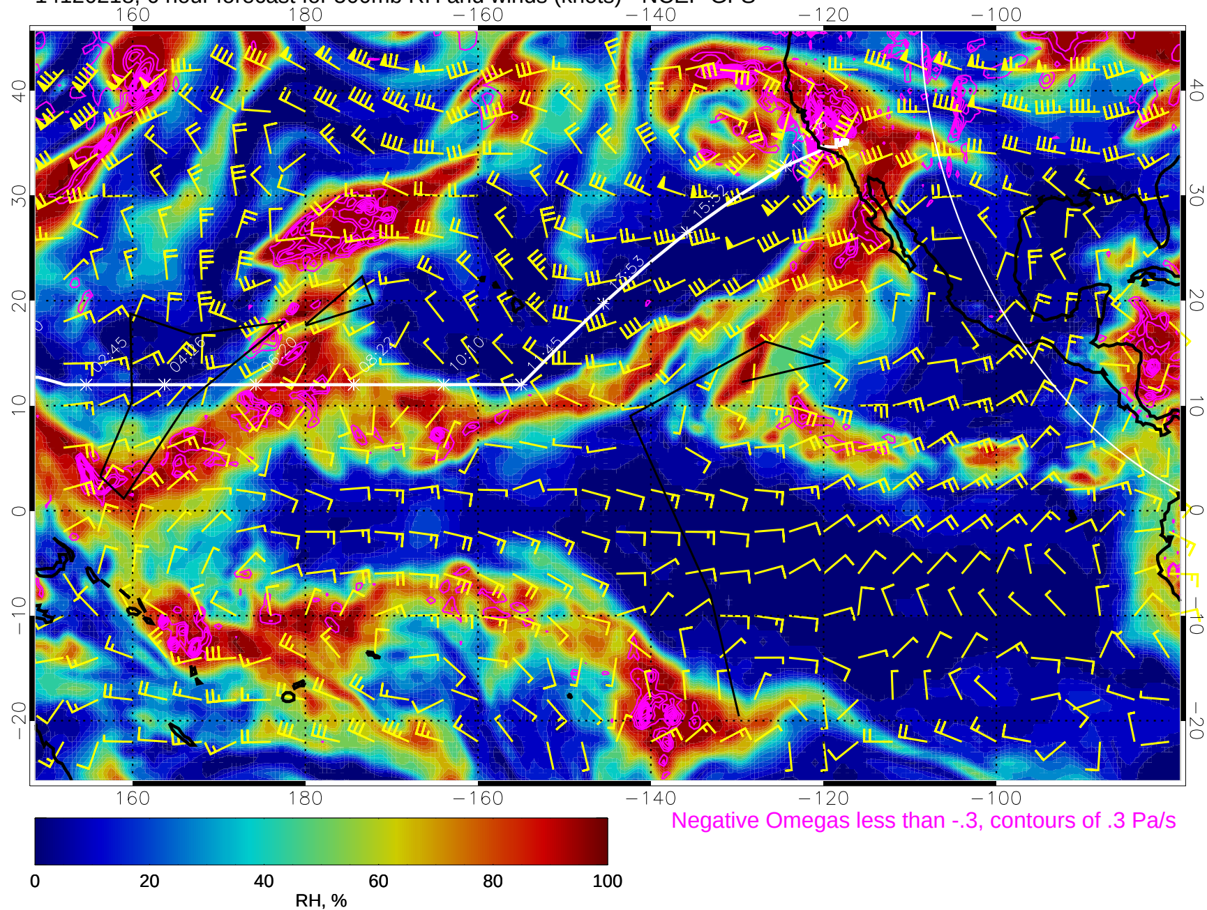
14120218, 6 hour forecast for 500mb RH and winds (knots) - NCEP GFS
