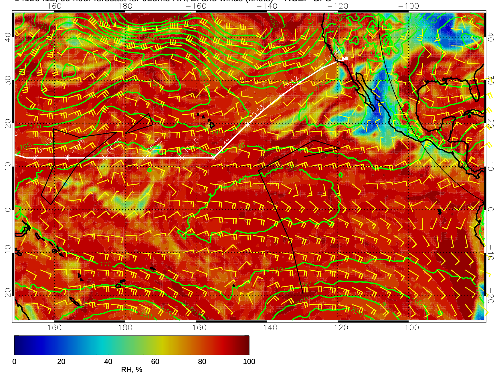
14120412, 60 hour forecast for 925mb RH, Z, and winds (knots) -- NCEP GFS
