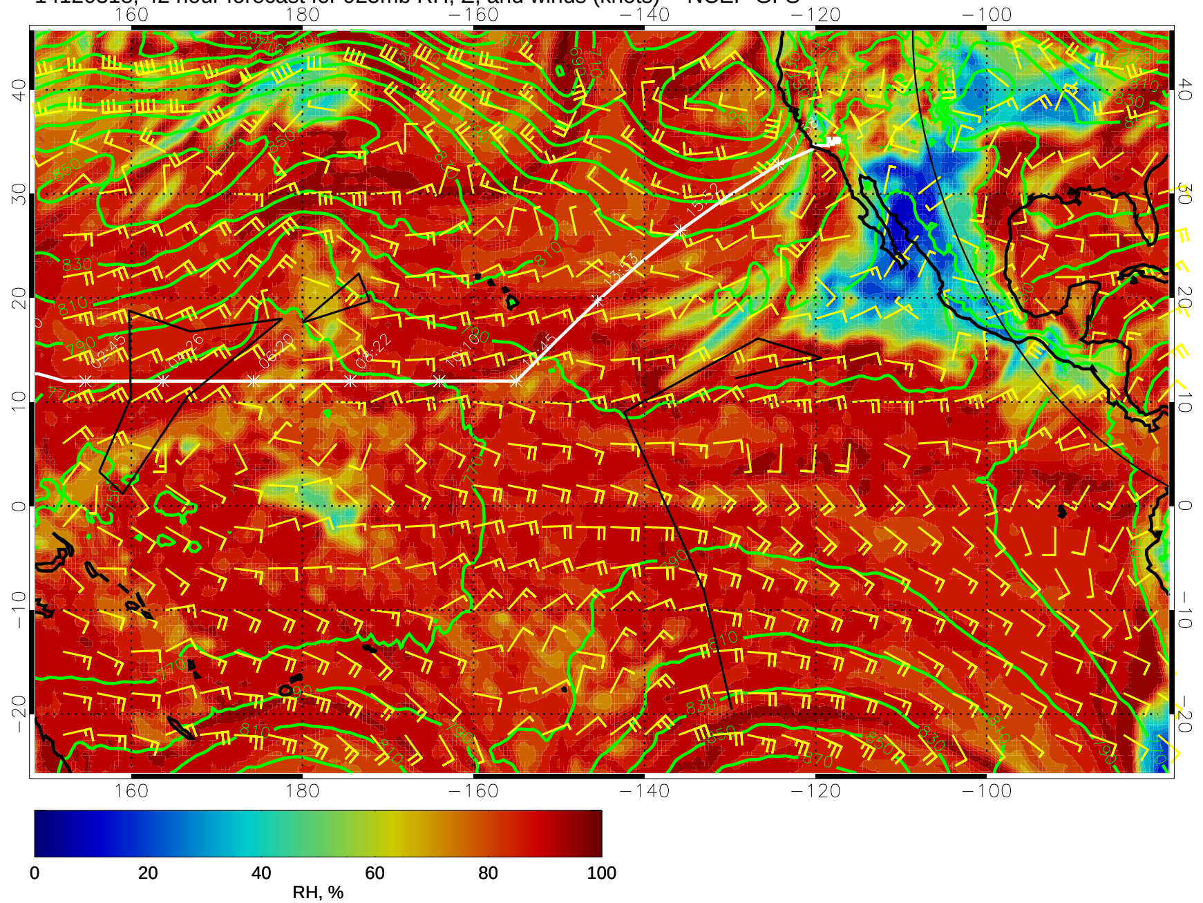
14120318, 42 hour forecast for 925mb RH, Z, and winds (knots) -- NCEP GFS
