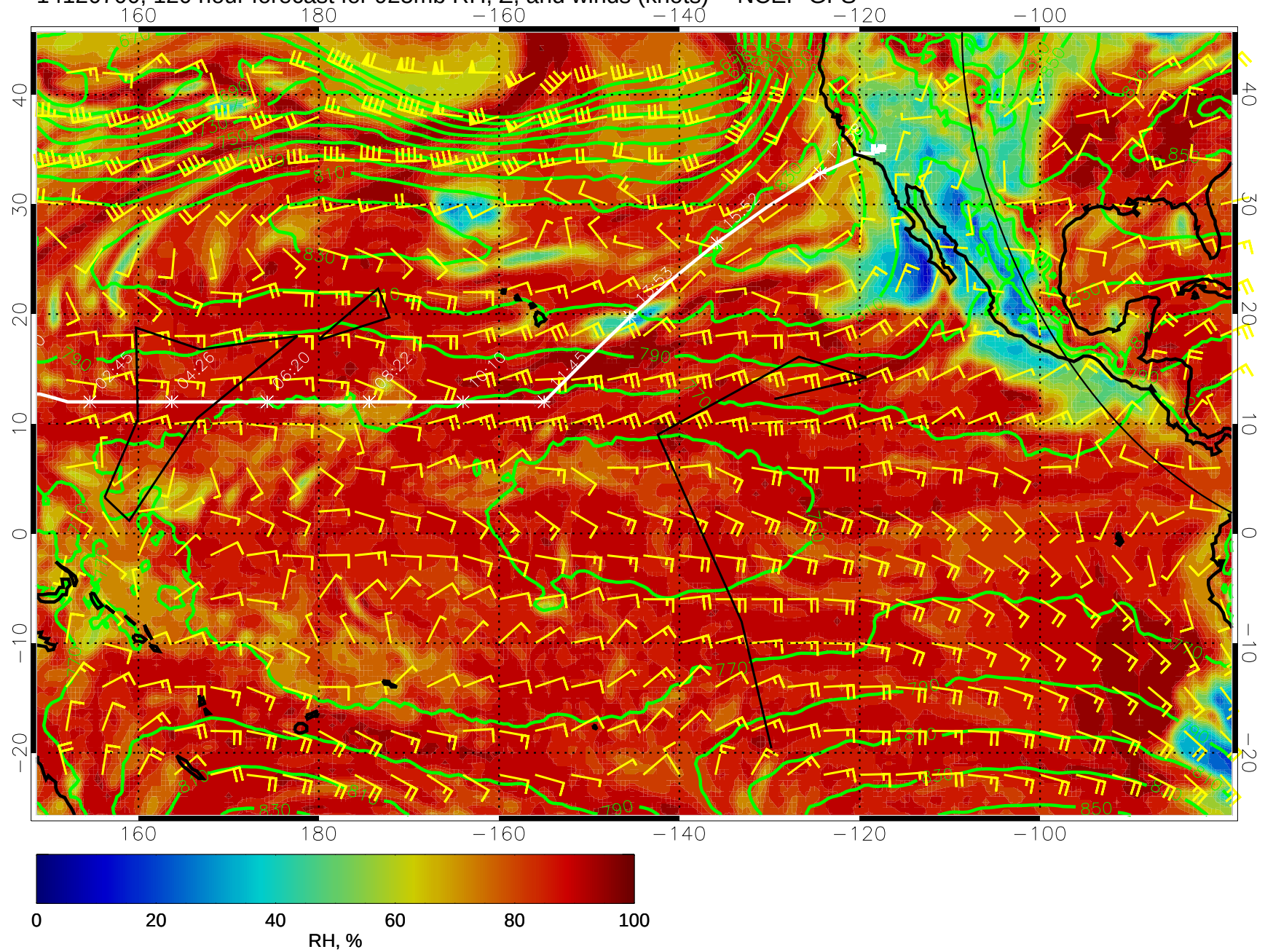
14120700, 120 hour forecast for 925mb RH, Z, and winds (knots) -- NCEP GFS
