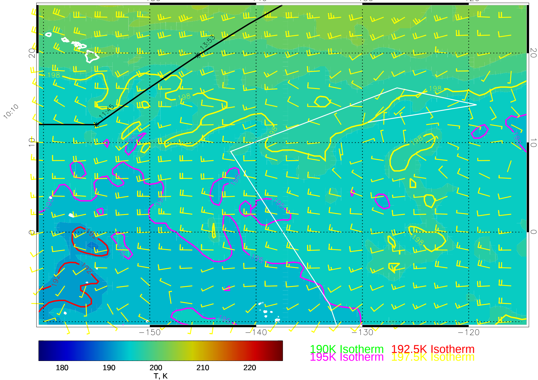
14120612, 108 hour forecast for 70mb T and winds (knots) -- NCEP GFS
