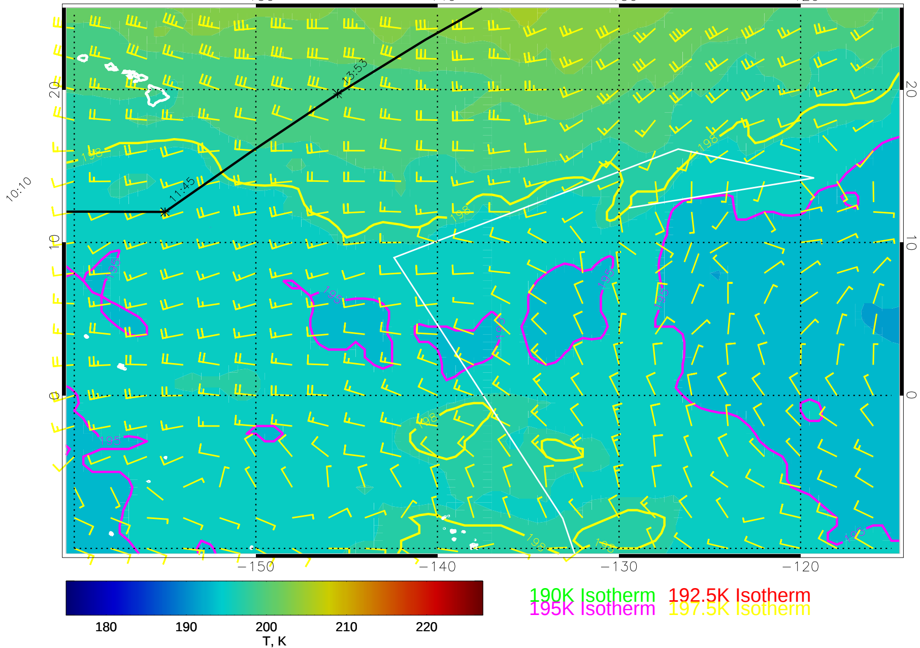
14120312, 36 hour forecast for 70mb T and winds (knots) -- NCEP GFS
