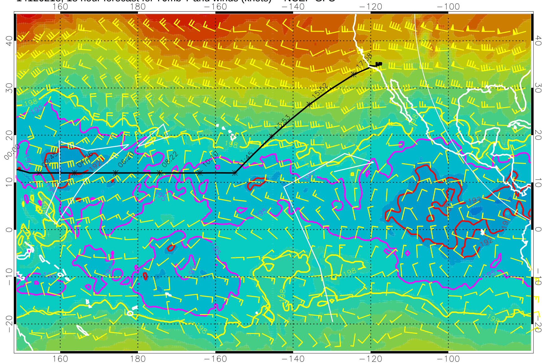
14120218, 18 hour forecast for 70mb T and winds (knots) -- NCEP GFS
