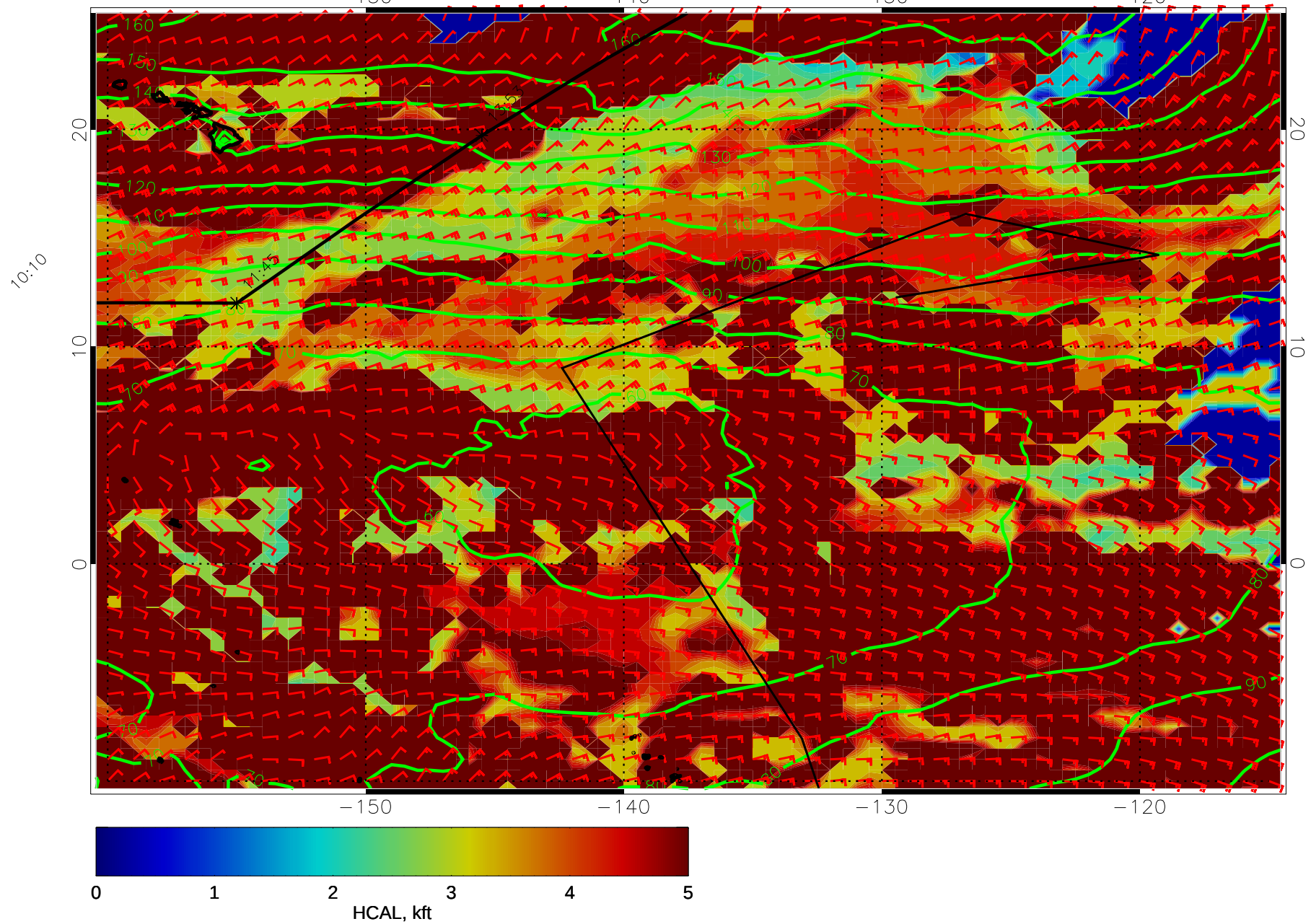
14120700, 120 hour forecast for HCAL, 1000mb Z, and winds (knots) -- NCEP GFS
