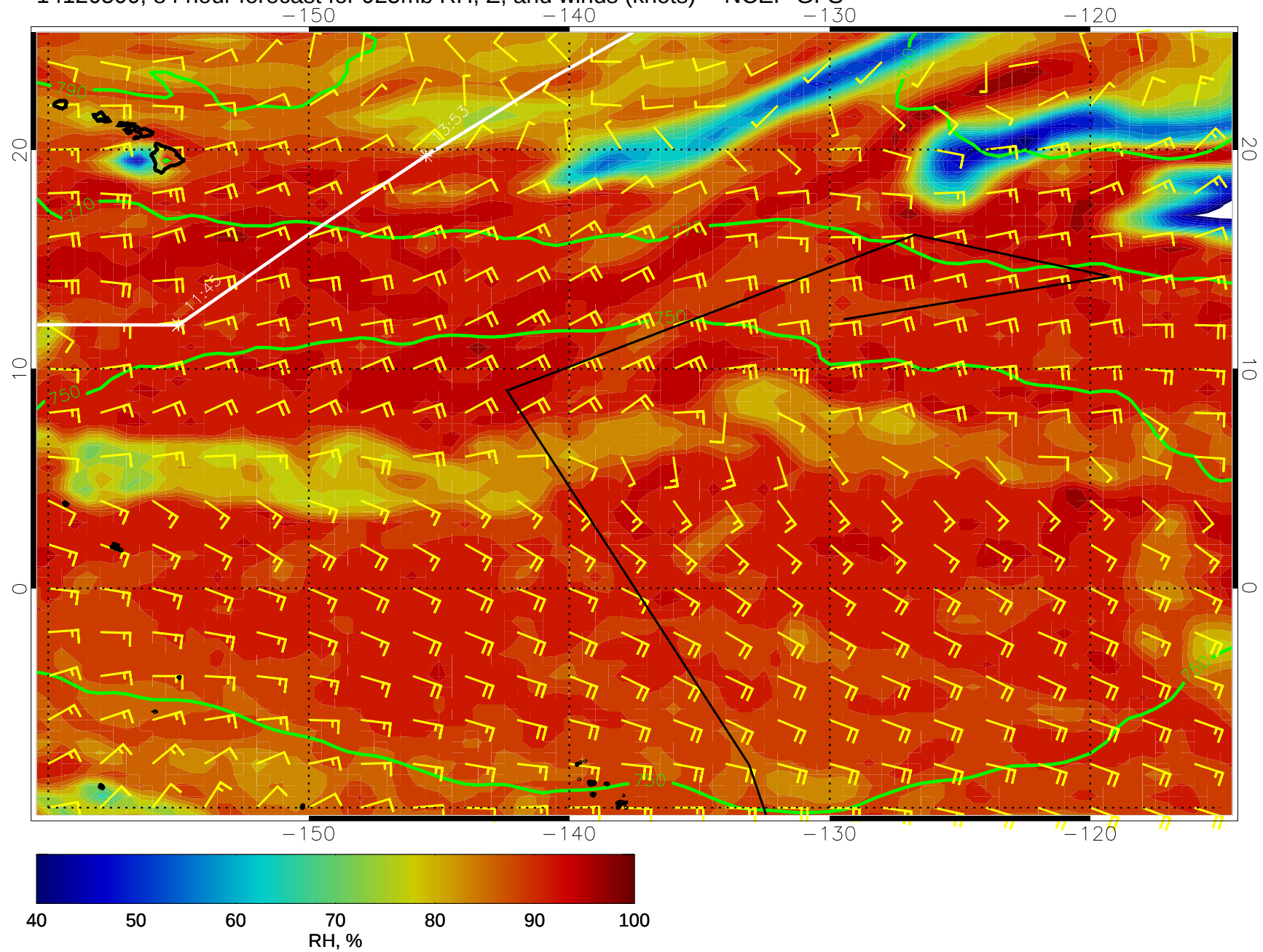
14120500, 84 hour forecast for 925mb RH, Z, and winds (knots) -- NCEP GFS
