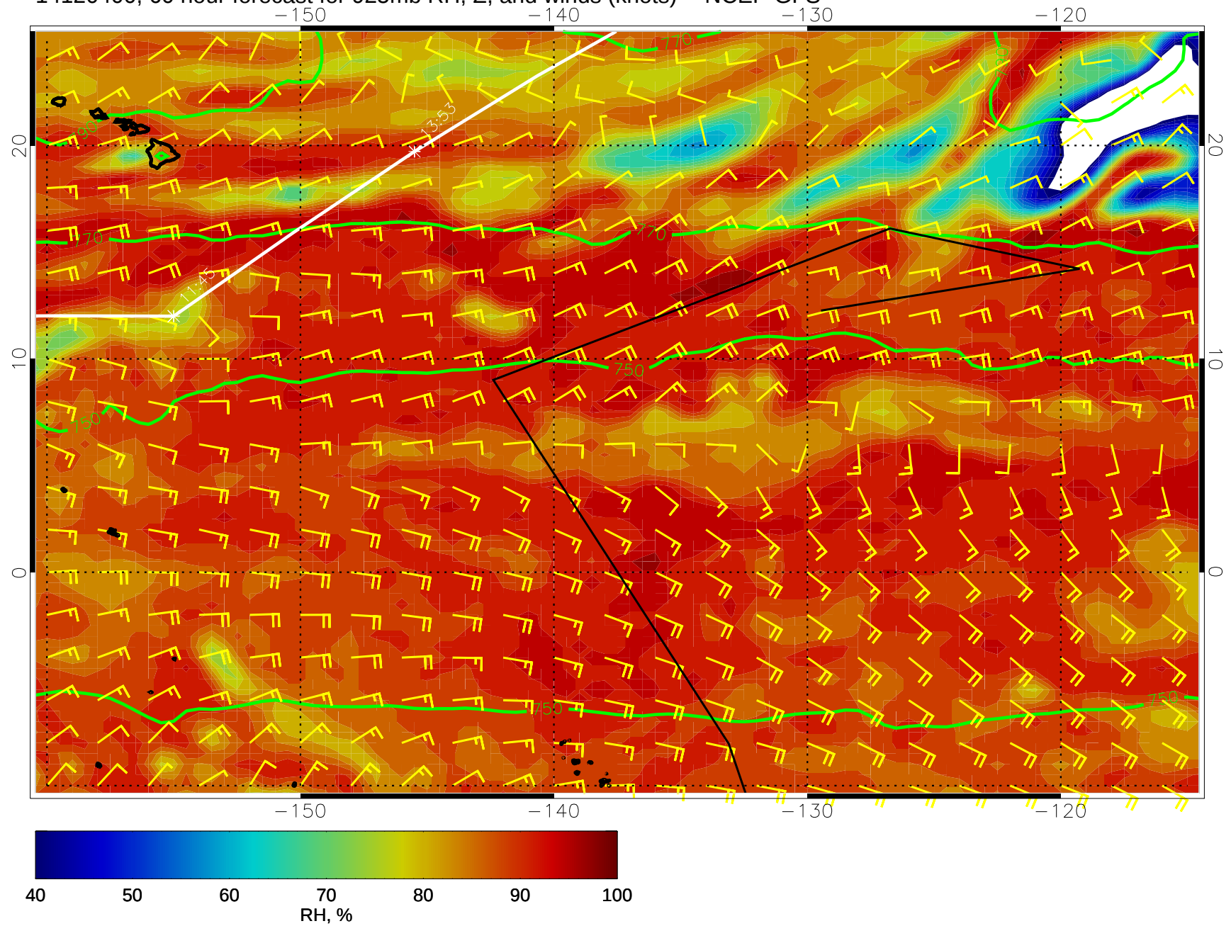
14120400, 60 hour forecast for 925mb RH, Z, and winds (knots) -- NCEP GFS
