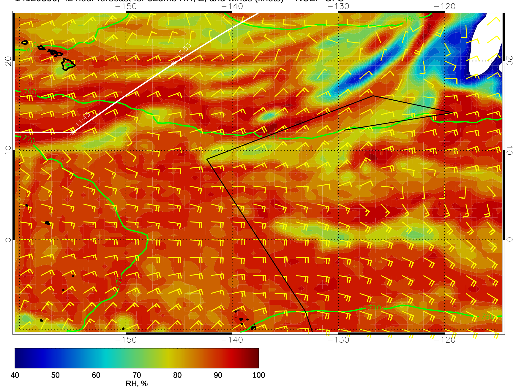
14120306, 42 hour forecast for 925mb RH, Z, and winds (knots) -- NCEP GFS
