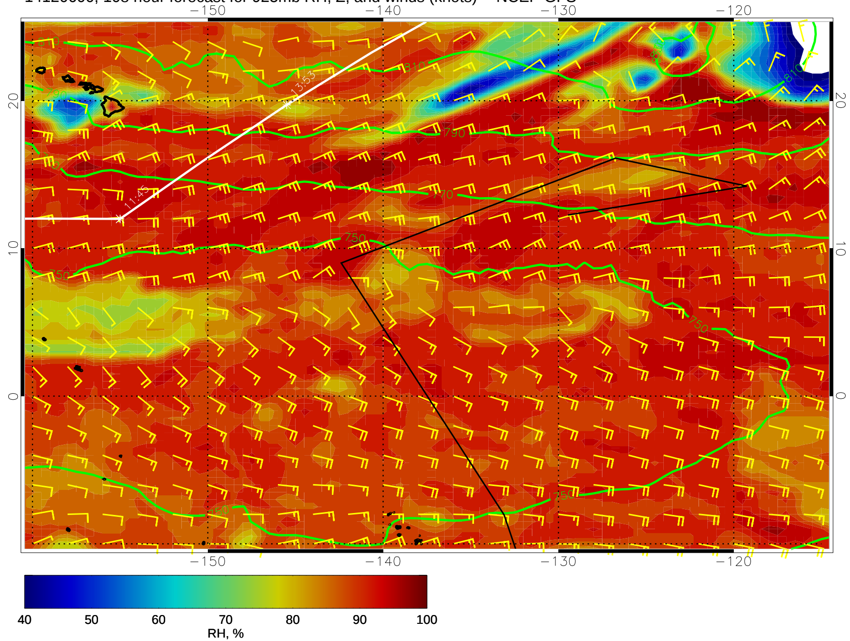
14120600, 108 hour forecast for 925mb RH, Z, and winds (knots) -- NCEP GFS
