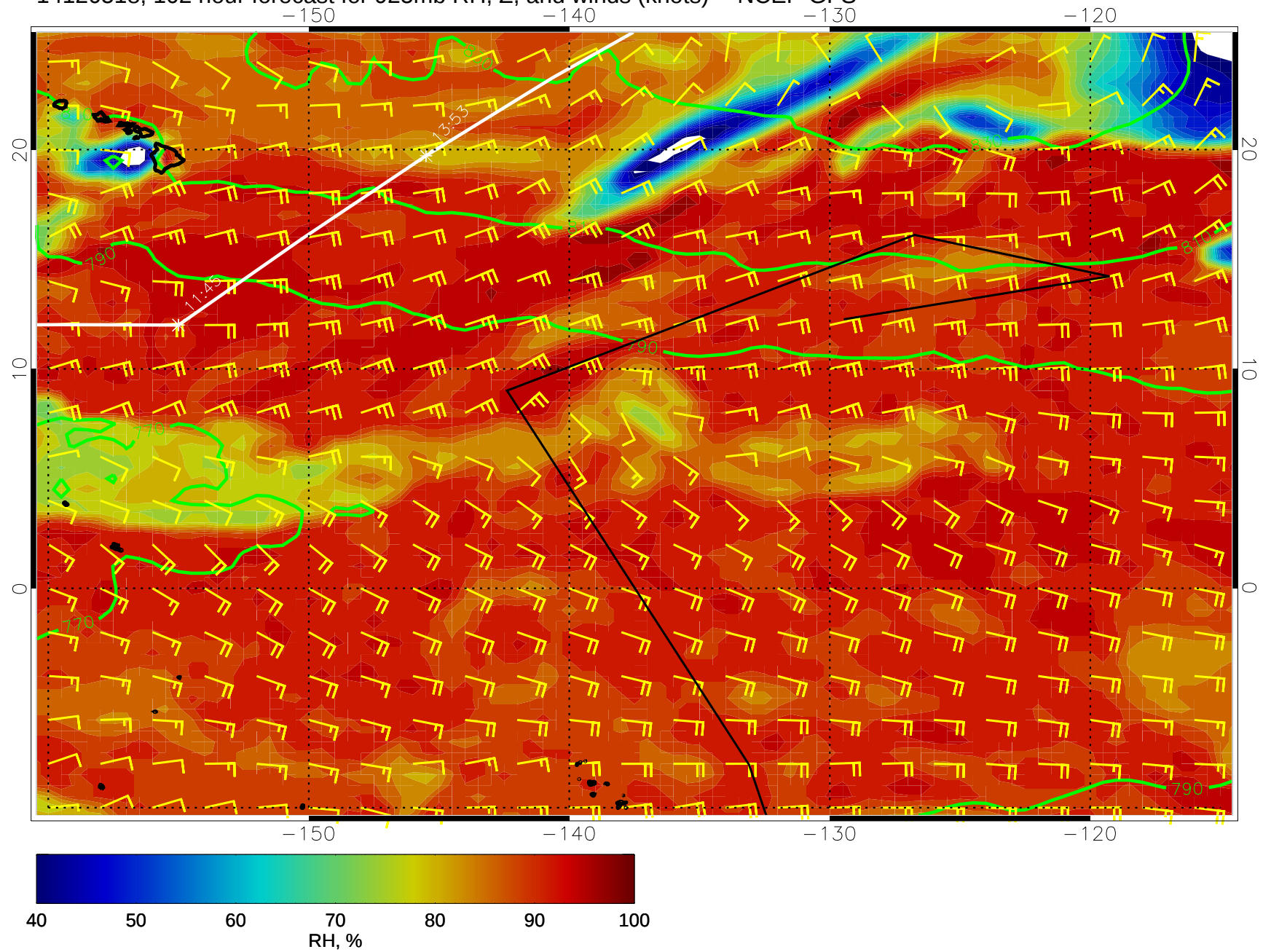
14120518, 102 hour forecast for 925mb RH, Z, and winds (knots) -- NCEP GFS
