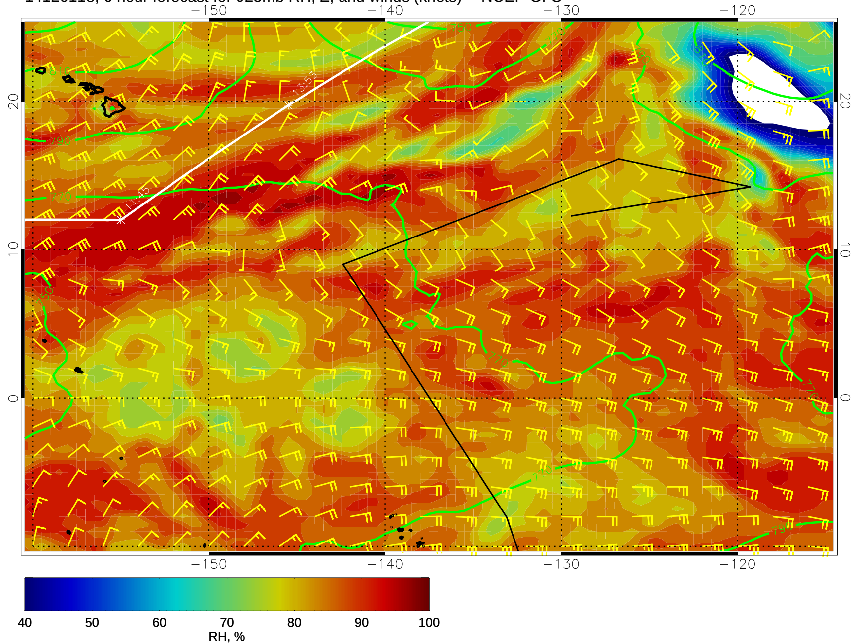
14120118, 6 hour forecast for 925mb RH, Z, and winds (knots) -- NCEP GFS
