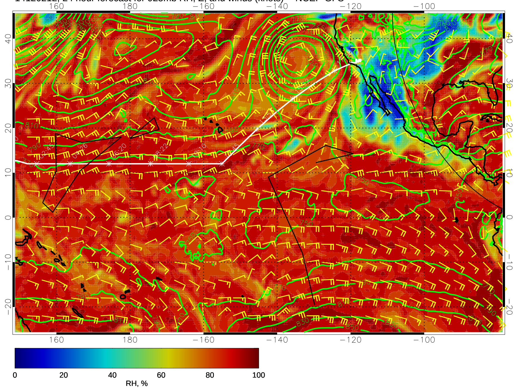
14120212, 24 hour forecast for 925mb RH, Z, and winds (knots) -- NCEP GFS
