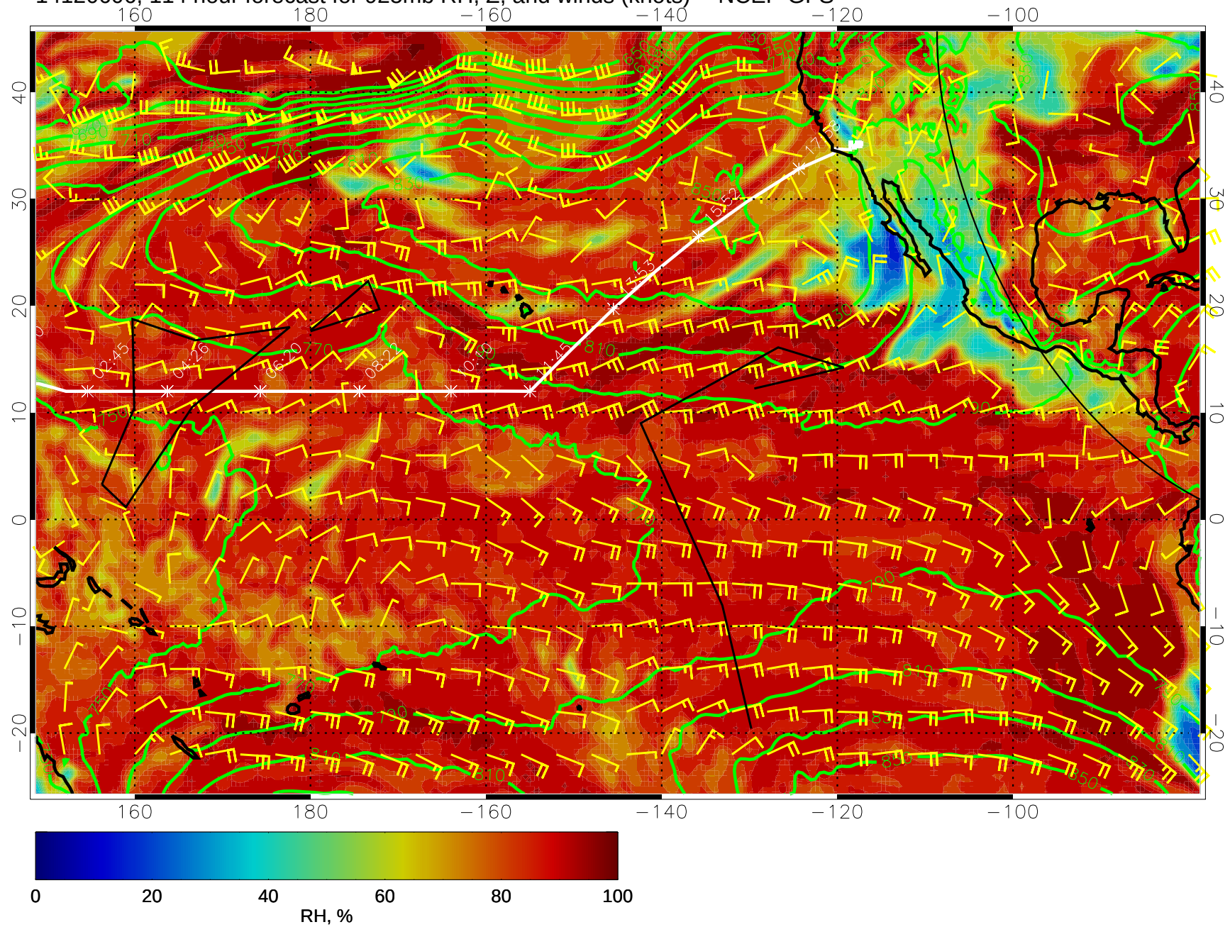
14120606, 114 hour forecast for 925mb RH, Z, and winds (knots) -- NCEP GFS
