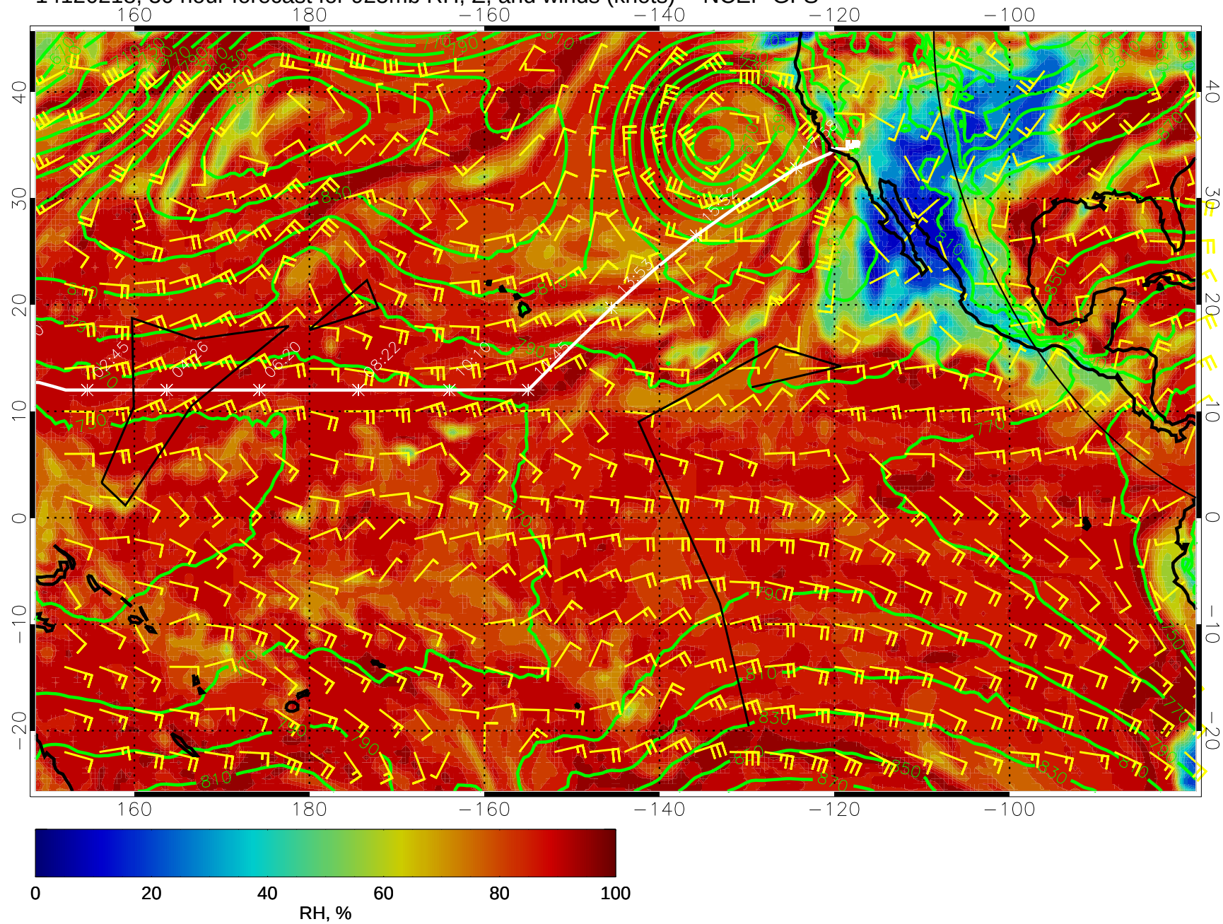
14120218, 30 hour forecast for 925mb RH, Z, and winds (knots) -- NCEP GFS
