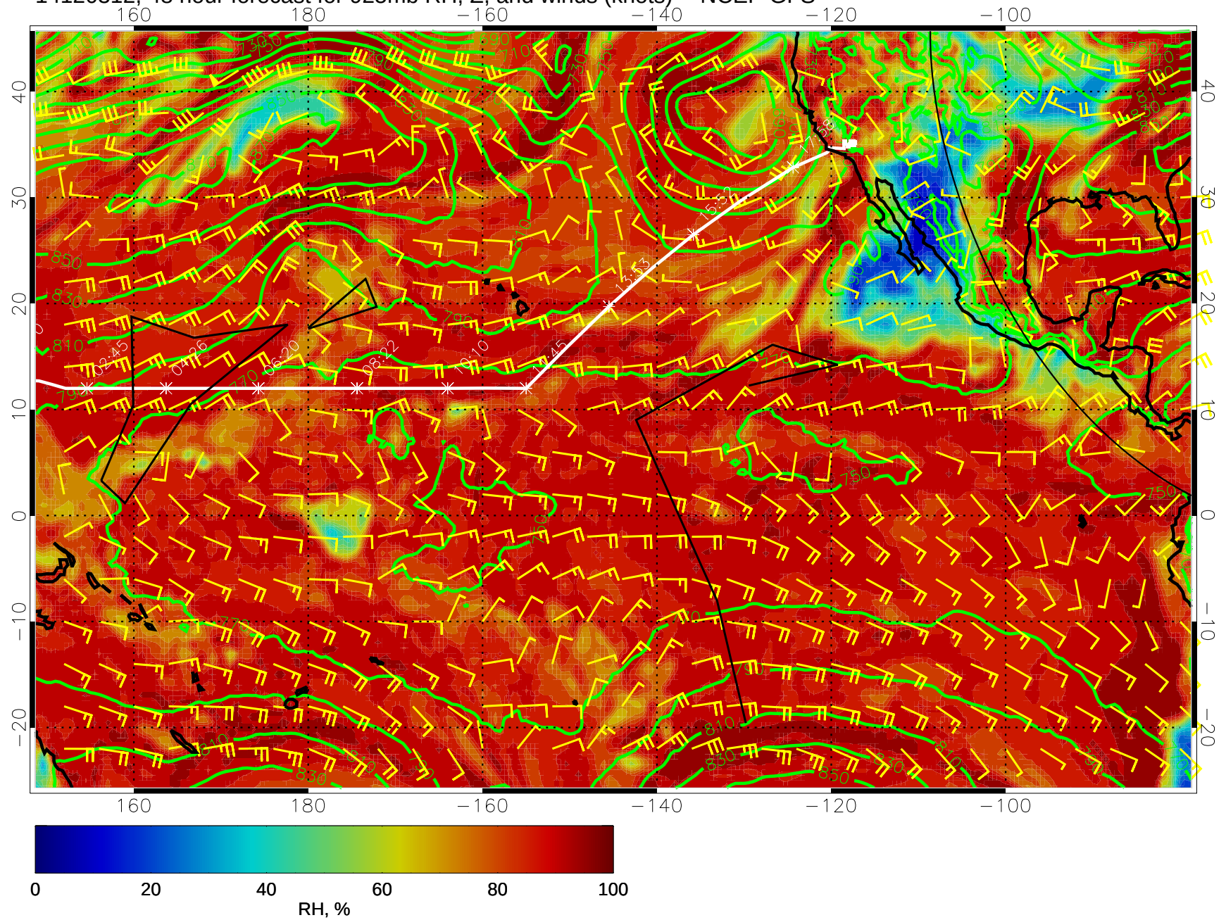
14120312, 48 hour forecast for 925mb RH, Z, and winds (knots) -- NCEP GFS
