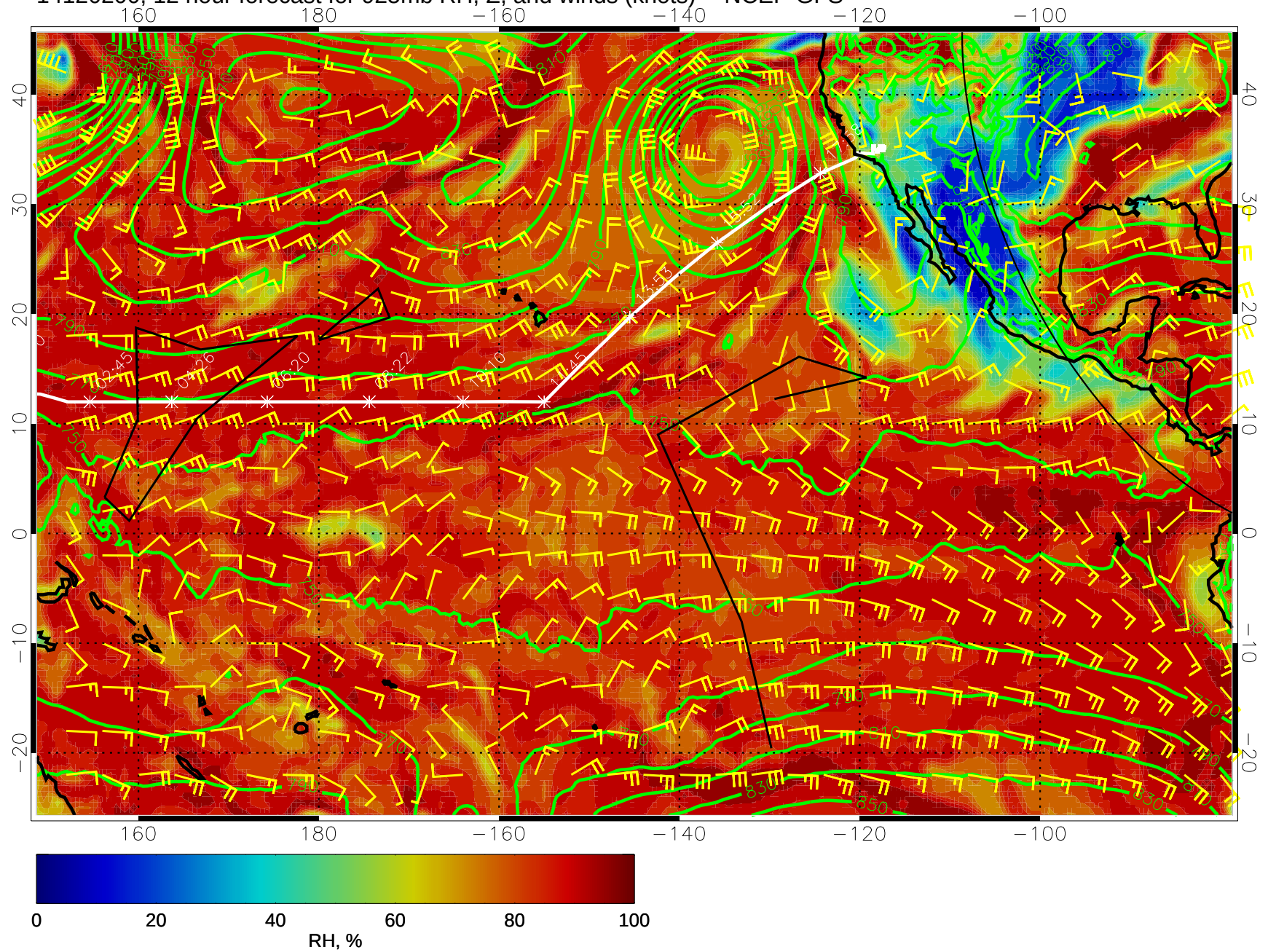
14120200, 12 hour forecast for 925mb RH, Z, and winds (knots) -- NCEP GFS
