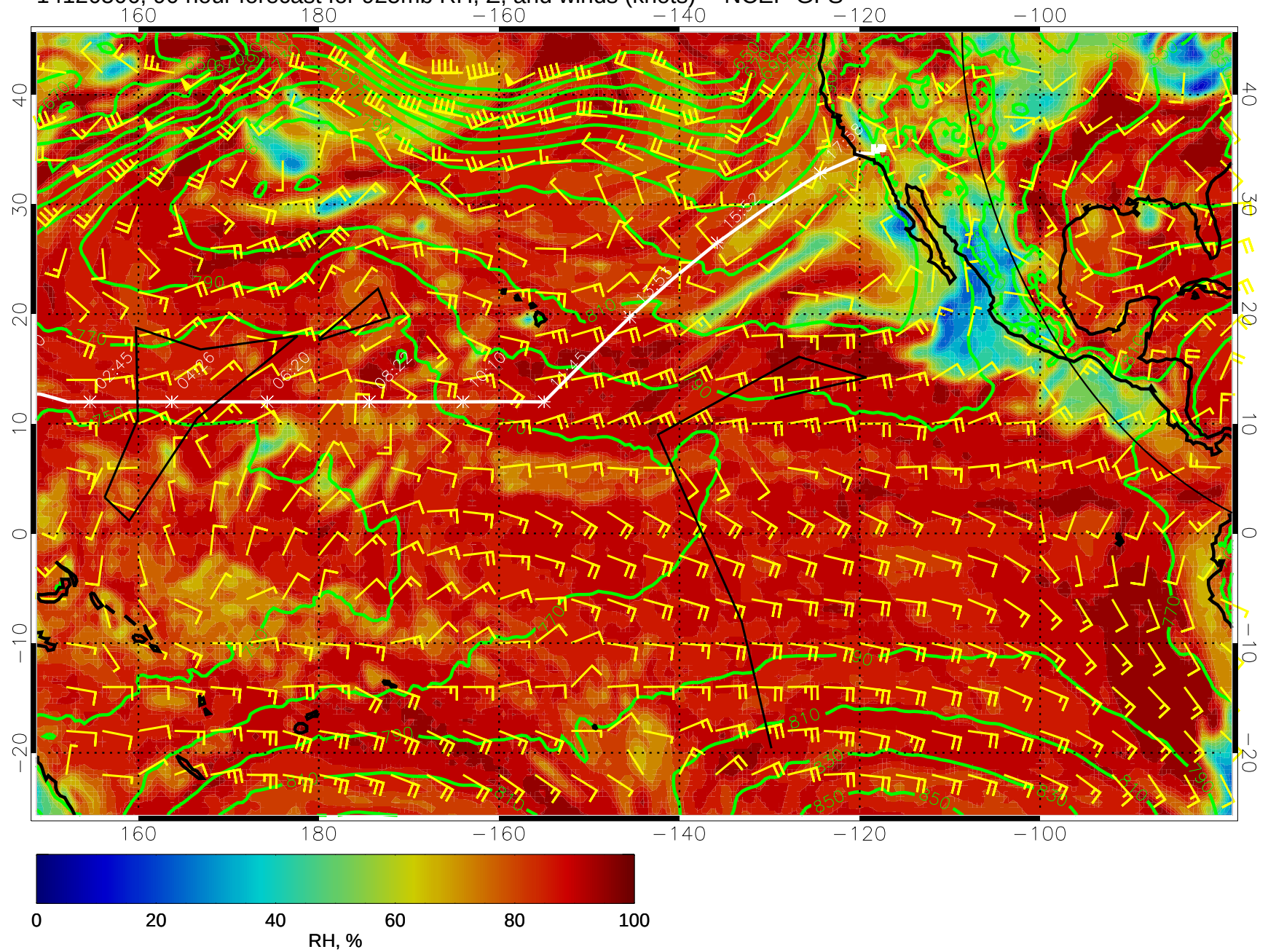
14120506, 90 hour forecast for 925mb RH, Z, and winds (knots) -- NCEP GFS
