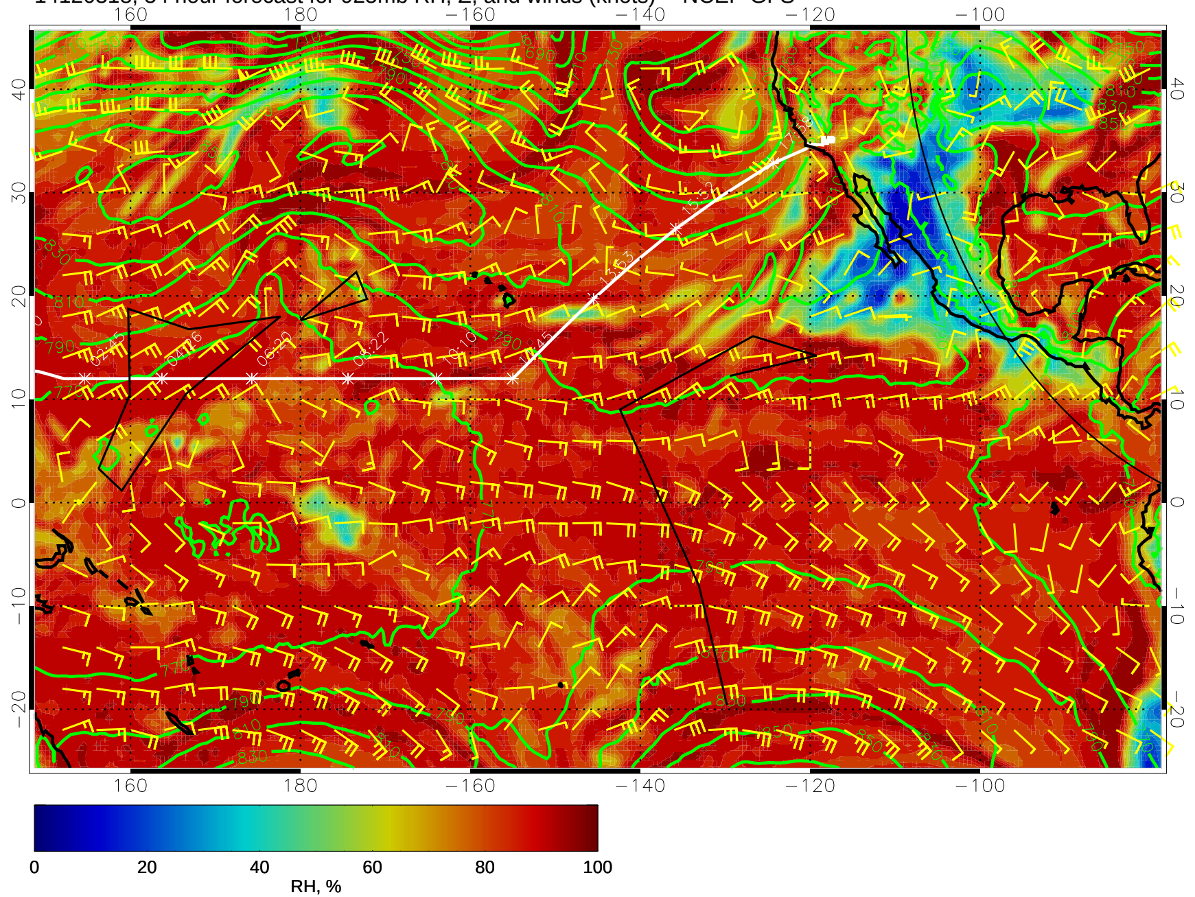
14120318, 54 hour forecast for 925mb RH, Z, and winds (knots) -- NCEP GFS
