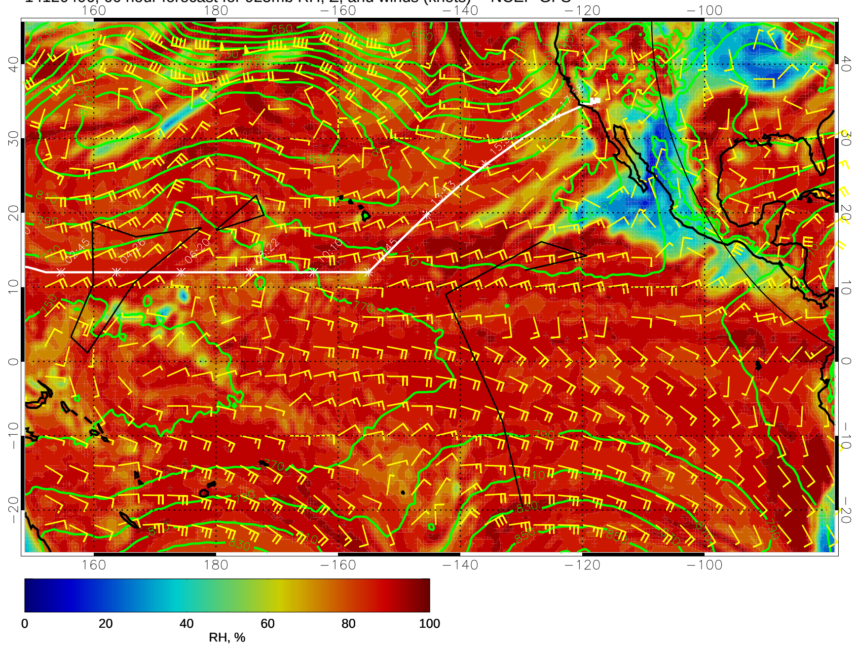
14120406, 66 hour forecast for 925mb RH, Z, and winds (knots) -- NCEP GFS
