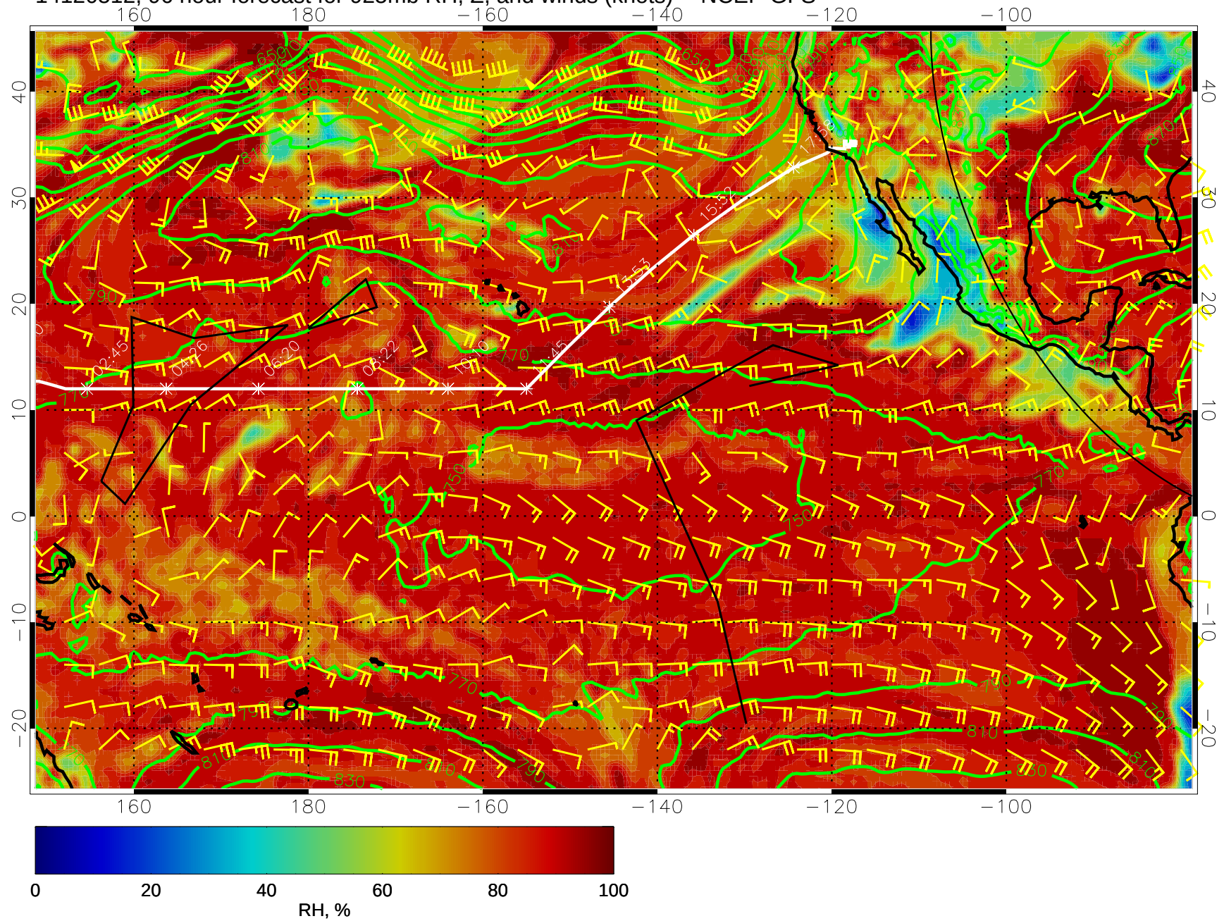
14120512, 96 hour forecast for 925mb RH, Z, and winds (knots) -- NCEP GFS
