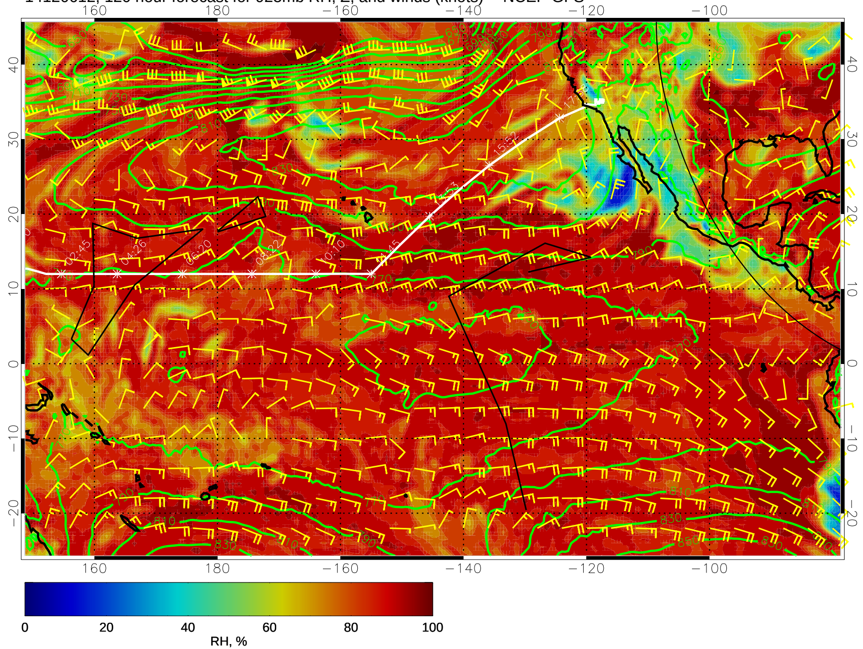
14120612, 120 hour forecast for 925mb RH, Z, and winds (knots) -- NCEP GFS
