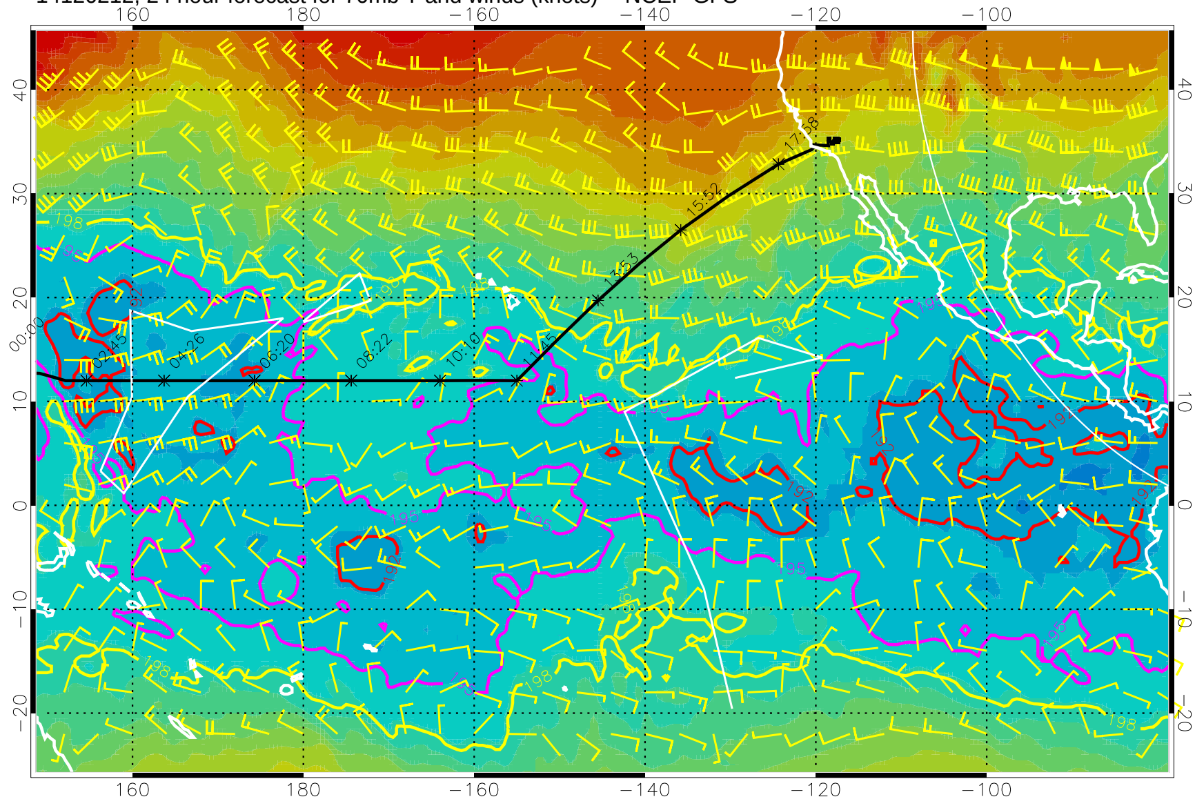
14120212, 24 hour forecast for 70mb T and winds (knots) -- NCEP GFS
