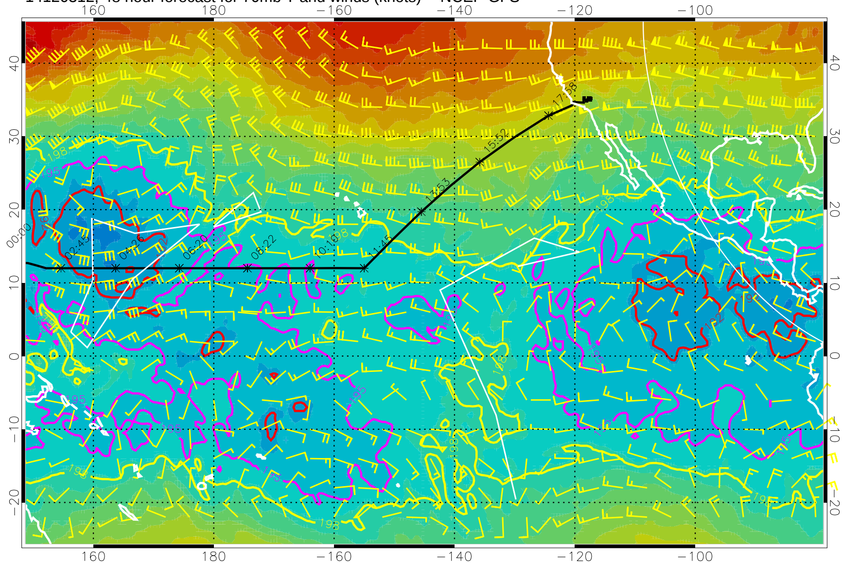
14120312, 48 hour forecast for 70mb T and winds (knots) -- NCEP GFS
