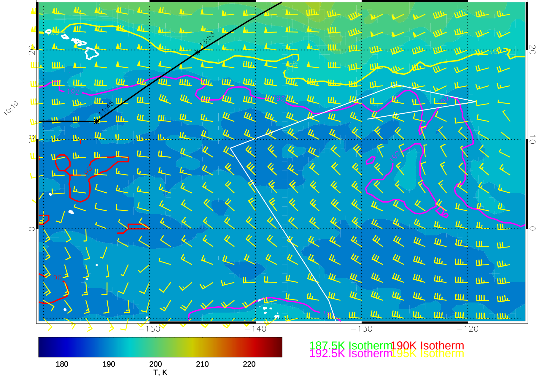
14120318, 54 hour forecast for 100mb T and winds (knots) -- NCEP GFS
