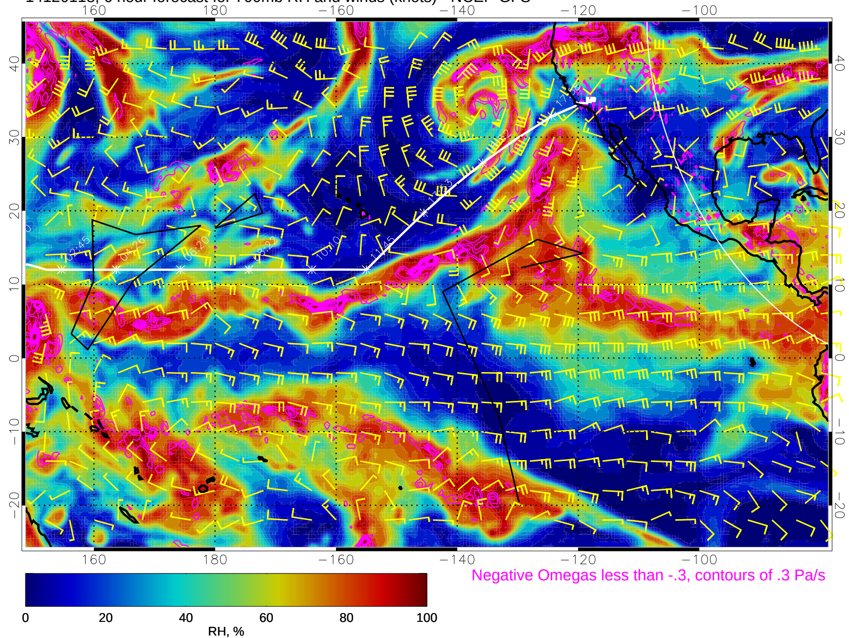
14120118, 6 hour forecast for 700mb RH and winds (knots) - NCEP GFS
