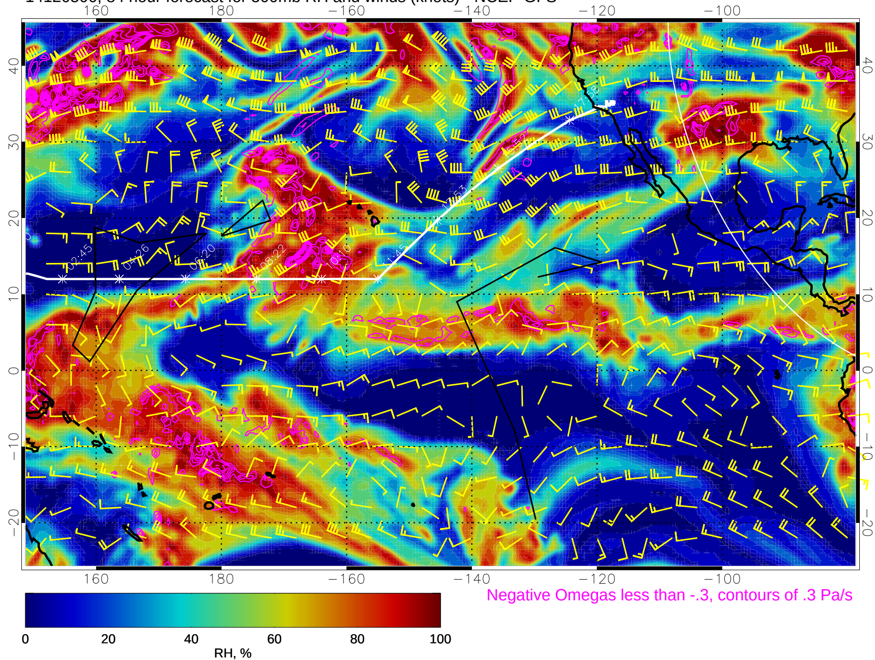
14120500, 84 hour forecast for 500mb RH and winds (knots) - NCEP GFS
