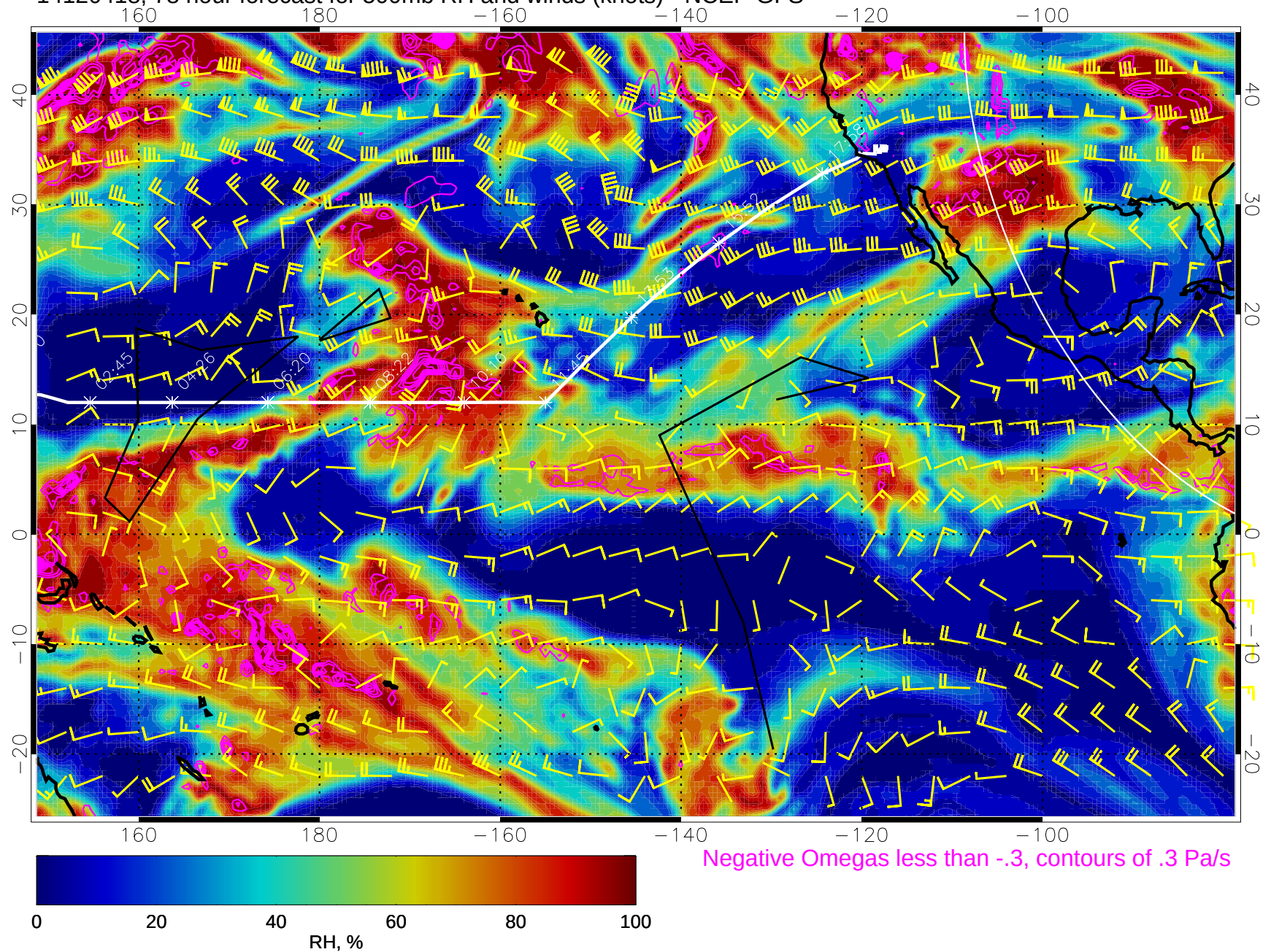
14120418, 78 hour forecast for 500mb RH and winds (knots) - NCEP GFS
