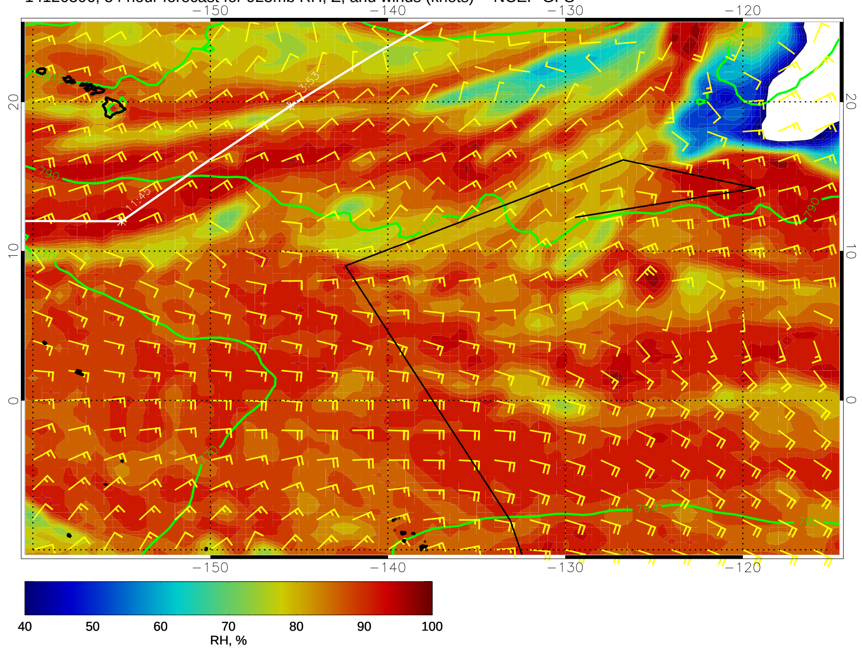
14120306, 54 hour forecast for 925mb RH, Z, and winds (knots) -- NCEP GFS
