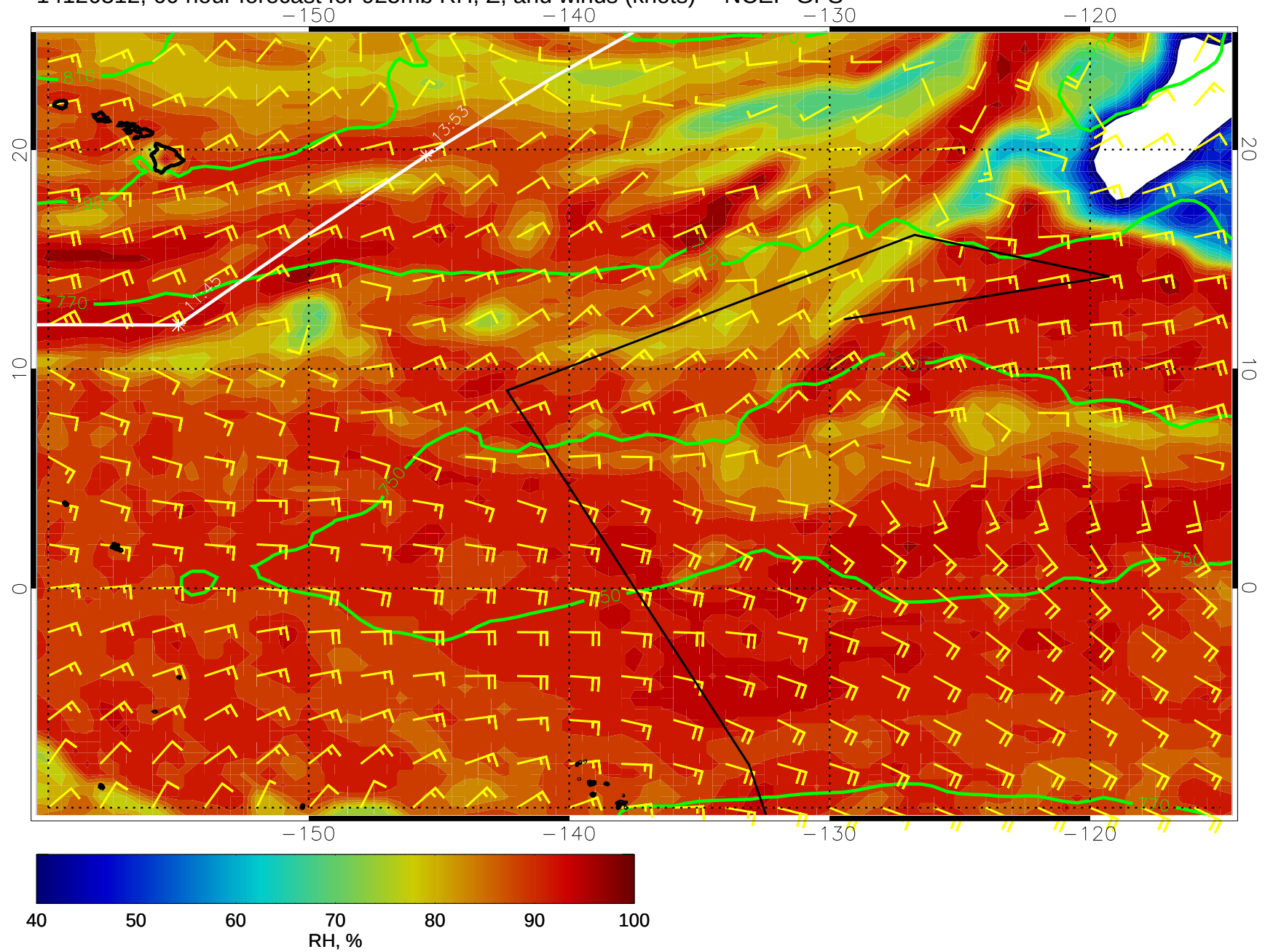
14120312, 60 hour forecast for 925mb RH, Z, and winds (knots) -- NCEP GFS
