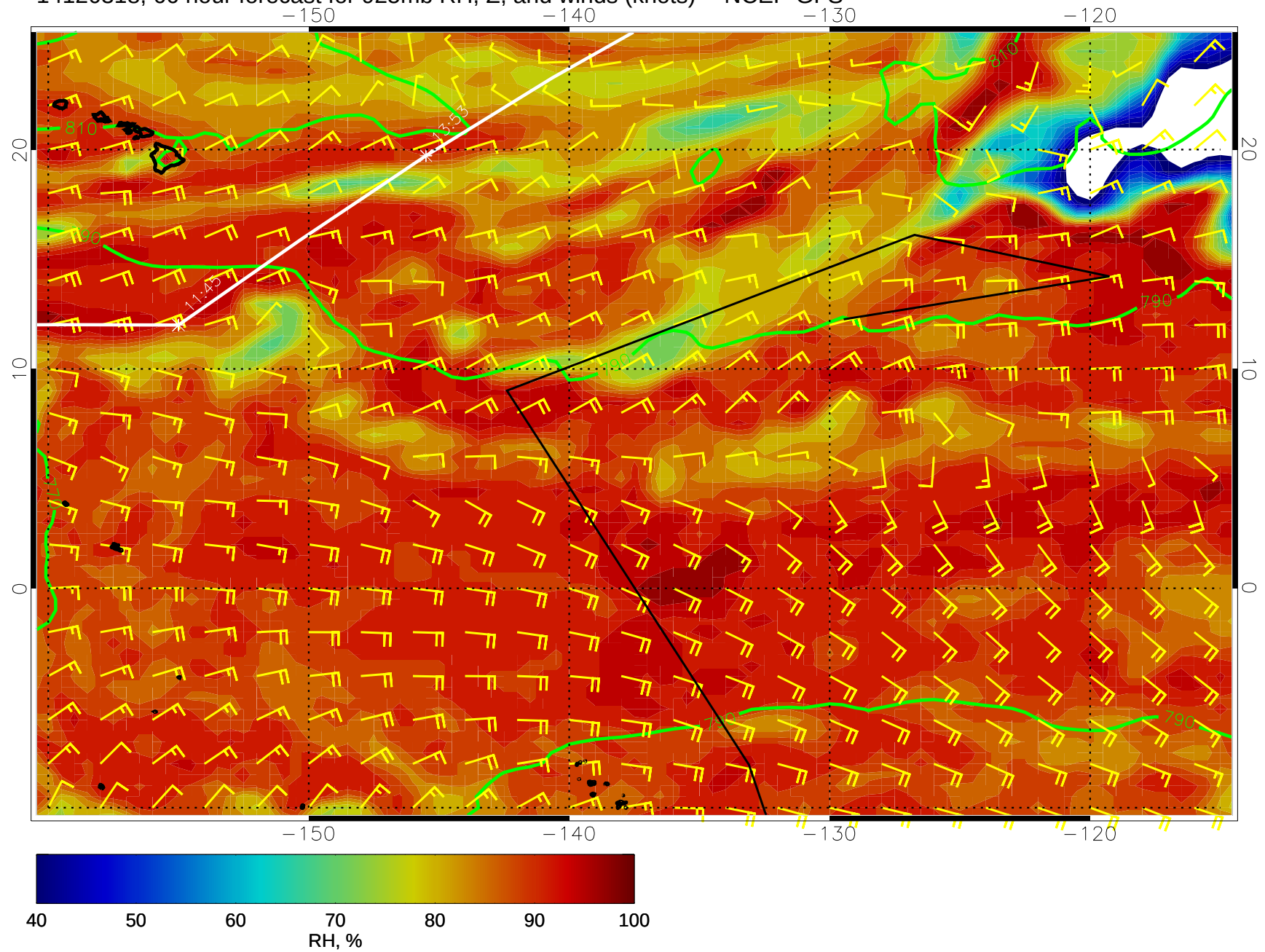
14120318, 66 hour forecast for 925mb RH, Z, and winds (knots) -- NCEP GFS
