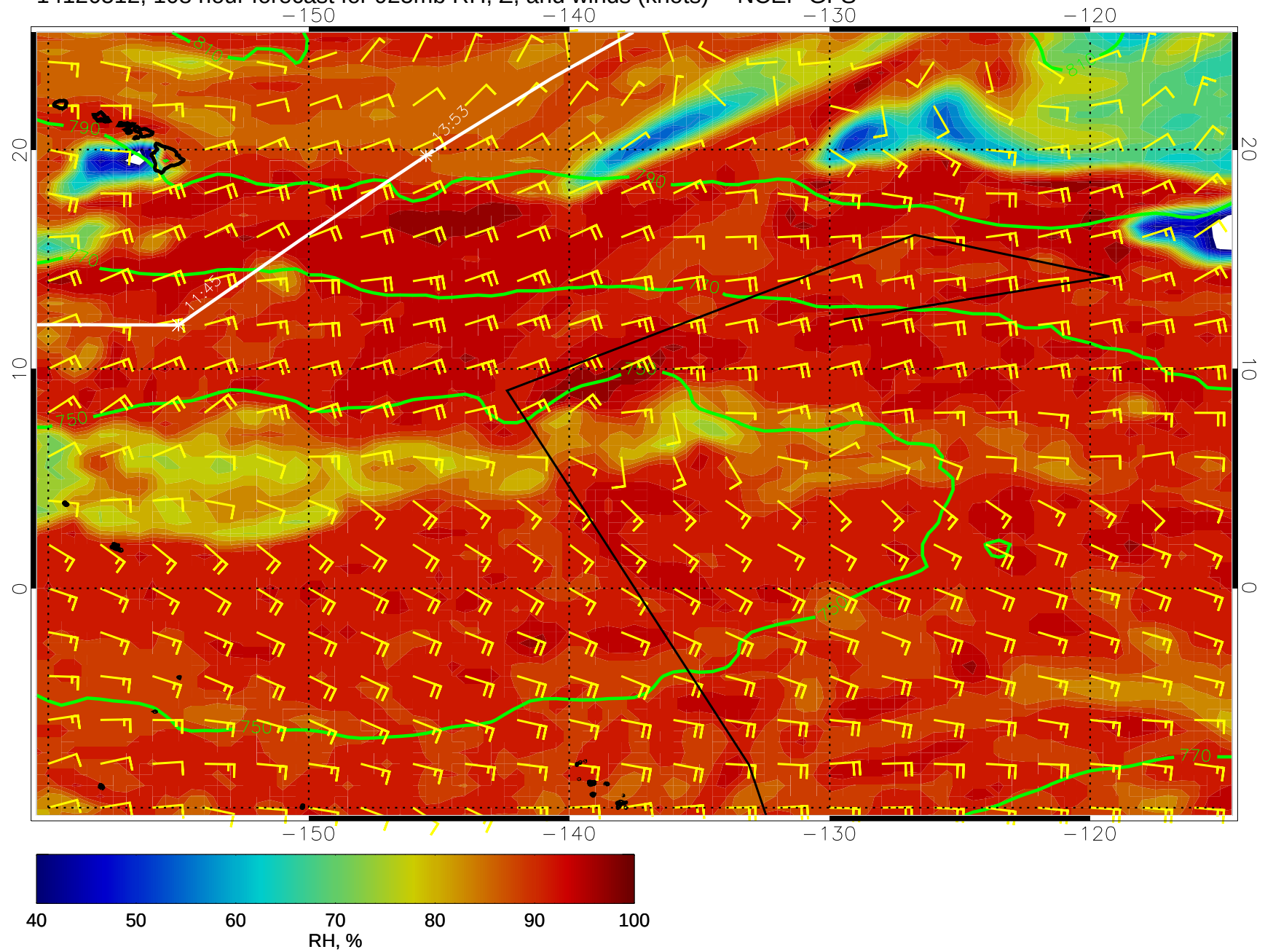
14120512, 108 hour forecast for 925mb RH, Z, and winds (knots) -- NCEP GFS
