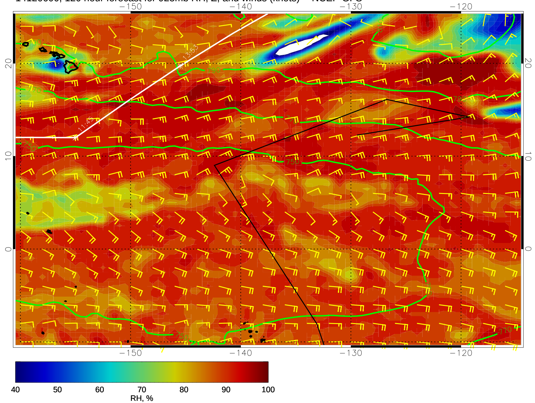
14120600, 120 hour forecast for 925mb RH, Z, and winds (knots) -- NCEP GFS
