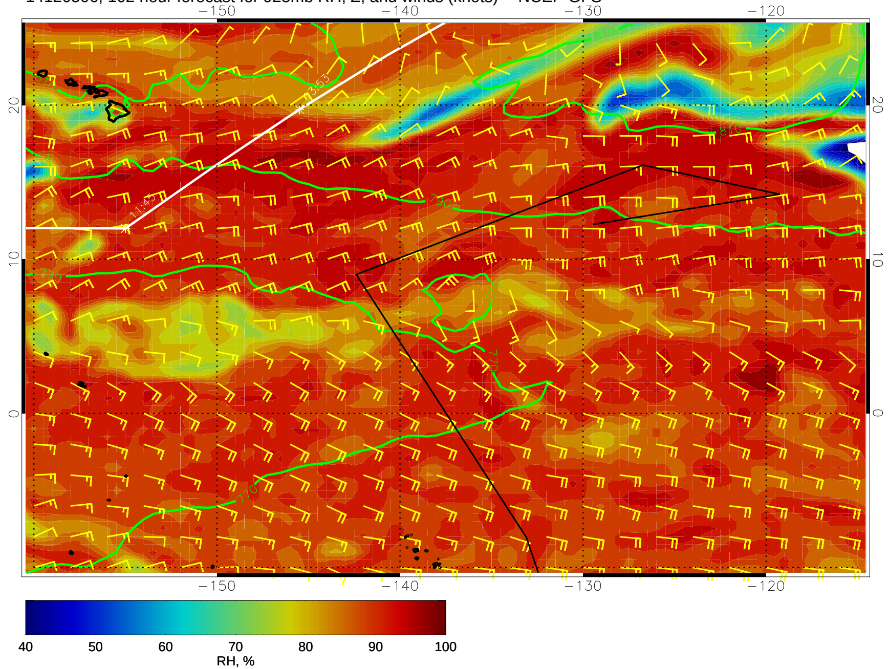
14120506, 102 hour forecast for 925mb RH, Z, and winds (knots) -- NCEP GFS
