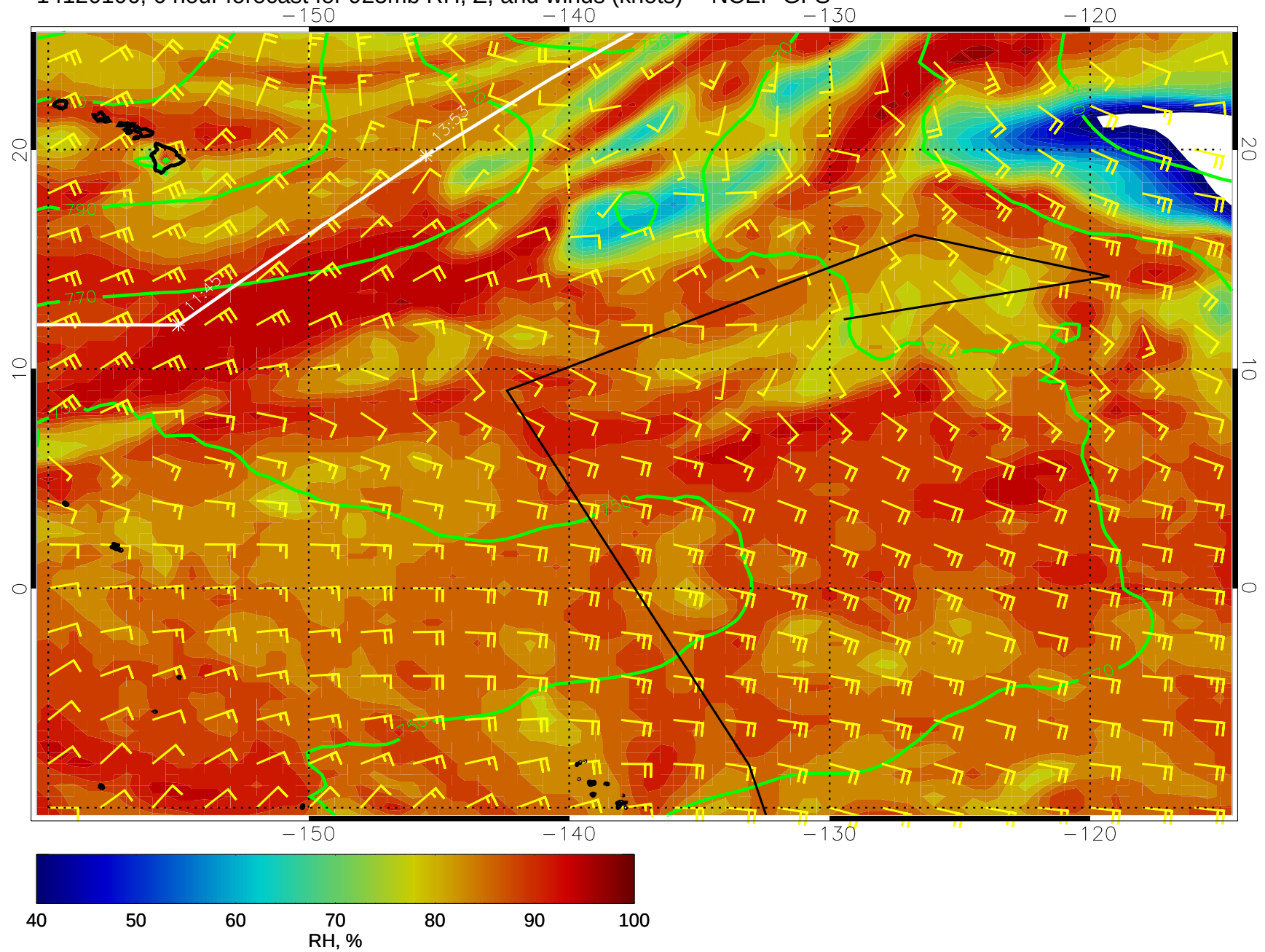
14120106, 6 hour forecast for 925mb RH, Z, and winds (knots) -- NCEP GFS
