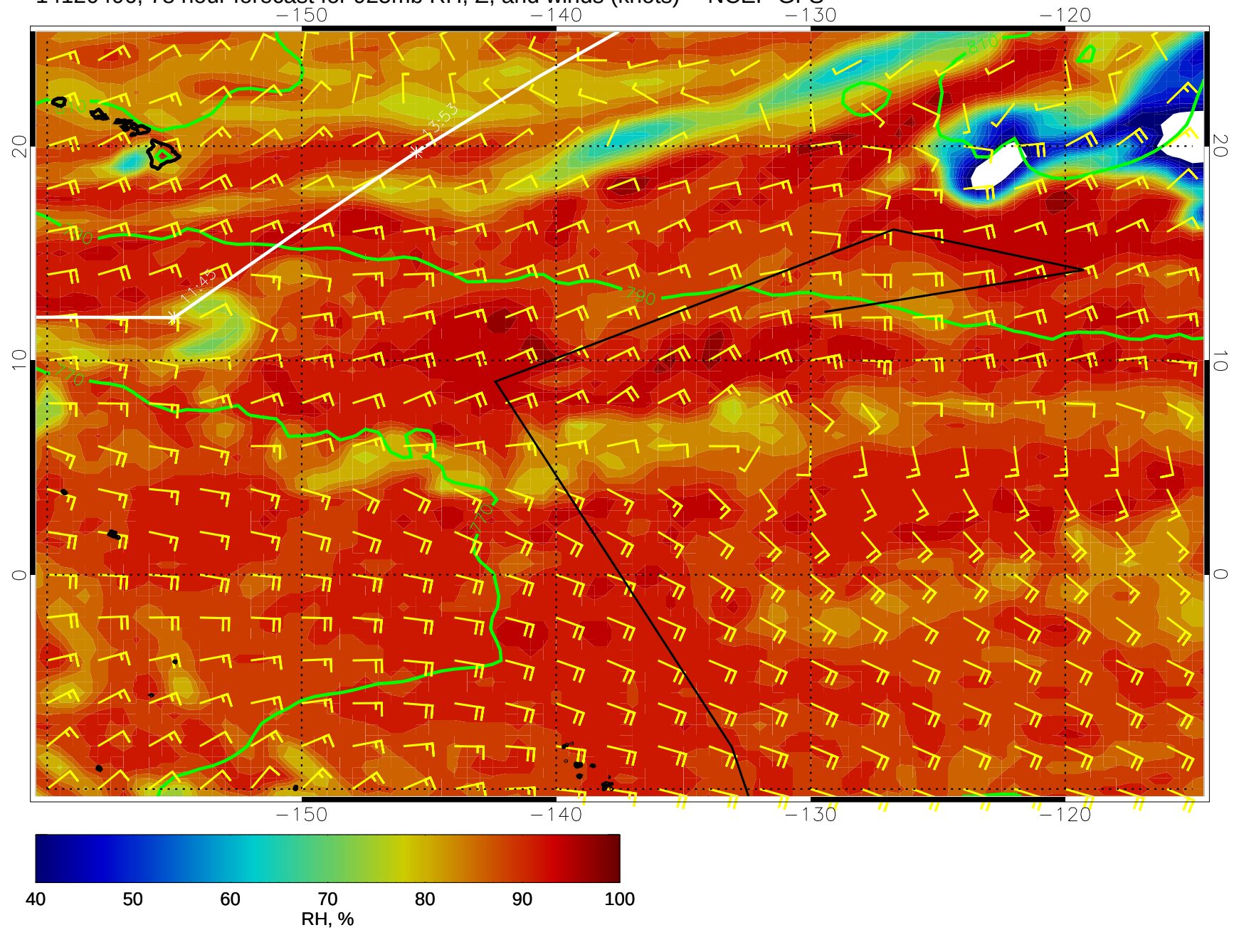
14120406, 78 hour forecast for 925mb RH, Z, and winds (knots) -- NCEP GFS
