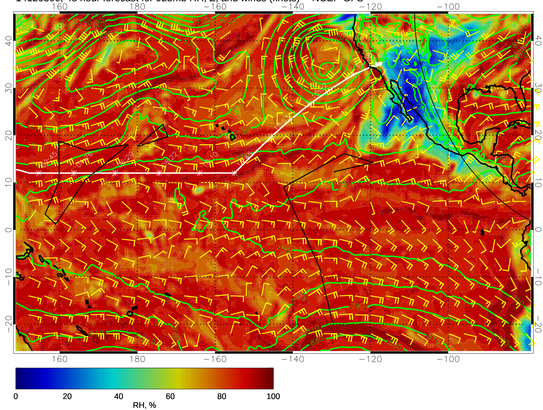
14120300, 48 hour forecast for 925mb RH, Z, and winds (knots) -- NCEP GFS
