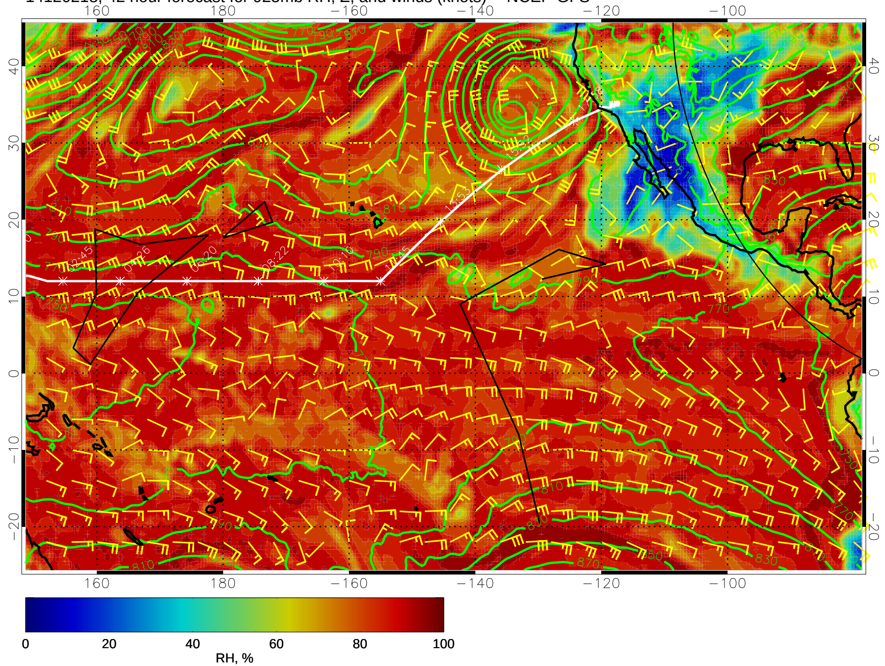
14120218, 42 hour forecast for 925mb RH, Z, and winds (knots) -- NCEP GFS
