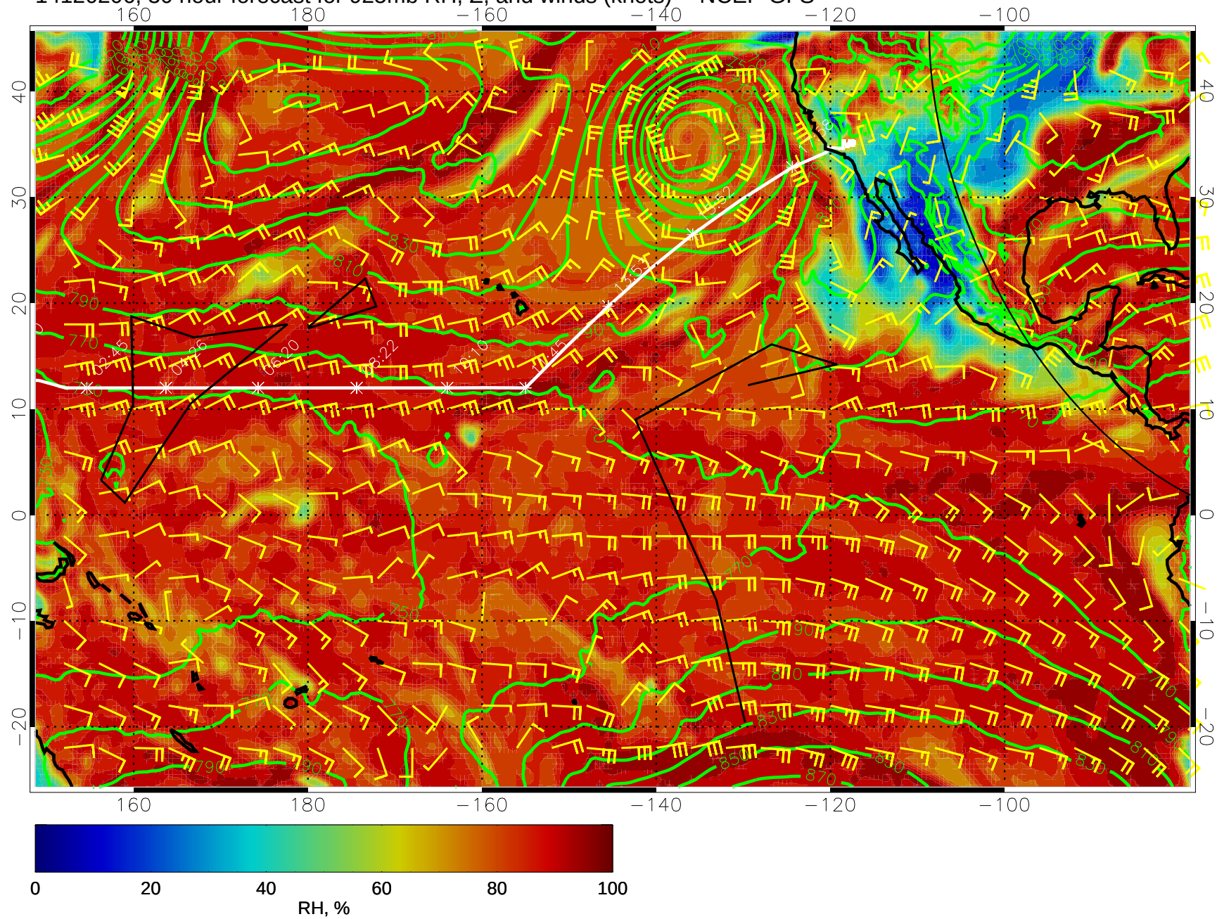
14120206, 30 hour forecast for 925mb RH, Z, and winds (knots) -- NCEP GFS
