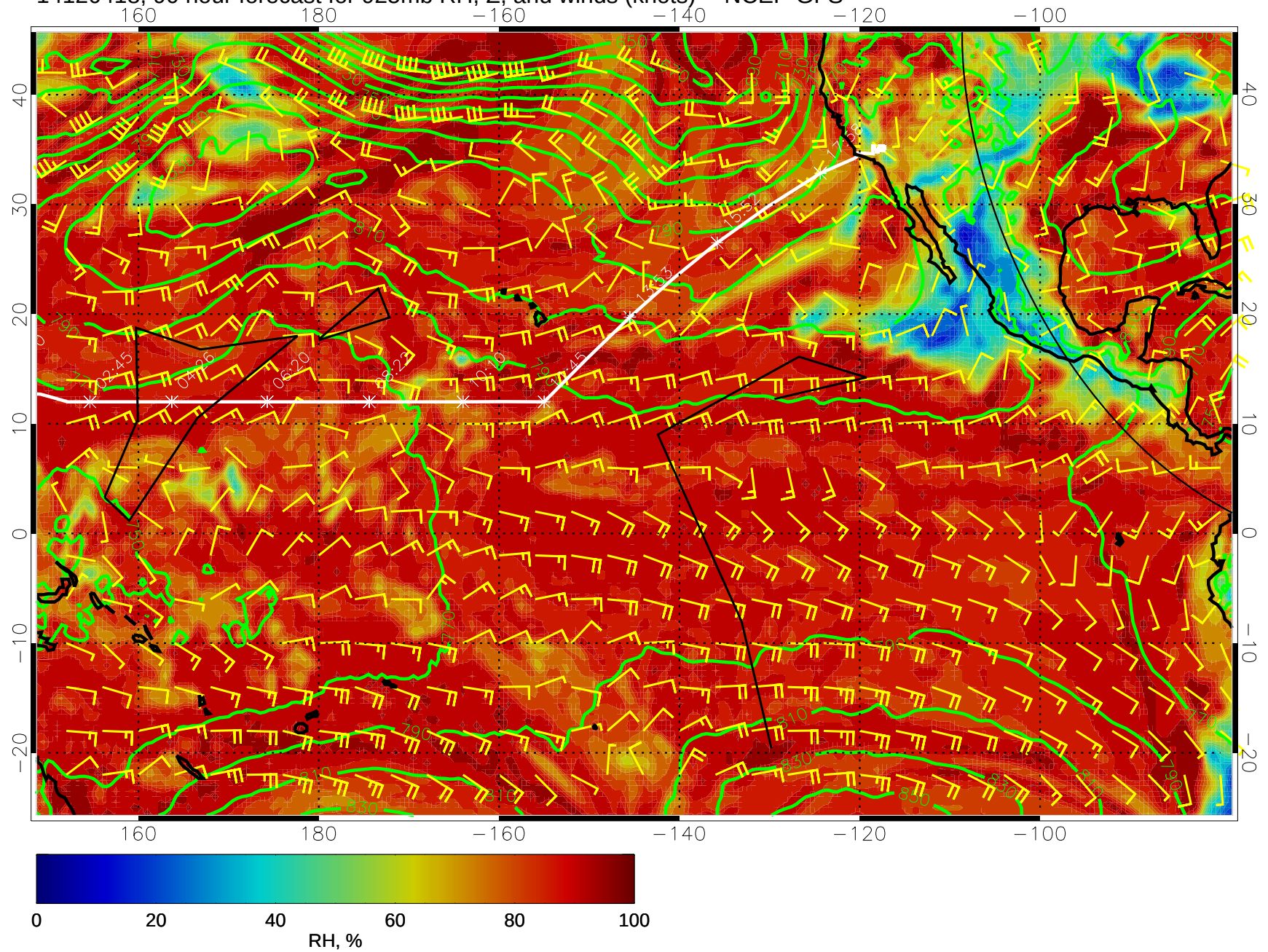
14120418, 90 hour forecast for 925mb RH, Z, and winds (knots) -- NCEP GFS
