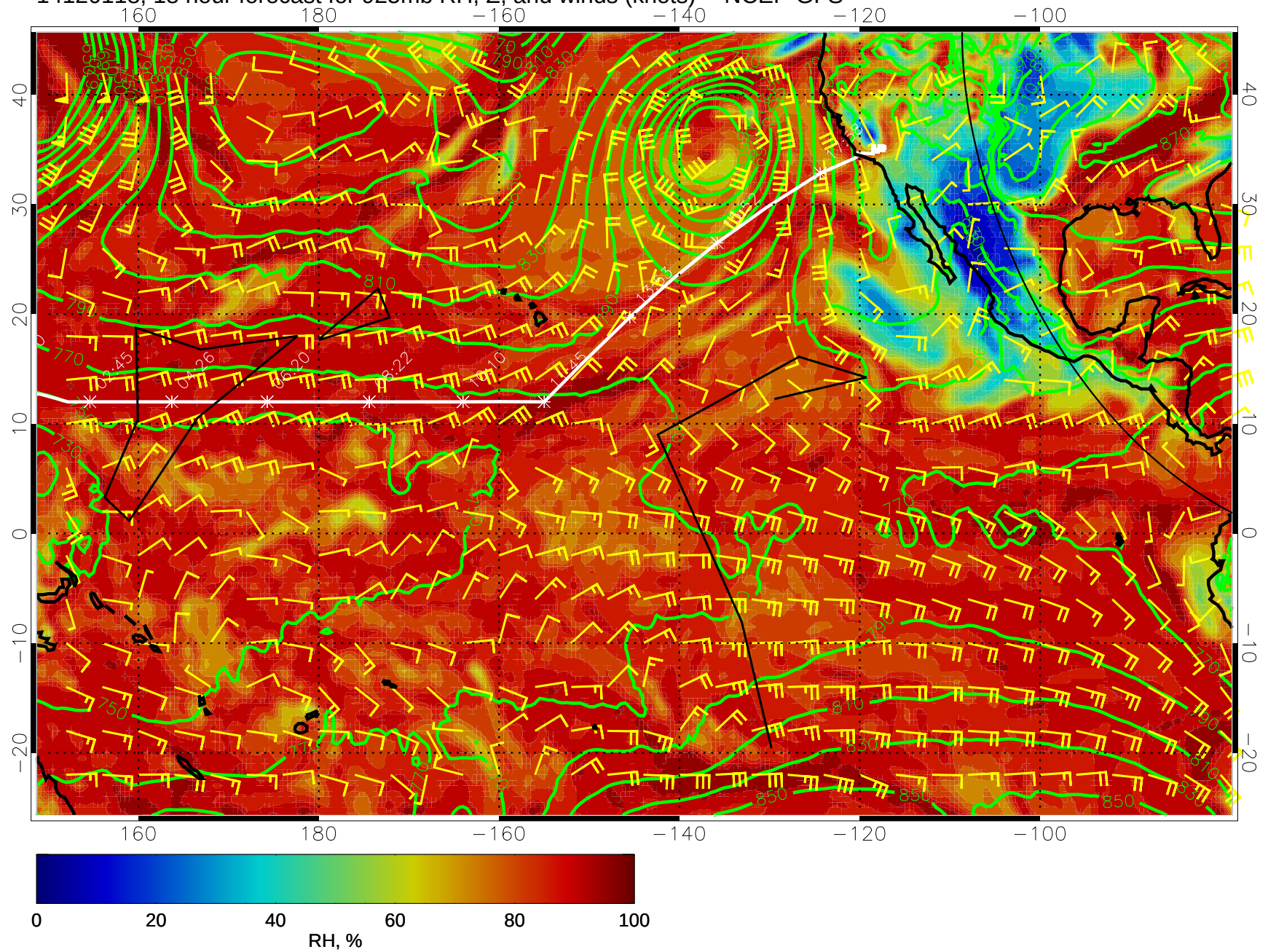
14120118, 18 hour forecast for 925mb RH, Z, and winds (knots) -- NCEP GFS
