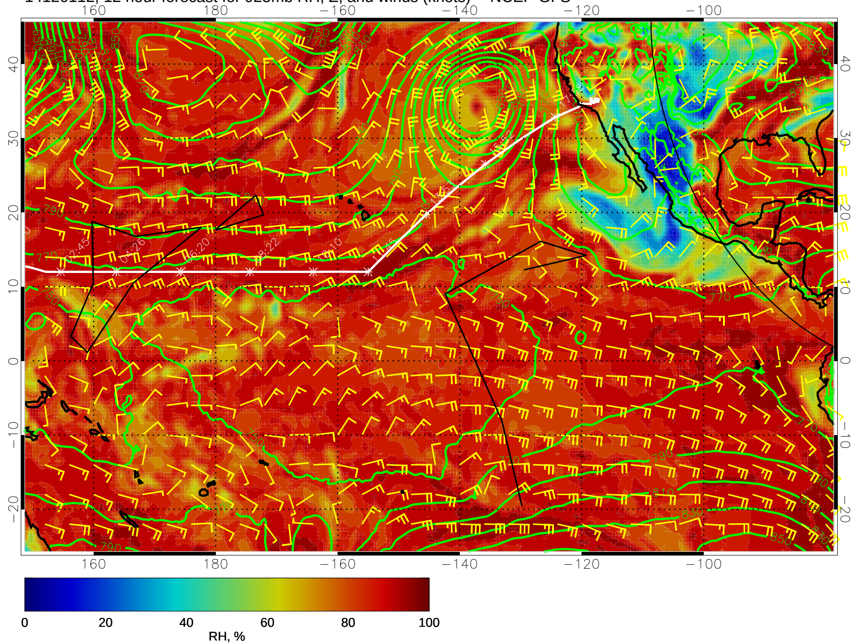
14120112, 12 hour forecast for 925mb RH, Z, and winds (knots) -- NCEP GFS
