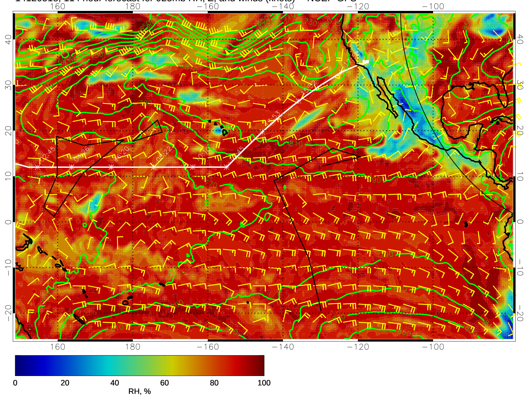
14120518, 114 hour forecast for 925mb RH, Z, and winds (knots) -- NCEP GFS
