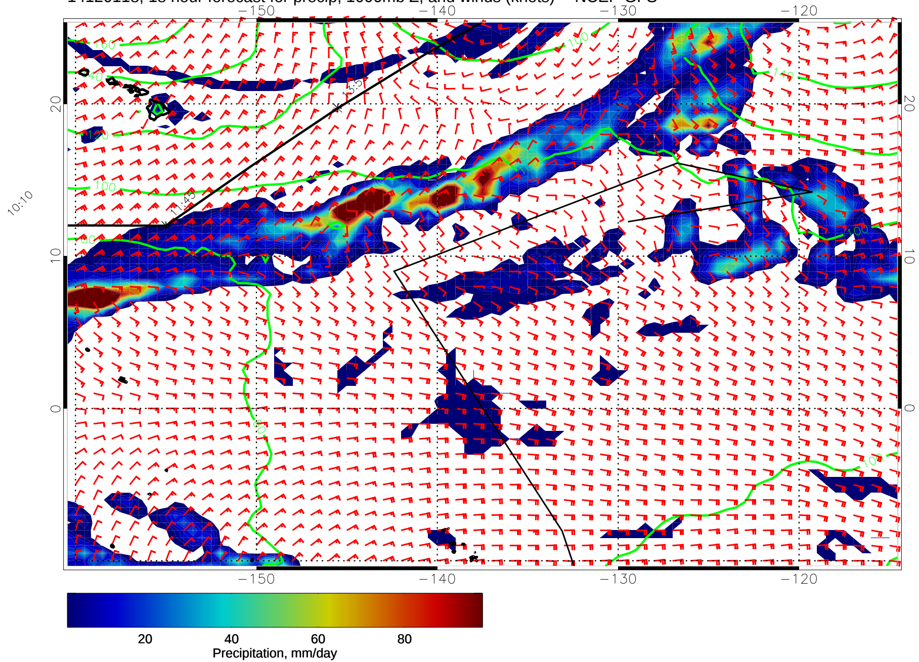
14120118, 18 hour forecast for precip, 1000mb Z, and winds (knots) -- NCEP GFS
