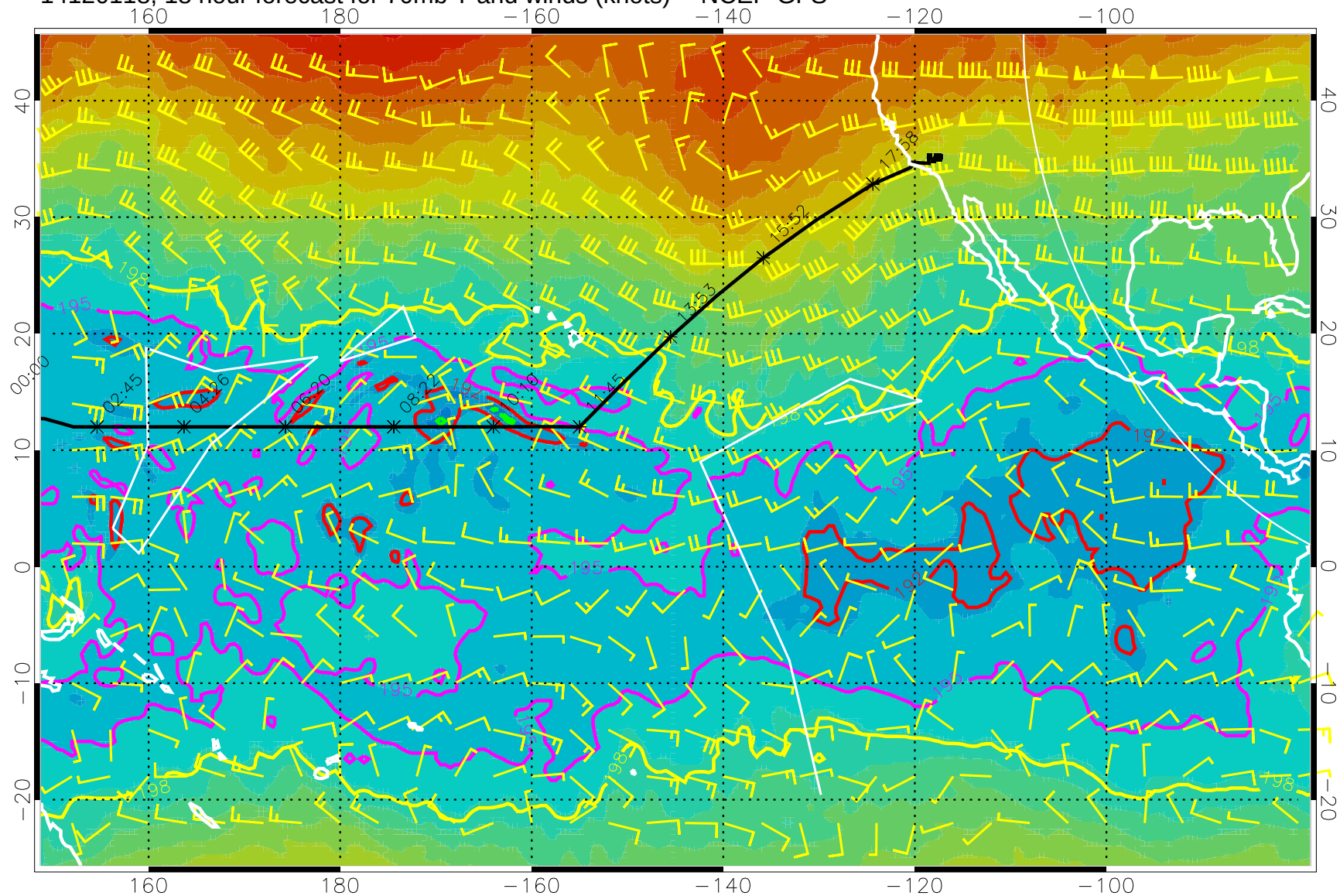
14120118, 18 hour forecast for 70mb T and winds (knots) -- NCEP GFS
