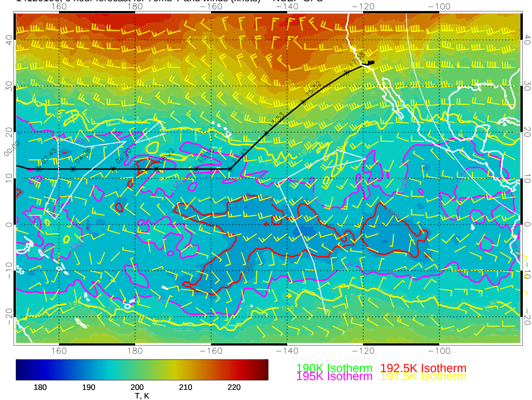
14120106, 6 hour forecast for 70mb T and winds (knots) -- NCEP GFS
