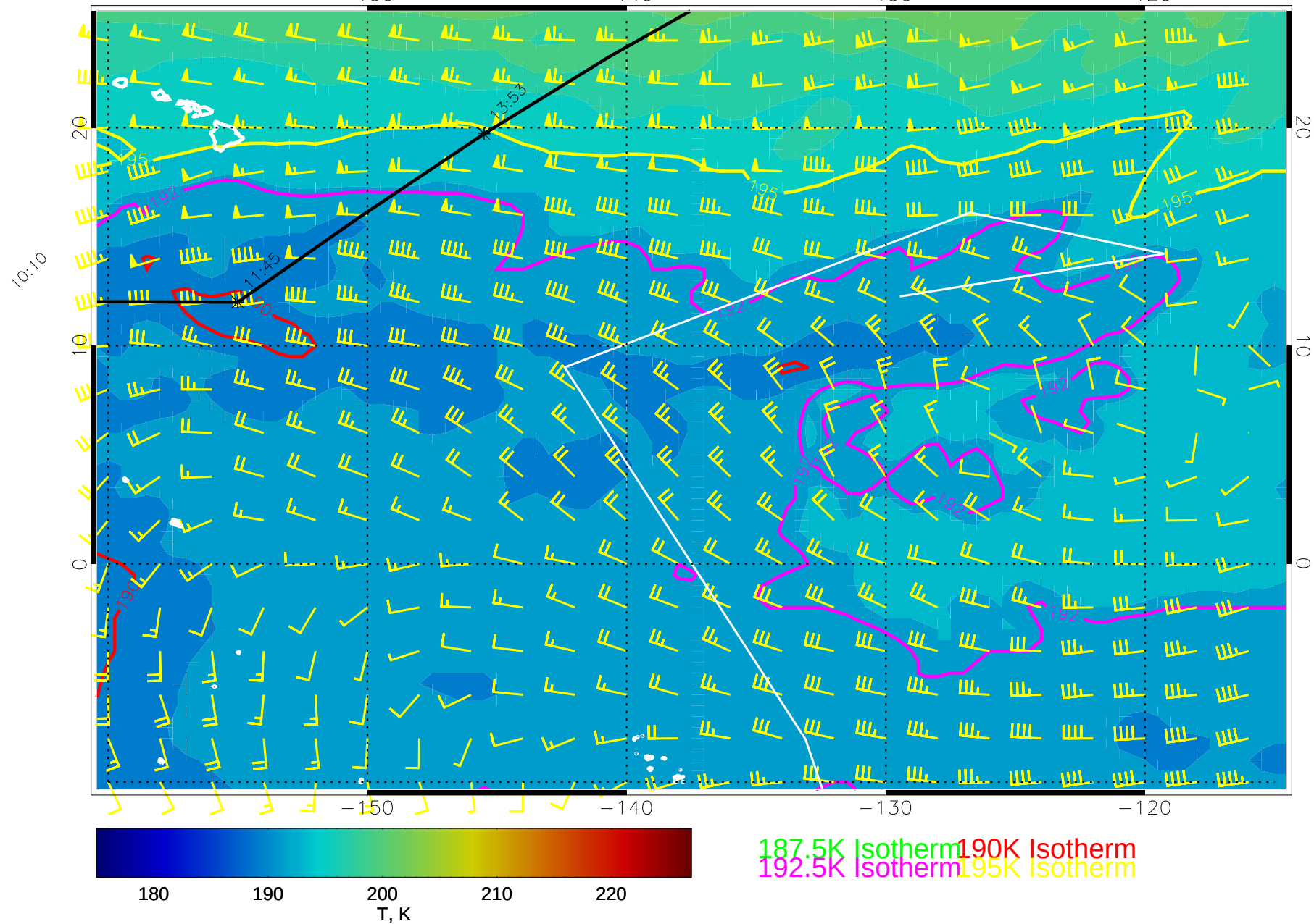
14120412, 84 hour forecast for 100mb T and winds (knots) -- NCEP GFS
