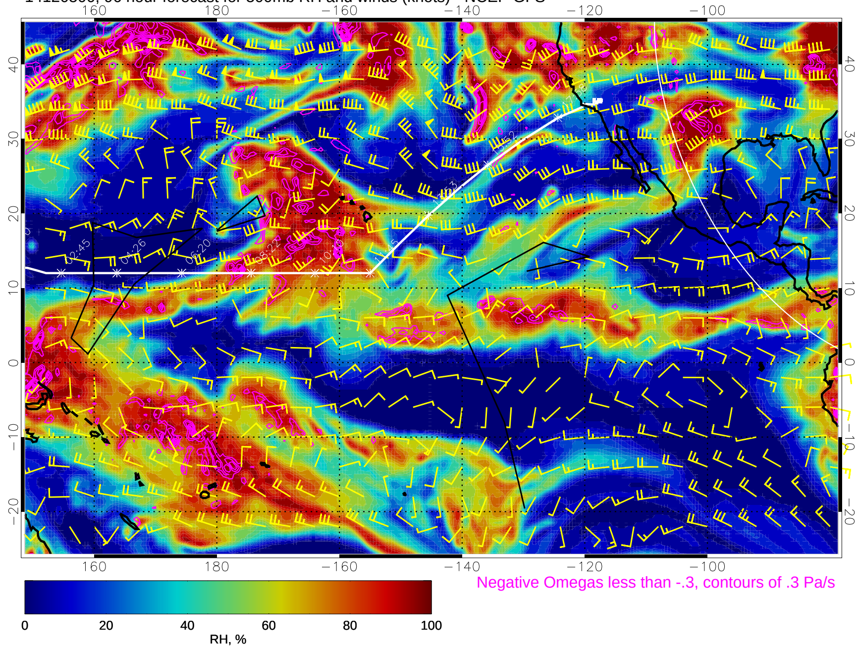
14120500, 96 hour forecast for 500mb RH and winds (knots) - NCEP GFS
