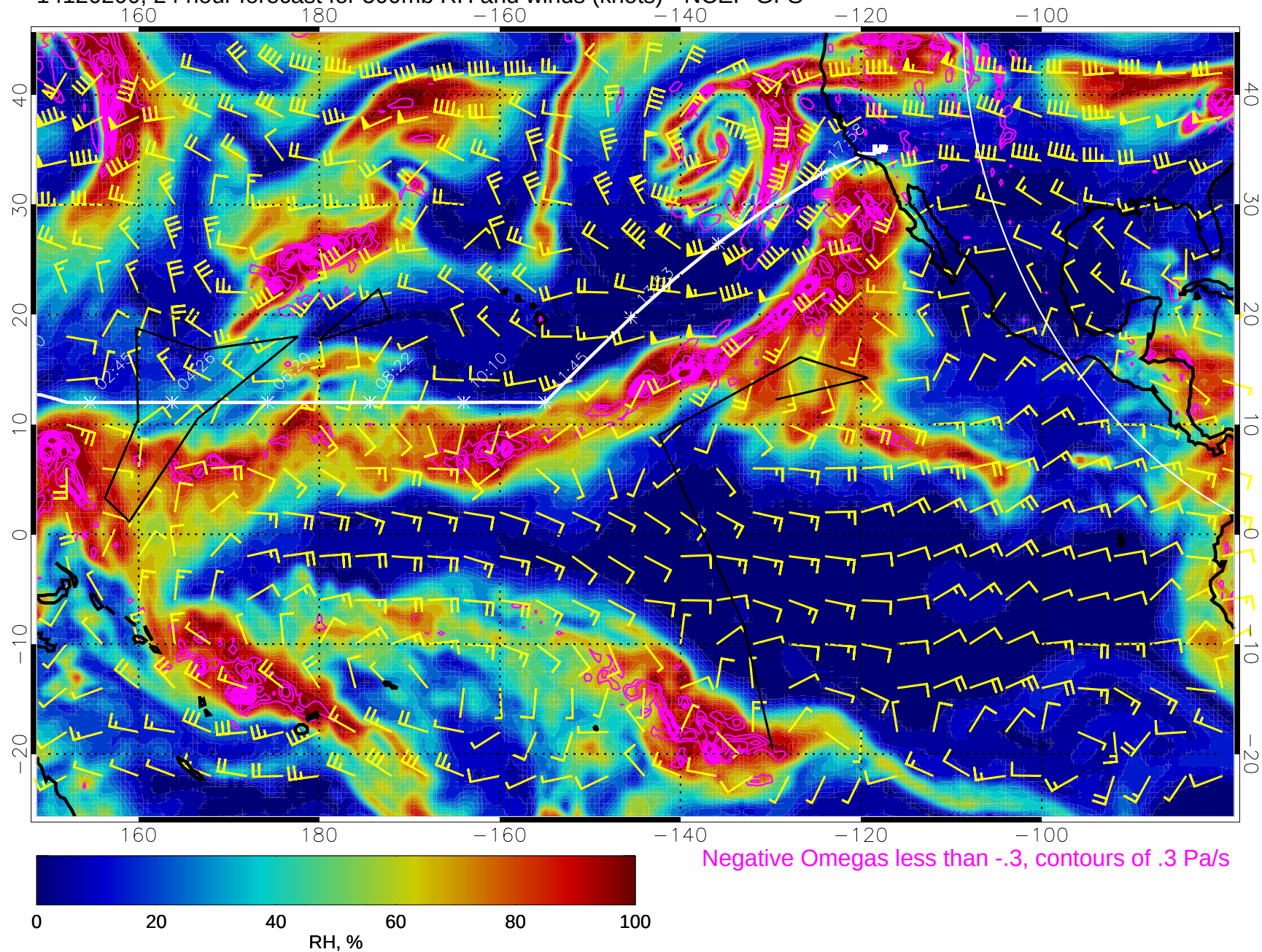
14120200, 24 hour forecast for 500mb RH and winds (knots) - NCEP GFS
