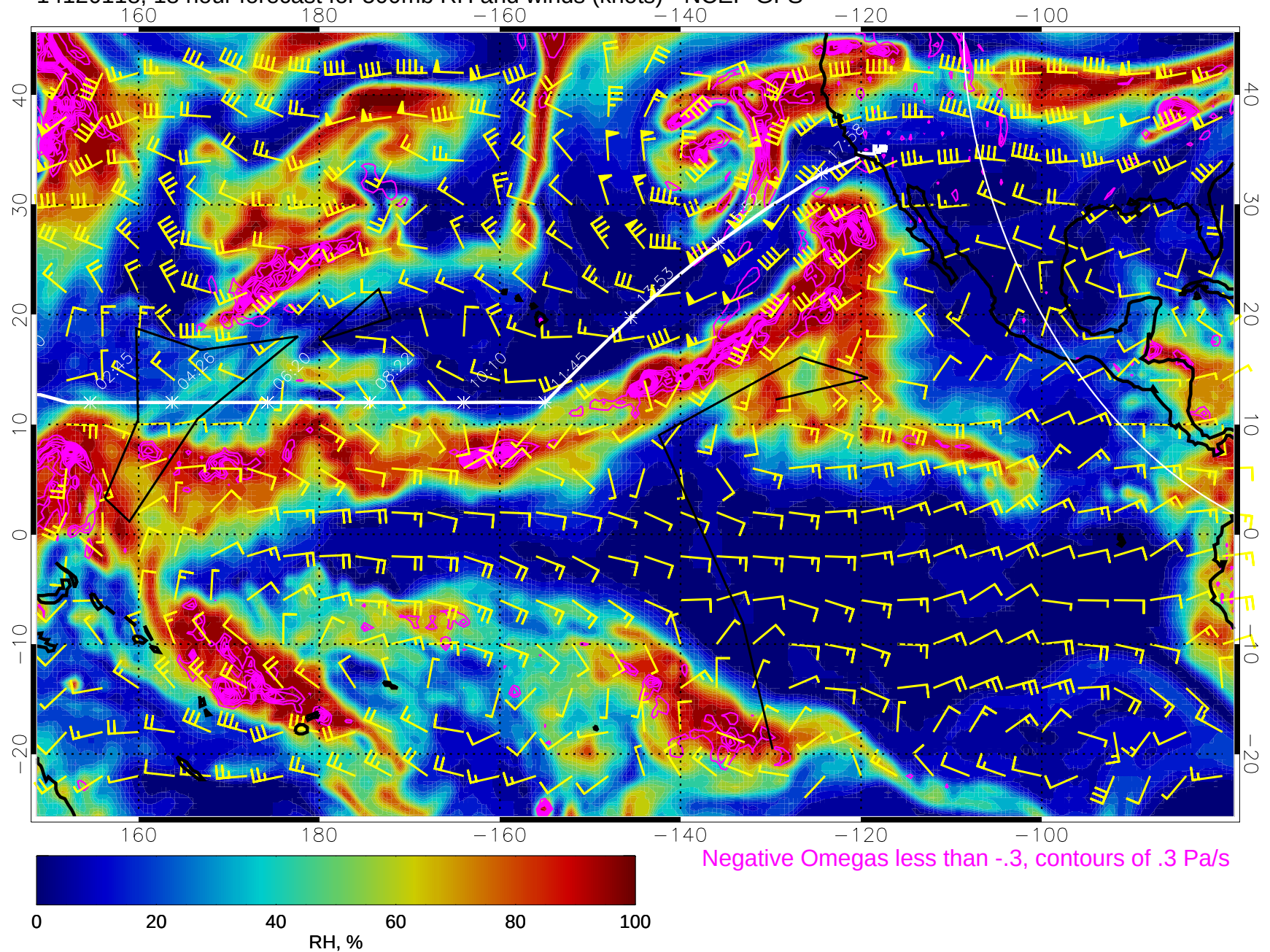
14120118, 18 hour forecast for 500mb RH and winds (knots) - NCEP GFS
