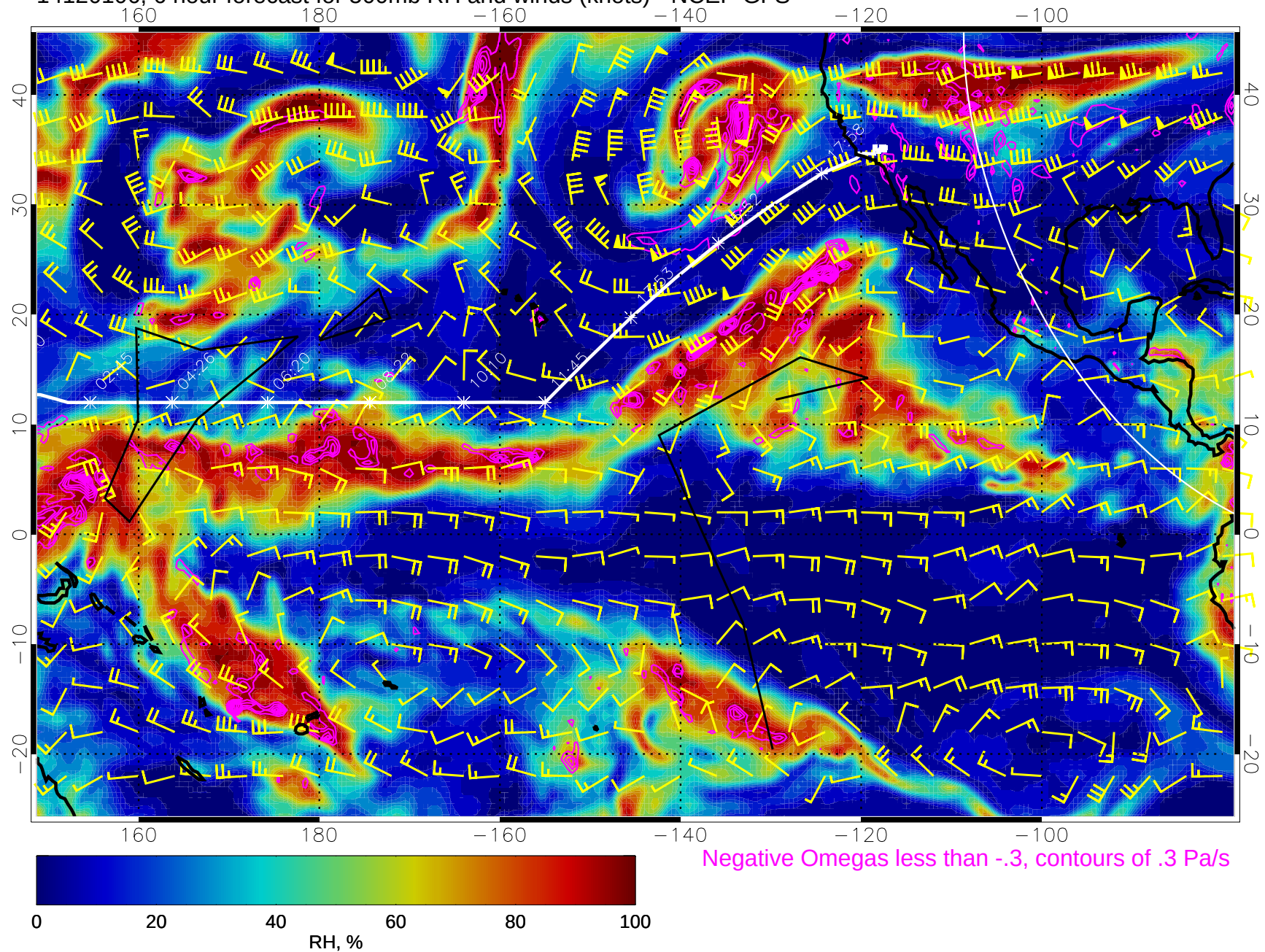
14120106, 6 hour forecast for 500mb RH and winds (knots) - NCEP GFS
