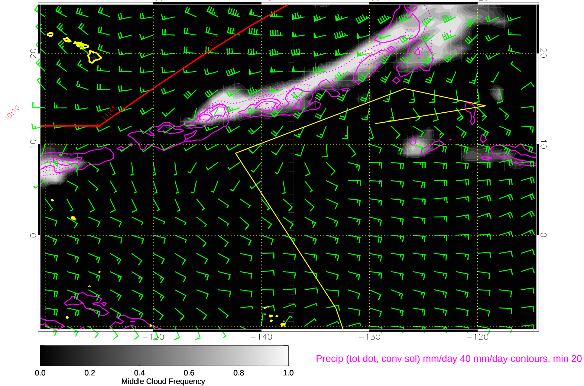
14120200, 24 hour forecast for 500mb winds (knots) and Middle Cloud Frequency -- NCEP GFS
