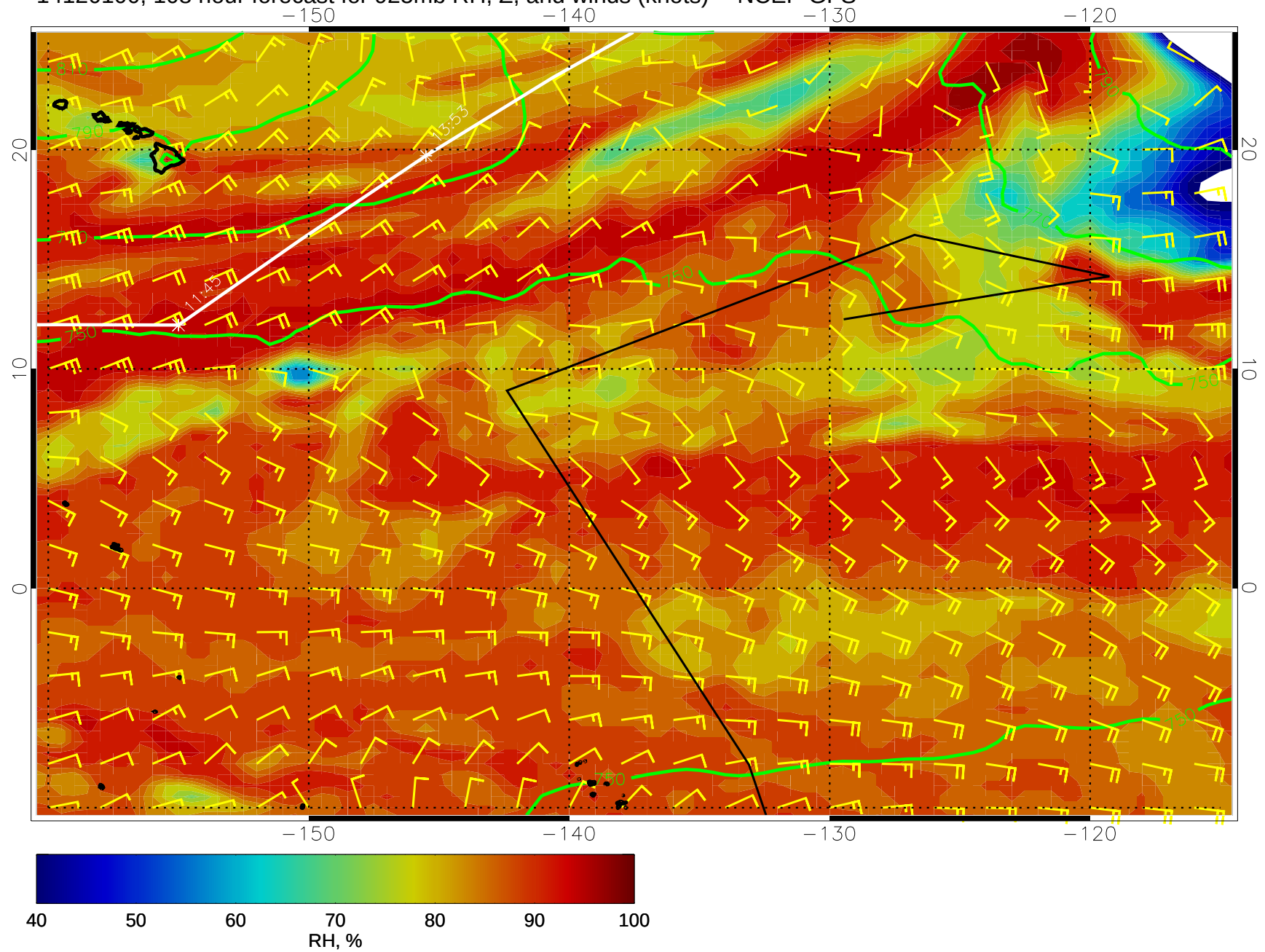
14120100, 108 hour forecast for 925mb RH, Z, and winds (knots) -- NCEP GFS
