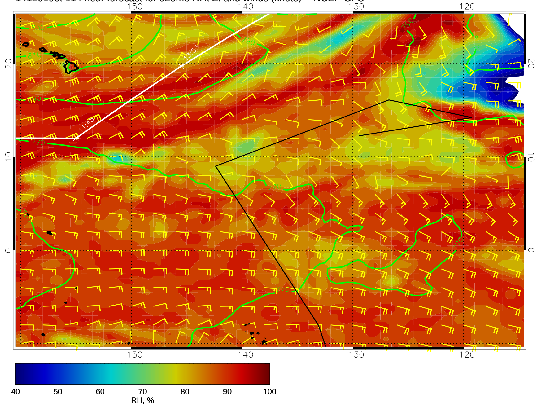
14120106, 114 hour forecast for 925mb RH, Z, and winds (knots) -- NCEP GFS
