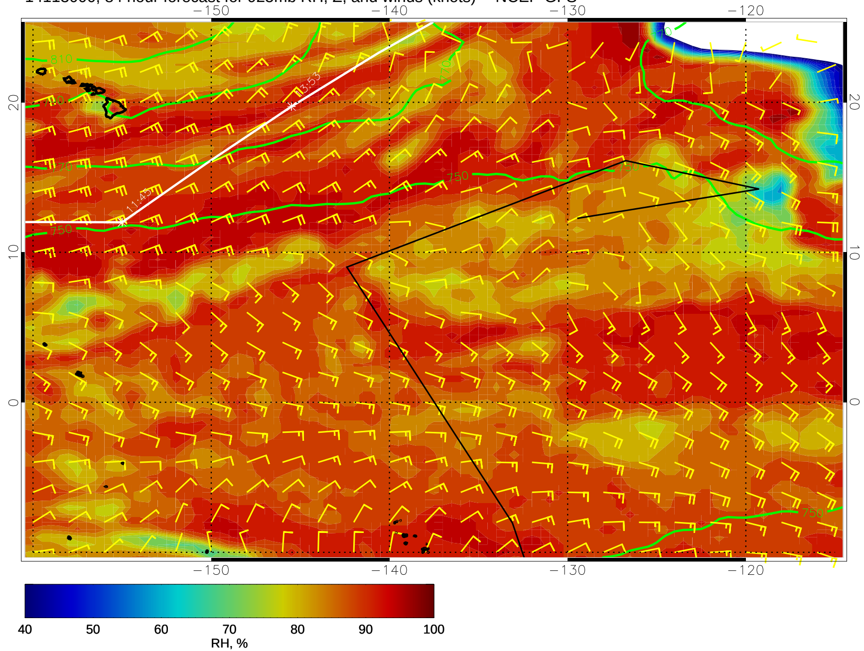
14113000, 84 hour forecast for 925mb RH, Z, and winds (knots) -- NCEP GFS
