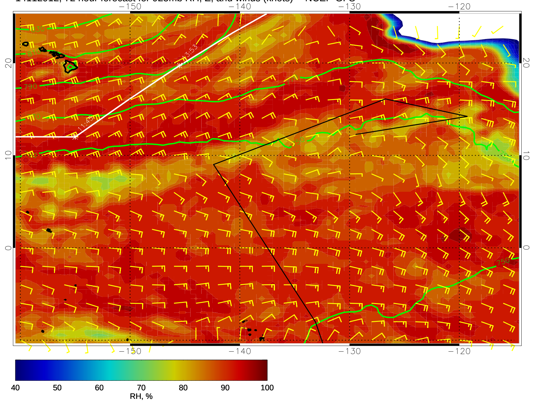
14112912, 72 hour forecast for 925mb RH, Z, and winds (knots) -- NCEP GFS
