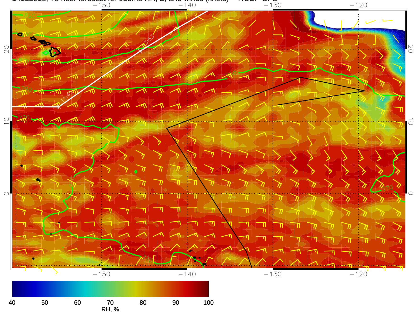
14112918, 78 hour forecast for 925mb RH, Z, and winds (knots) -- NCEP GFS
