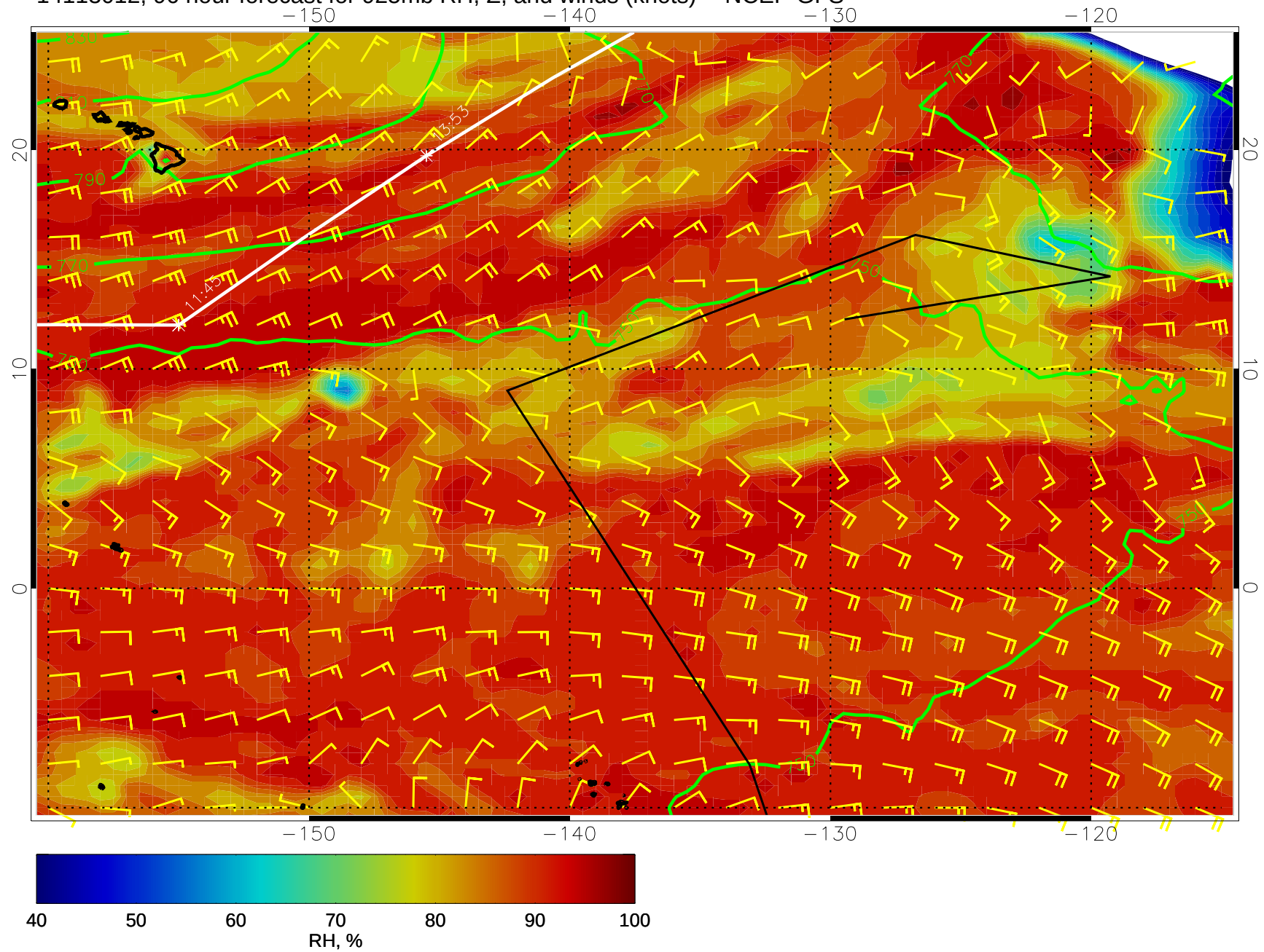
14113012, 96 hour forecast for 925mb RH, Z, and winds (knots) -- NCEP GFS
