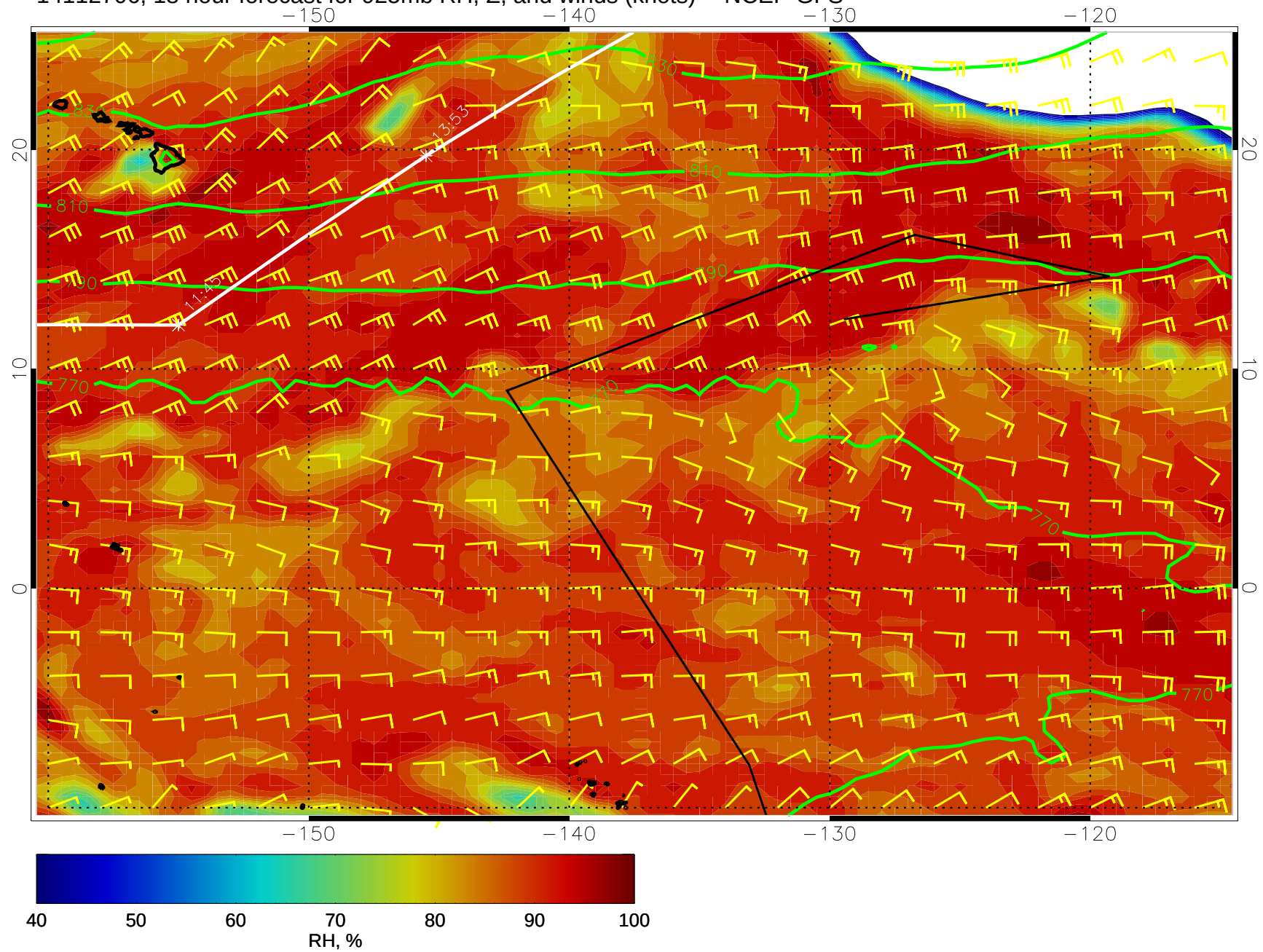
14112706, 18 hour forecast for 925mb RH, Z, and winds (knots) -- NCEP GFS
