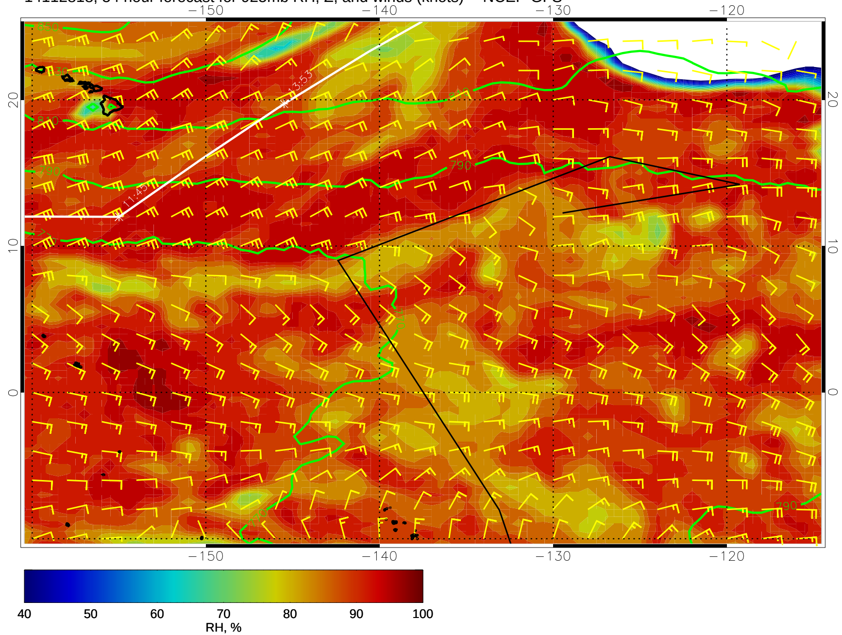
14112818, 54 hour forecast for 925mb RH, Z, and winds (knots) -- NCEP GFS
