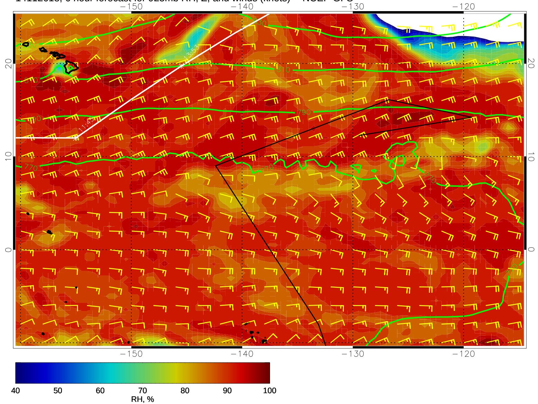
14112618, 6 hour forecast for 925mb RH, Z, and winds (knots) -- NCEP GFS
