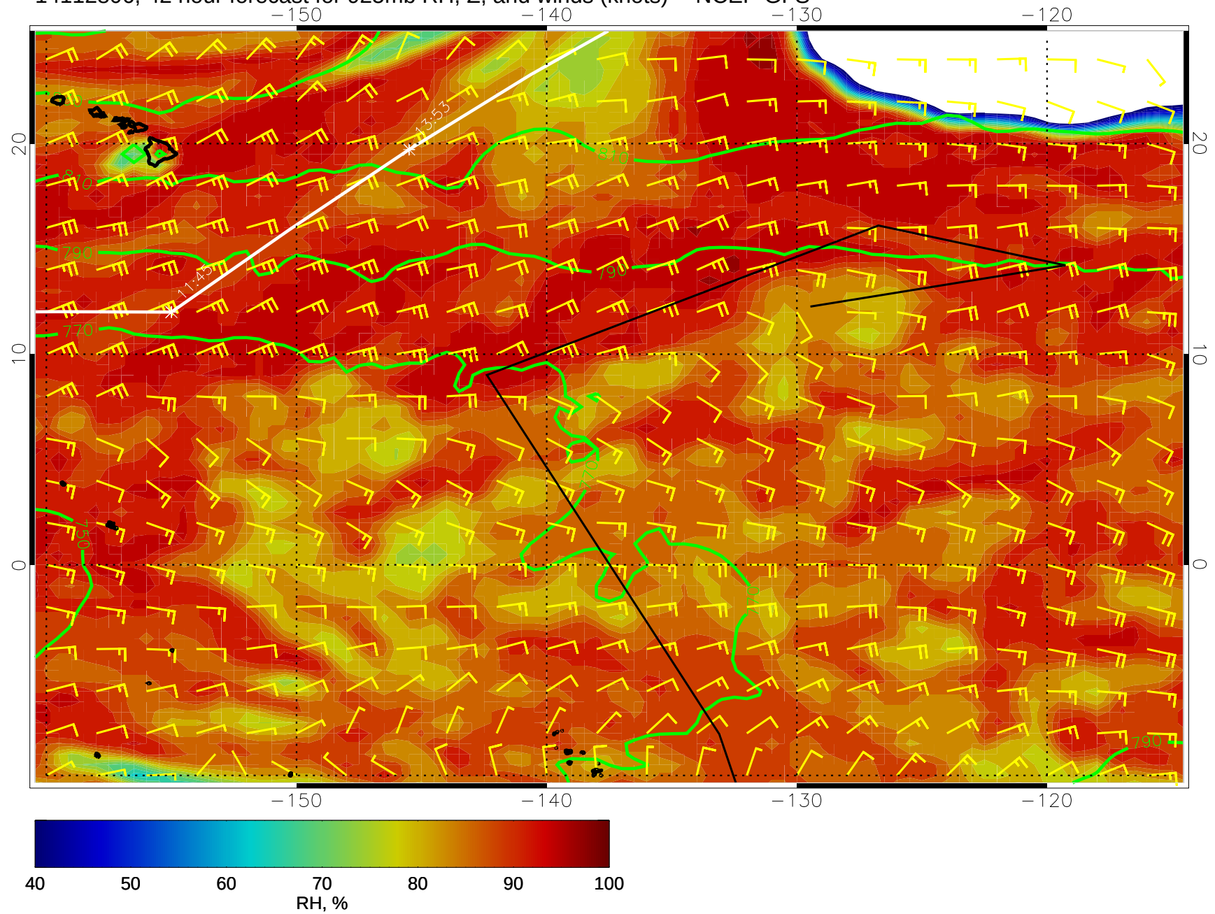
14112806, 42 hour forecast for 925mb RH, Z, and winds (knots) -- NCEP GFS
