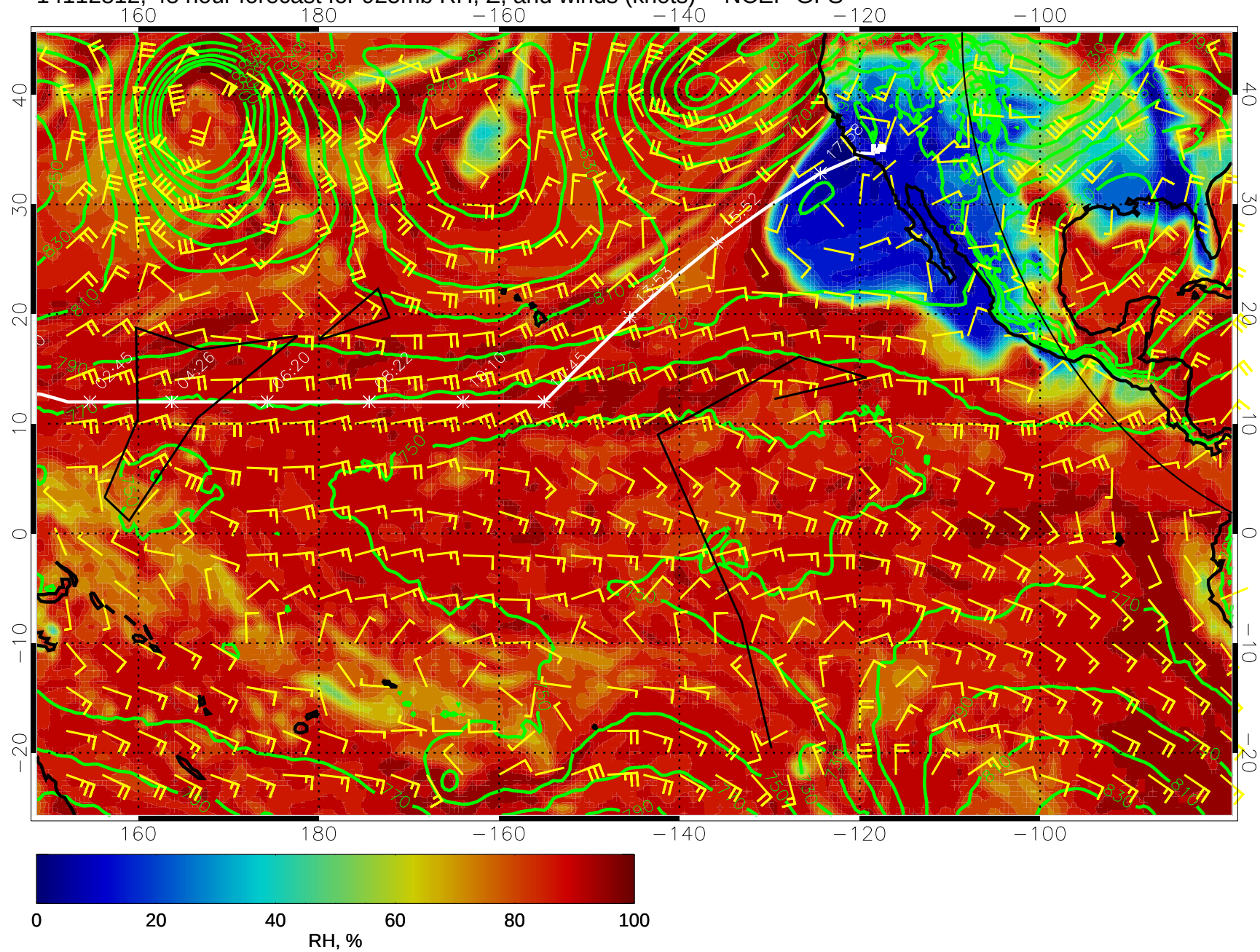
14112812, 48 hour forecast for 925mb RH, Z, and winds (knots) -- NCEP GFS
