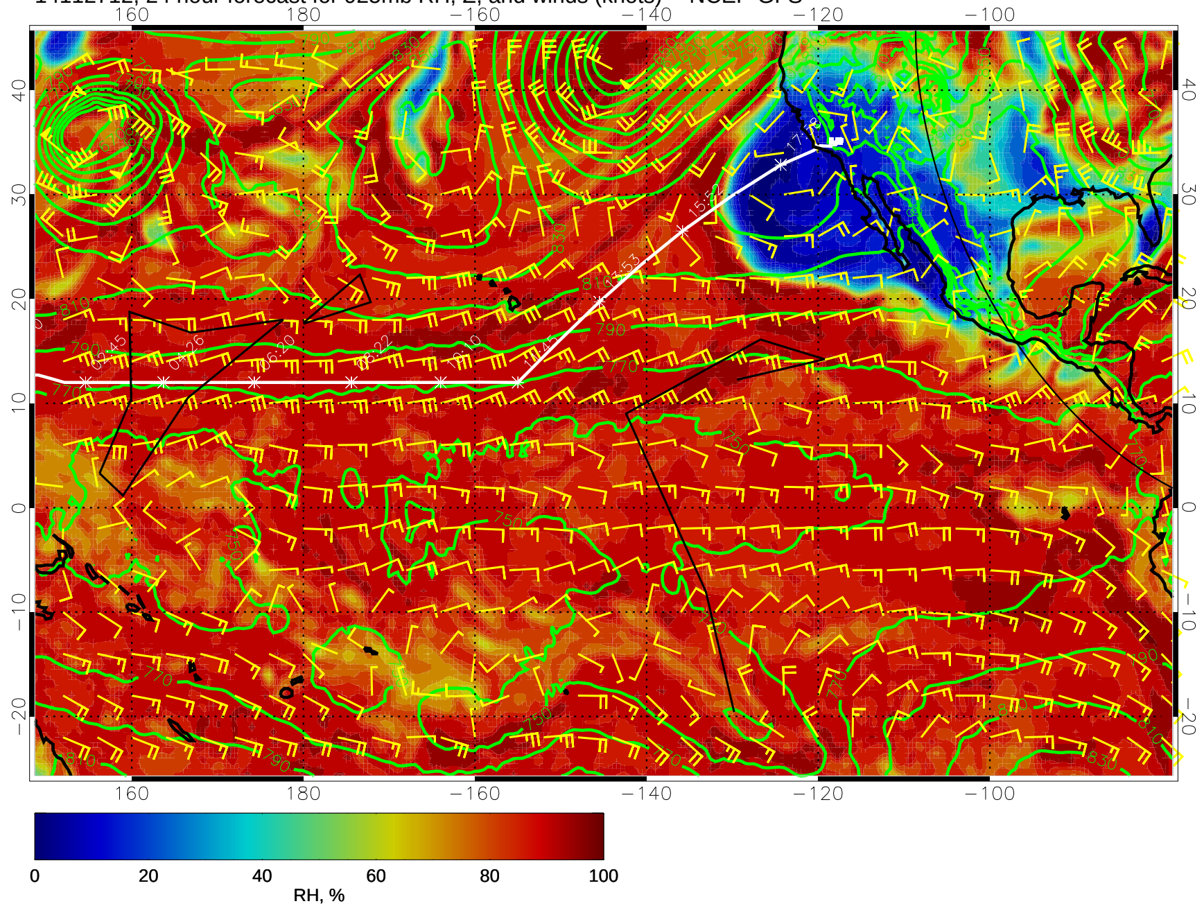
14112712, 24 hour forecast for 925mb RH, Z, and winds (knots) -- NCEP GFS
