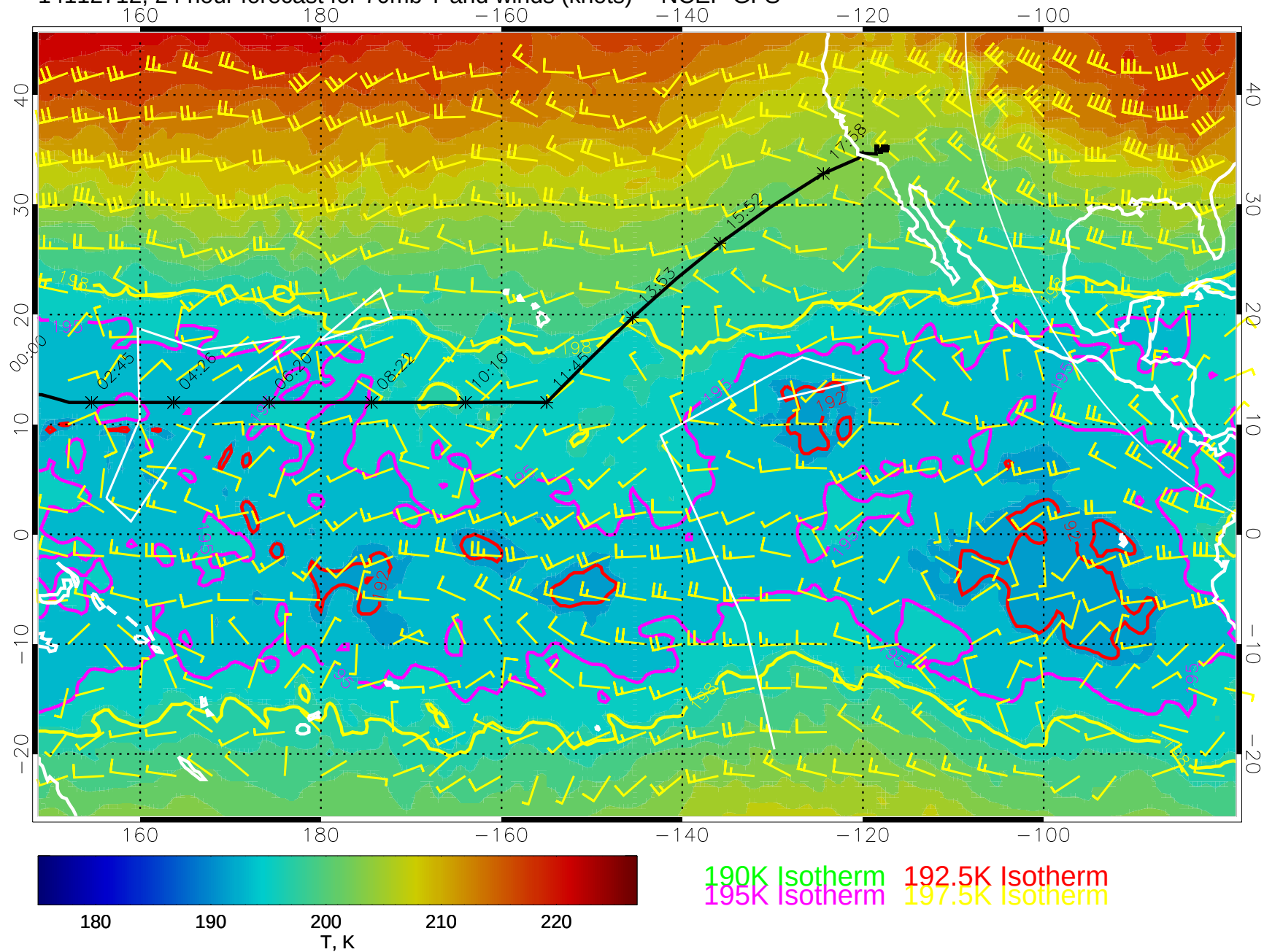
14112712, 24 hour forecast for 70mb T and winds (knots) -- NCEP GFS
