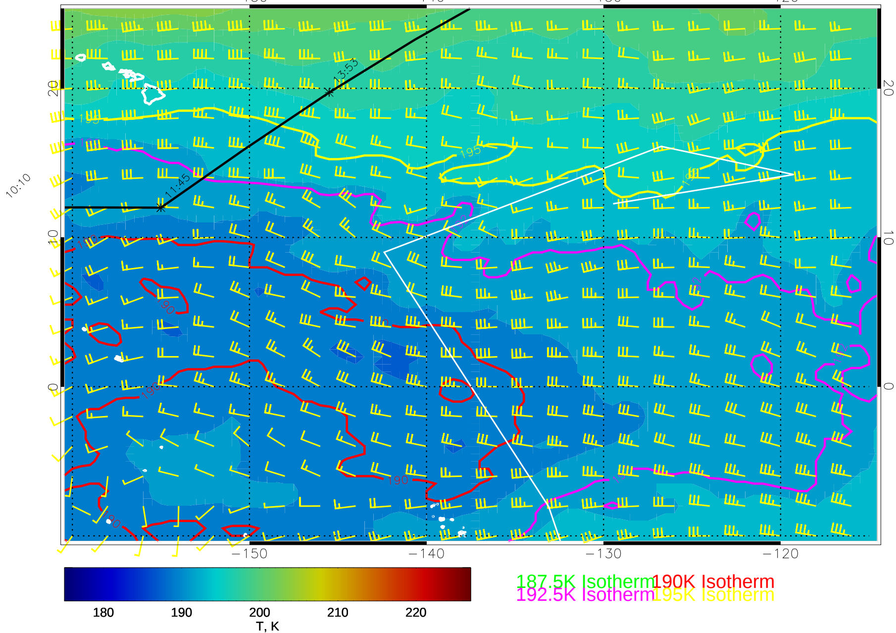
14112818, 54 hour forecast for 100mb T and winds (knots) -- NCEP GFS
