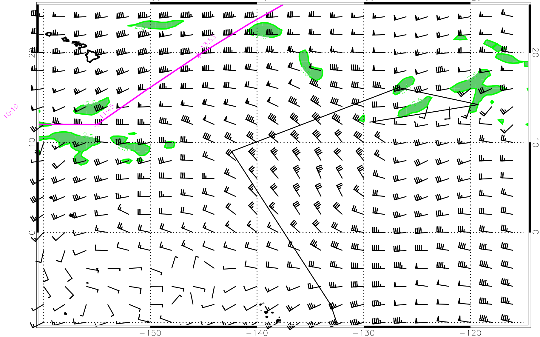
14112912, 72 hour forecast for 45Kft Knapp_Ellrod TI and winds (knots) -- NCEP GFS
