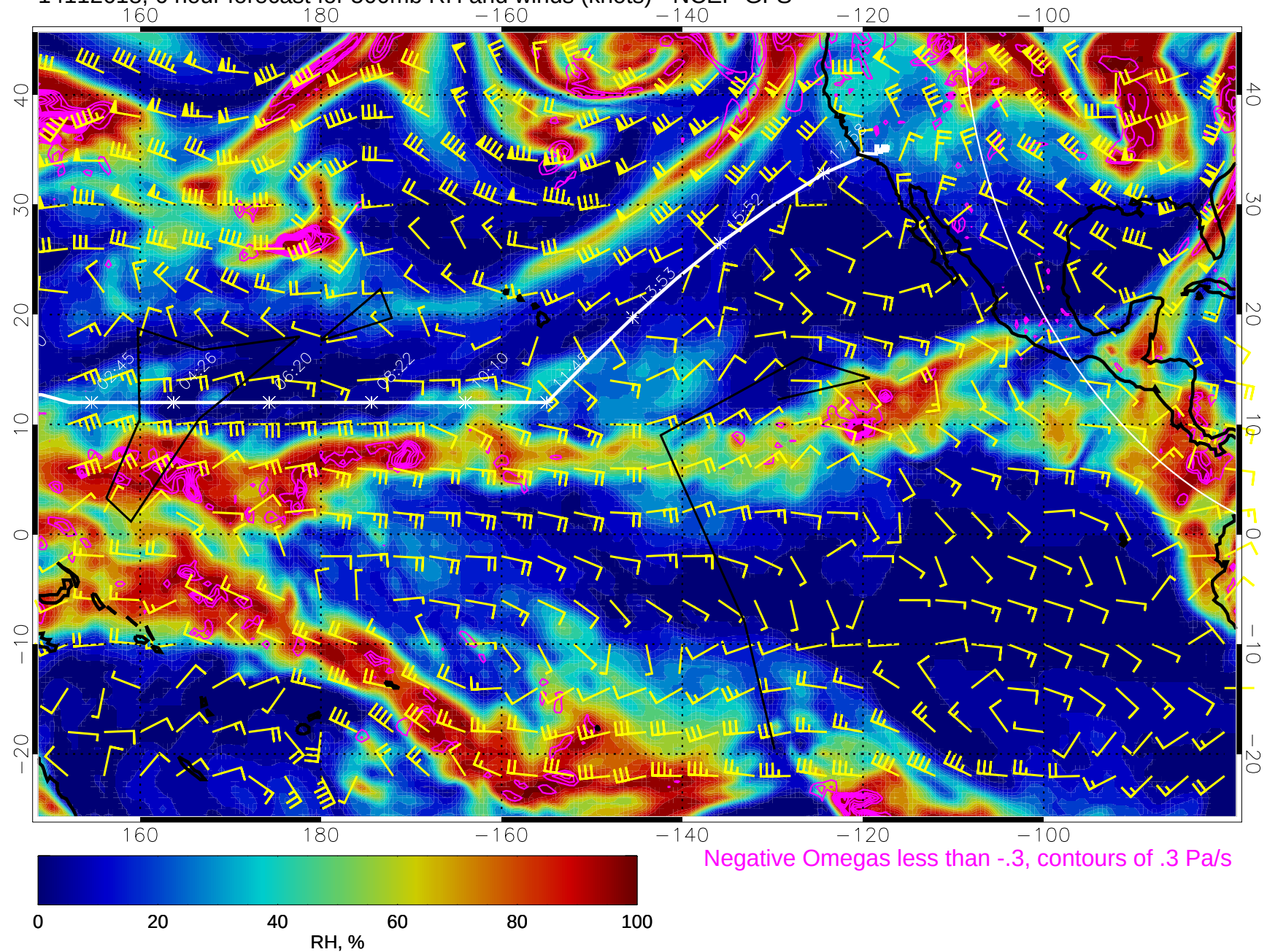
14112618, 6 hour forecast for 500mb RH and winds (knots) - NCEP GFS
