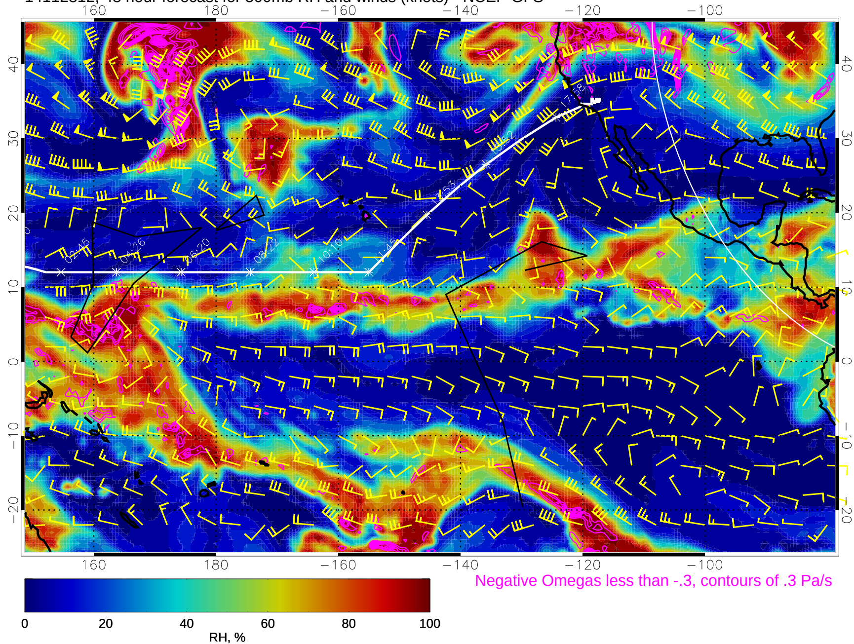
14112812, 48 hour forecast for 500mb RH and winds (knots) - NCEP GFS
