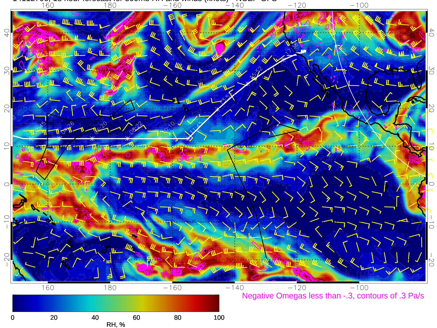
14112706, 18 hour forecast for 500mb RH and winds (knots) - NCEP GFS
