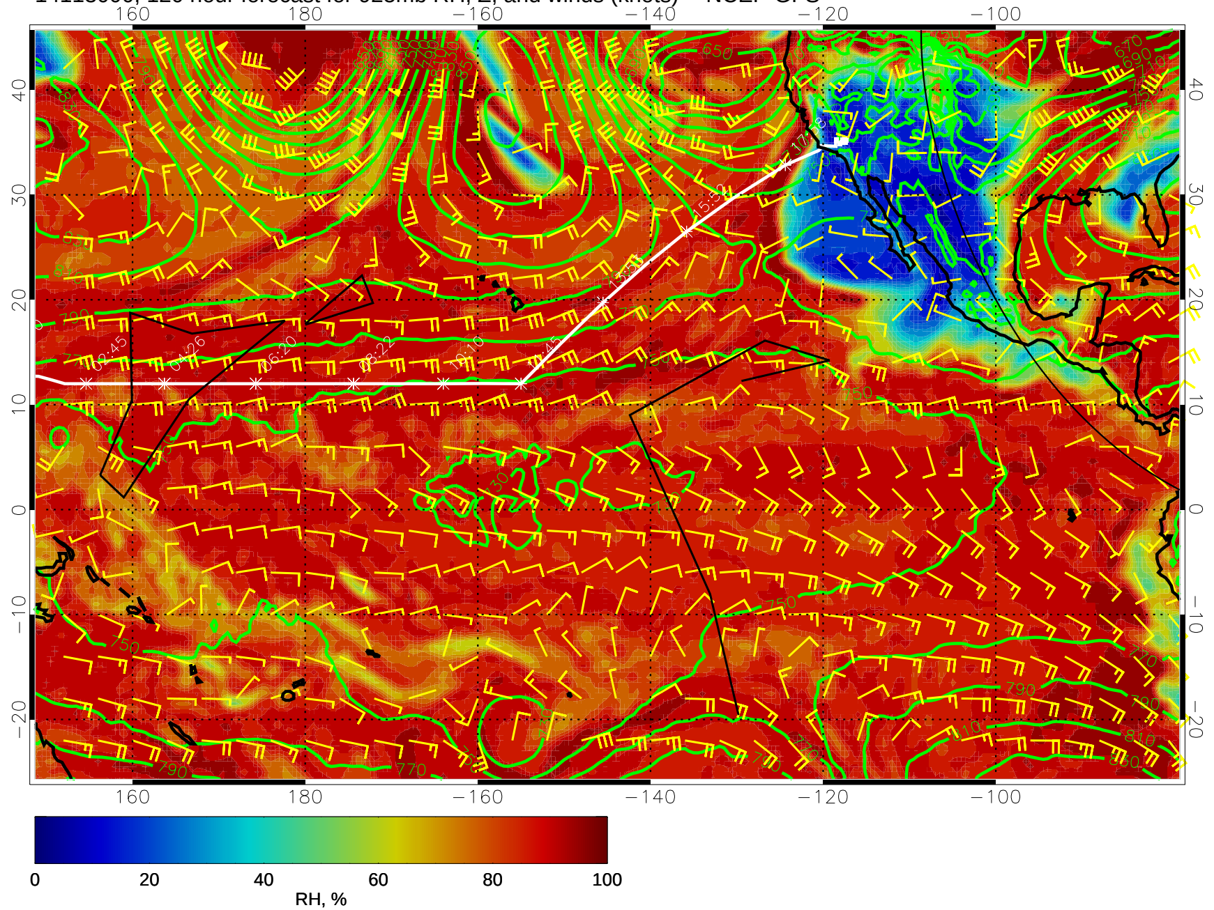
14113000, 120 hour forecast for 925mb RH, Z, and winds (knots) -- NCEP GFS
