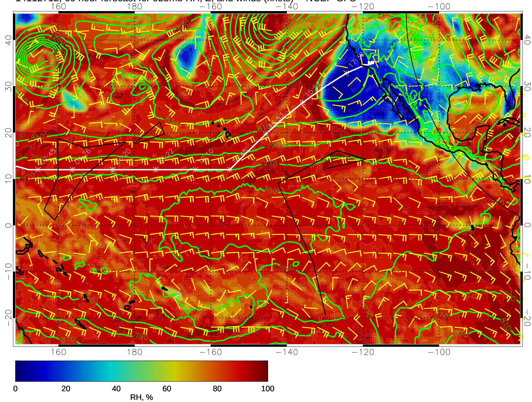
14112712, 60 hour forecast for 925mb RH, Z, and winds (knots) -- NCEP GFS
