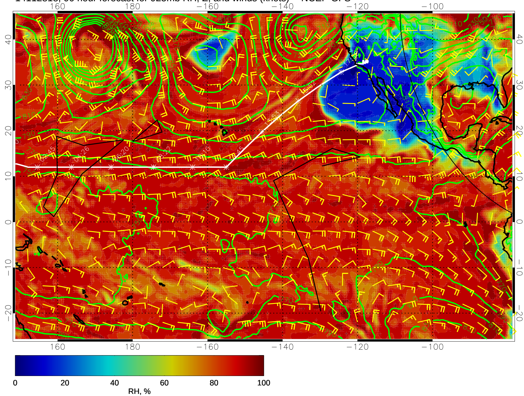
14112818, 90 hour forecast for 925mb RH, Z, and winds (knots) -- NCEP GFS
