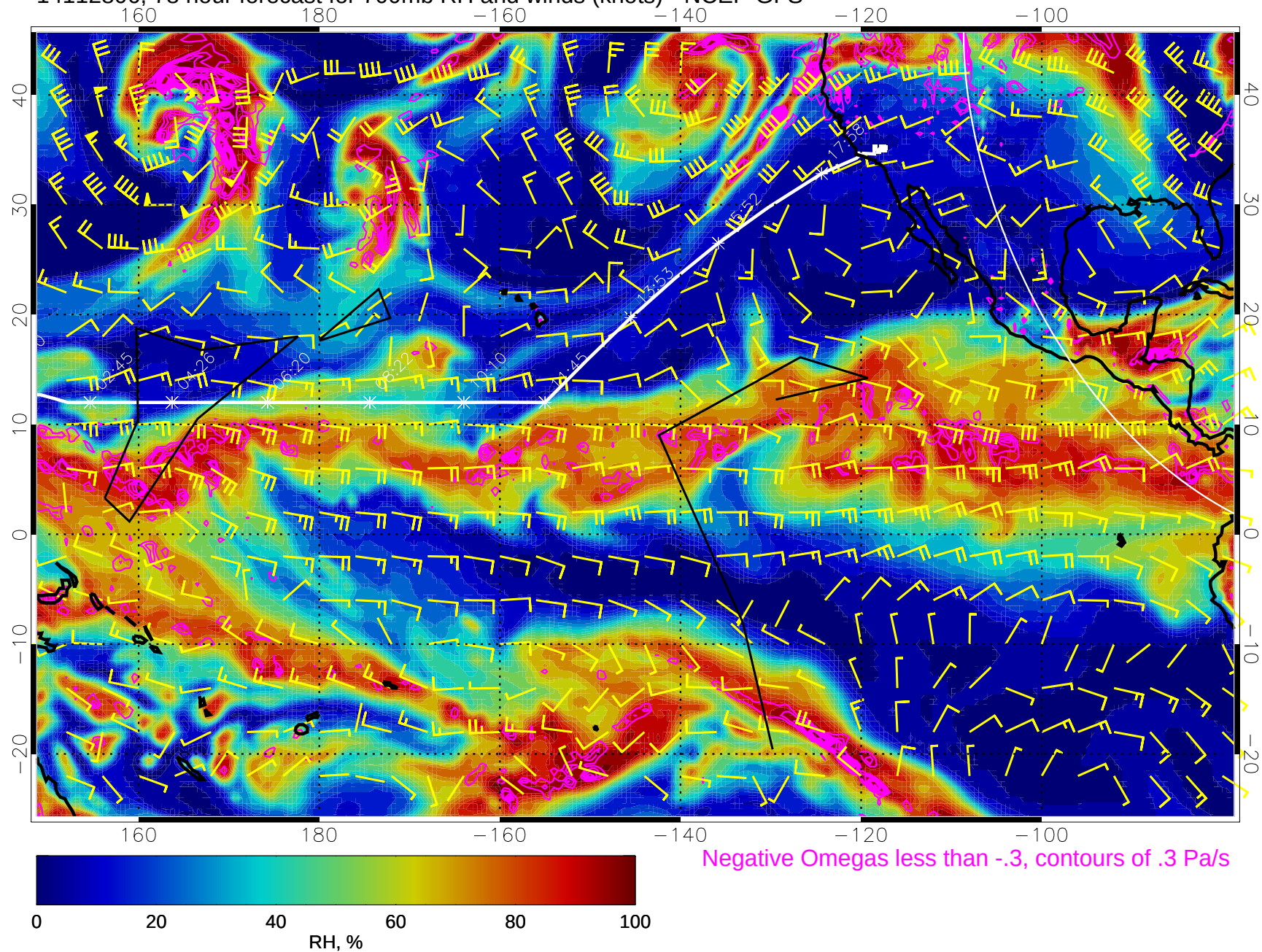
14112806, 78 hour forecast for 700mb RH and winds (knots) - NCEP GFS
