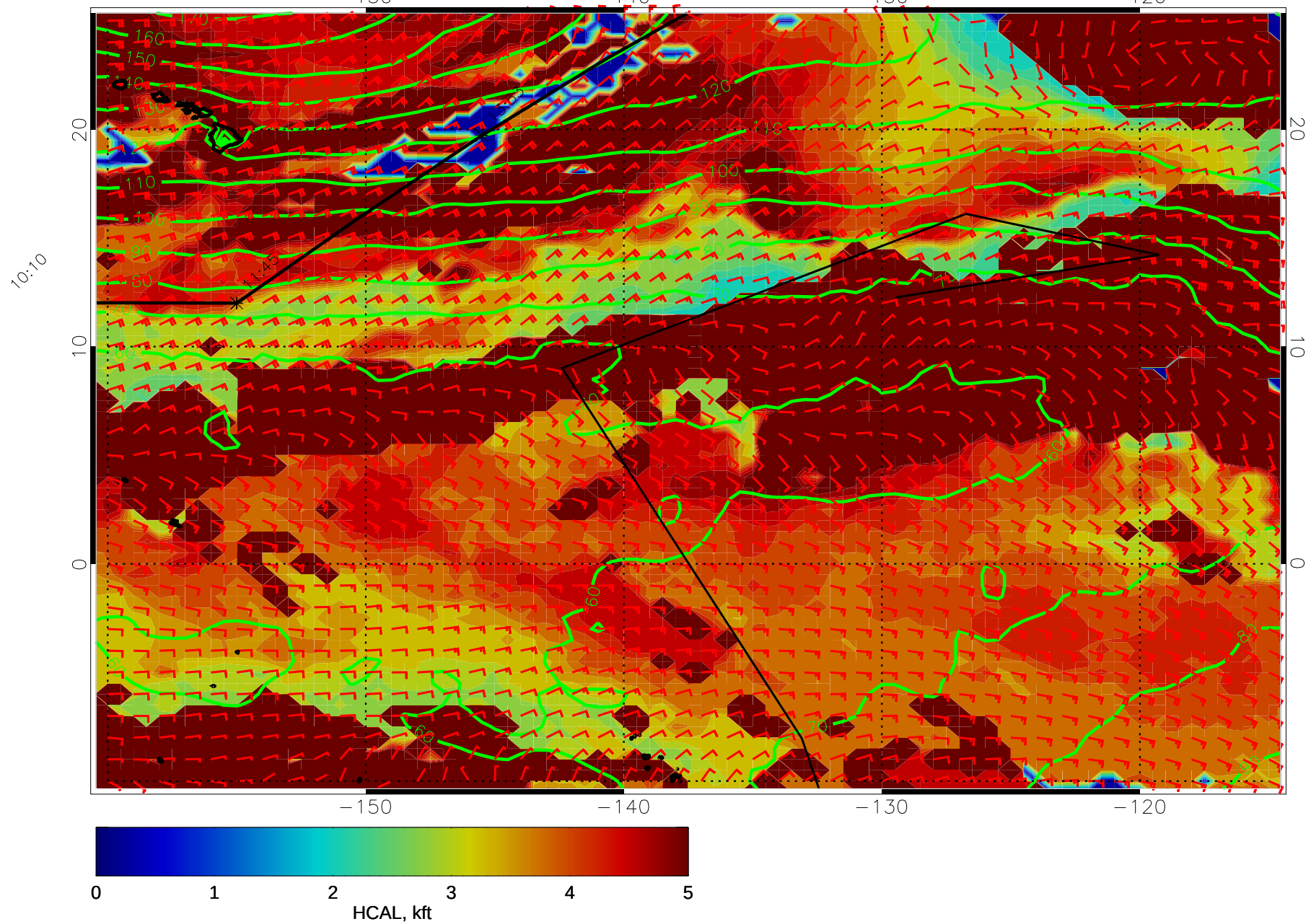
14112912, 108 hour forecast for HCAL, 1000mb Z, and winds (knots) -- NCEP GFS
