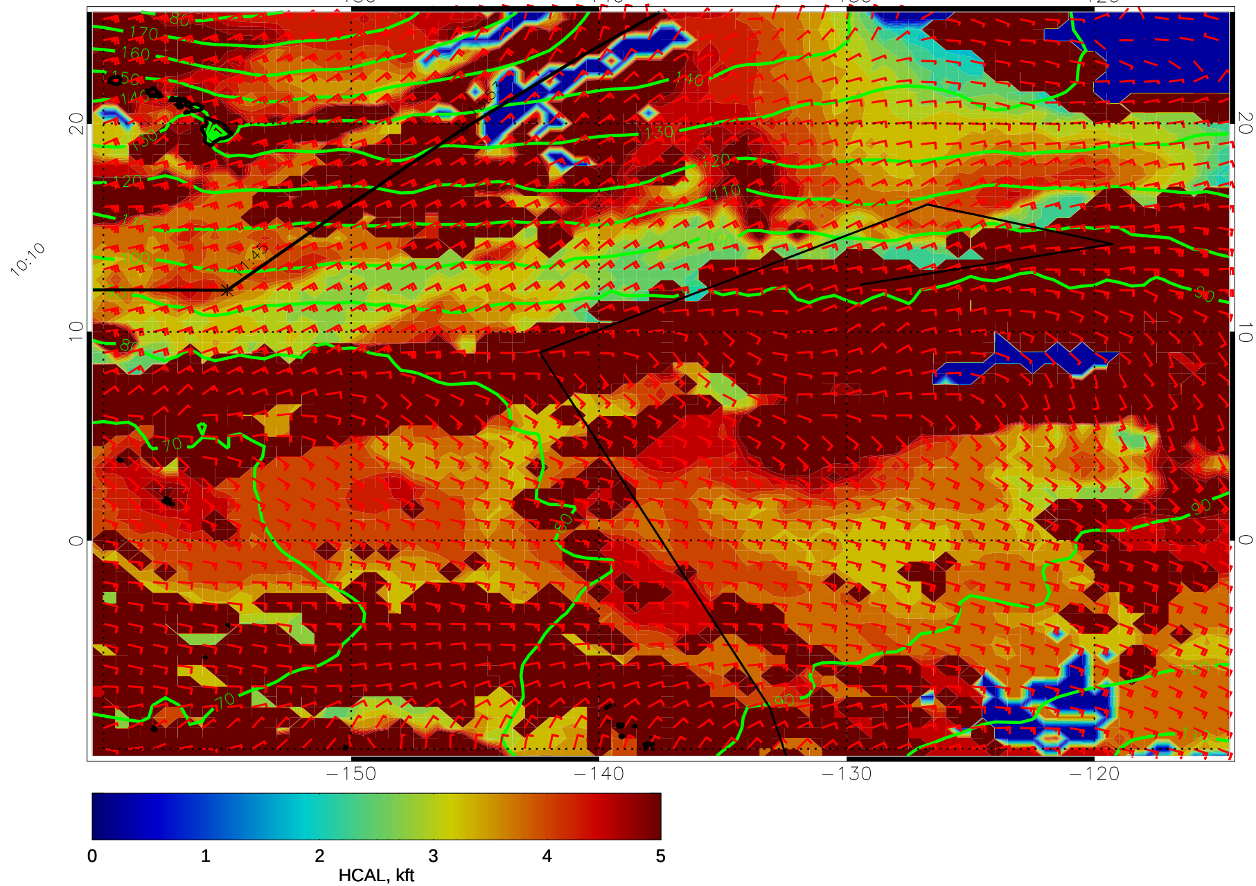
14112906, 102 hour forecast for HCAL, 1000mb Z, and winds (knots) -- NCEP GFS
