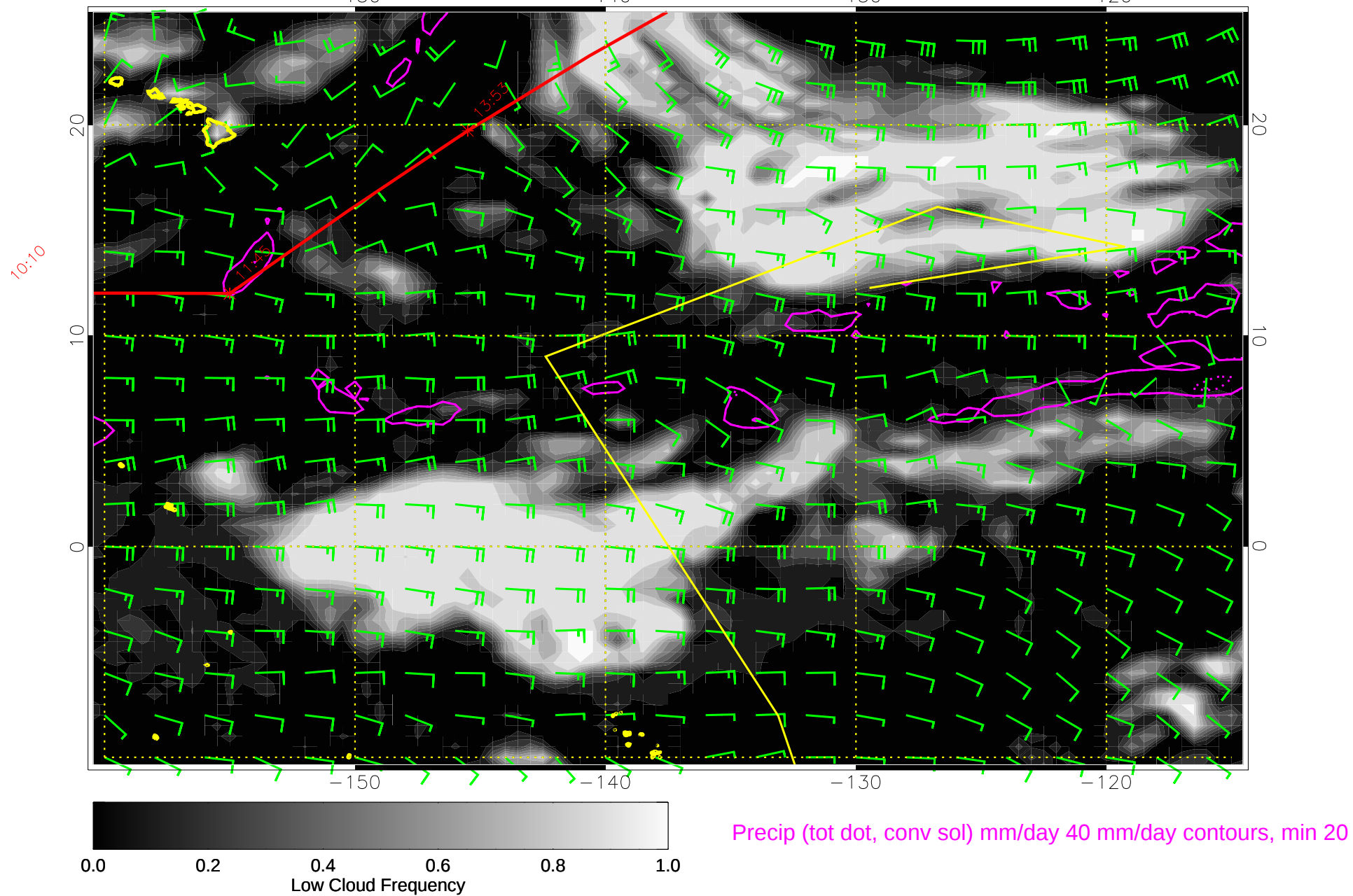
14112512, 12 hour forecast for 850mb winds (knots) and Low Cloud Frequency -- NCEP GFS
