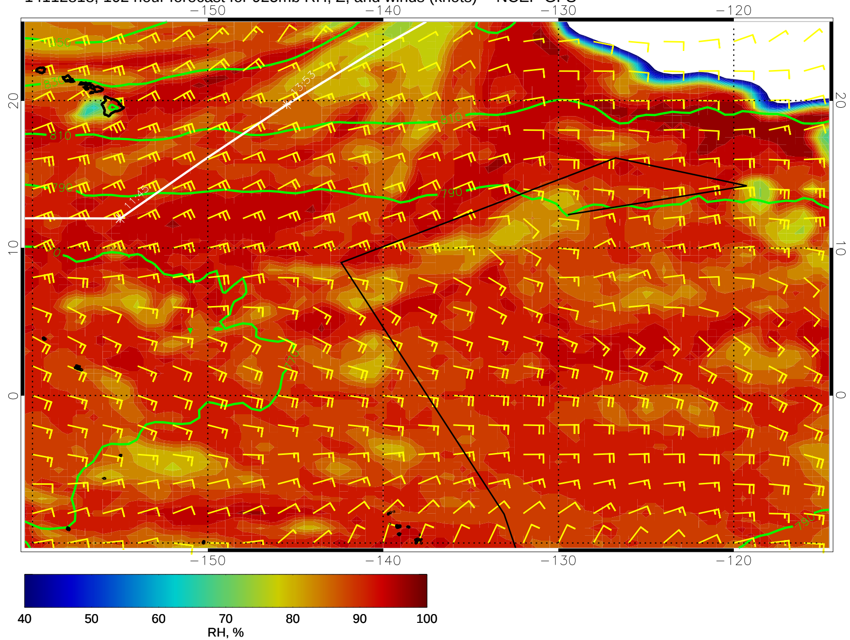
14112818, 102 hour forecast for 925mb RH, Z, and winds (knots) -- NCEP GFS
