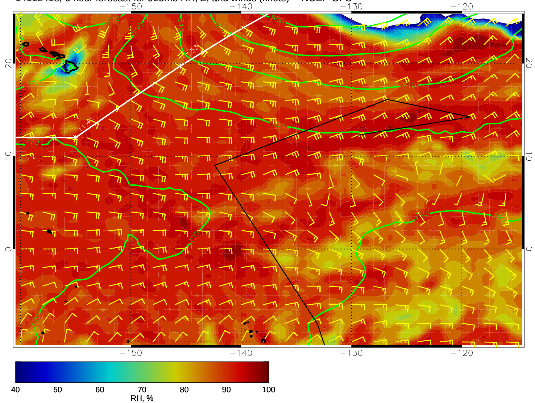
14112418, 6 hour forecast for 925mb RH, Z, and winds (knots) -- NCEP GFS
