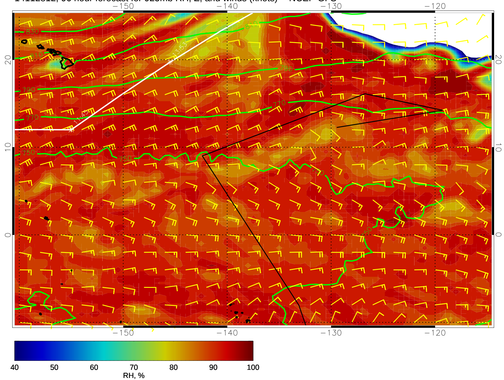
14112812, 96 hour forecast for 925mb RH, Z, and winds (knots) -- NCEP GFS
