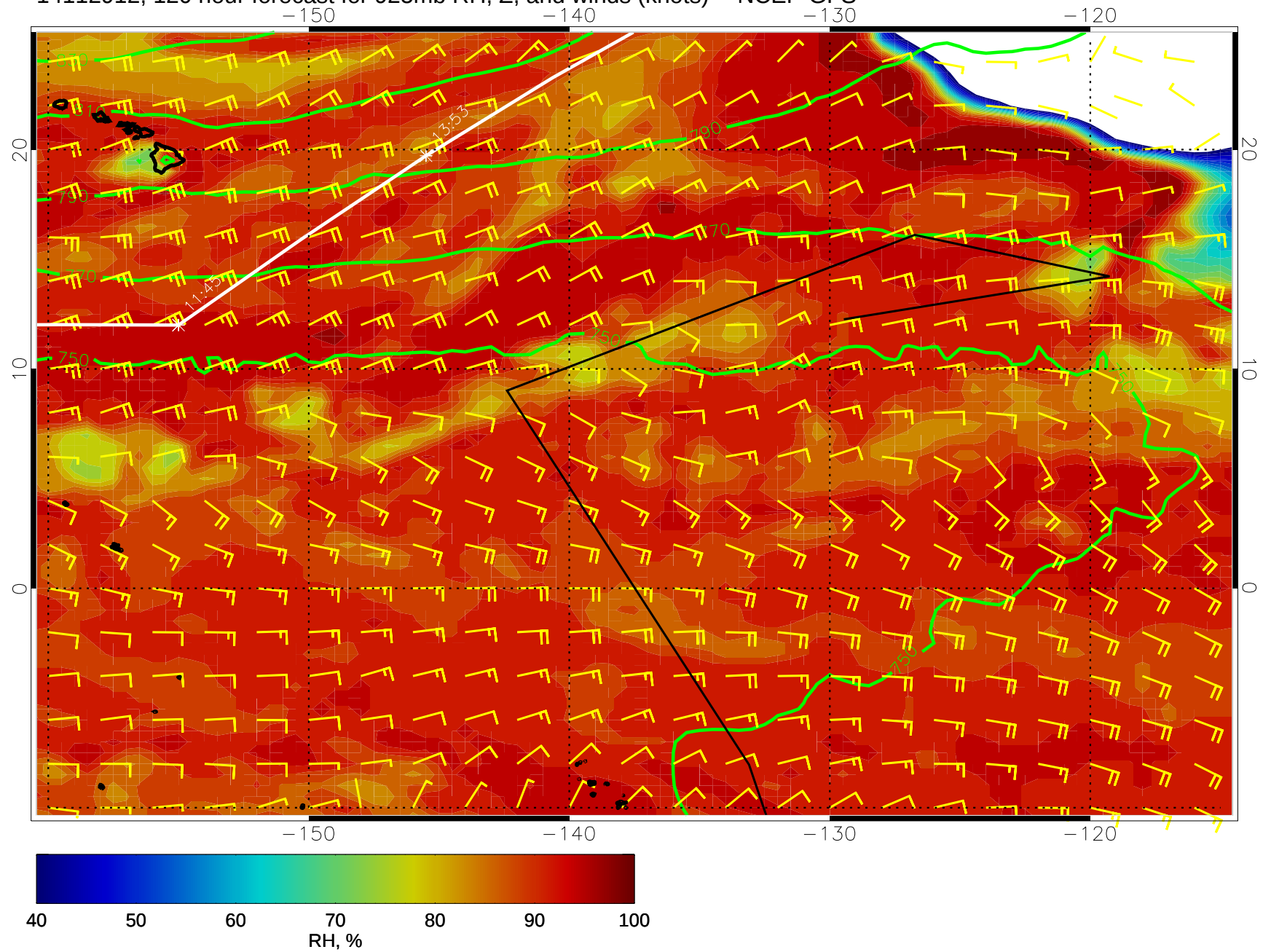
14112912, 120 hour forecast for 925mb RH, Z, and winds (knots) -- NCEP GFS
