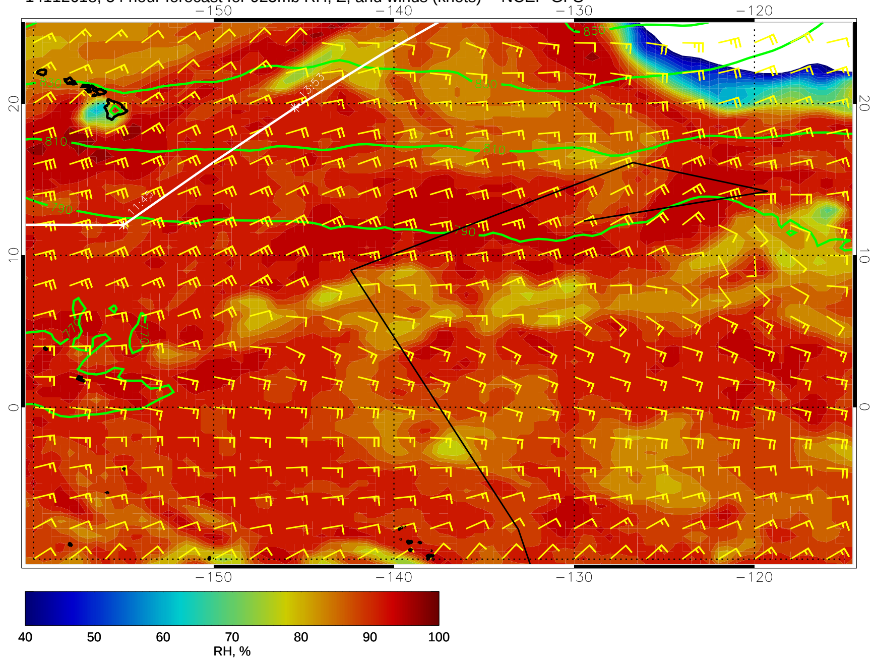
14112618, 54 hour forecast for 925mb RH, Z, and winds (knots) -- NCEP GFS
