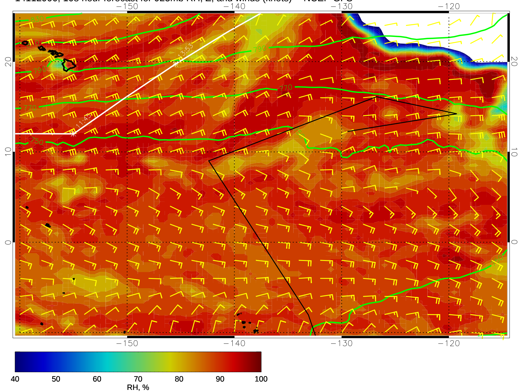
14112900, 108 hour forecast for 925mb RH, Z, and winds (knots) -- NCEP GFS
