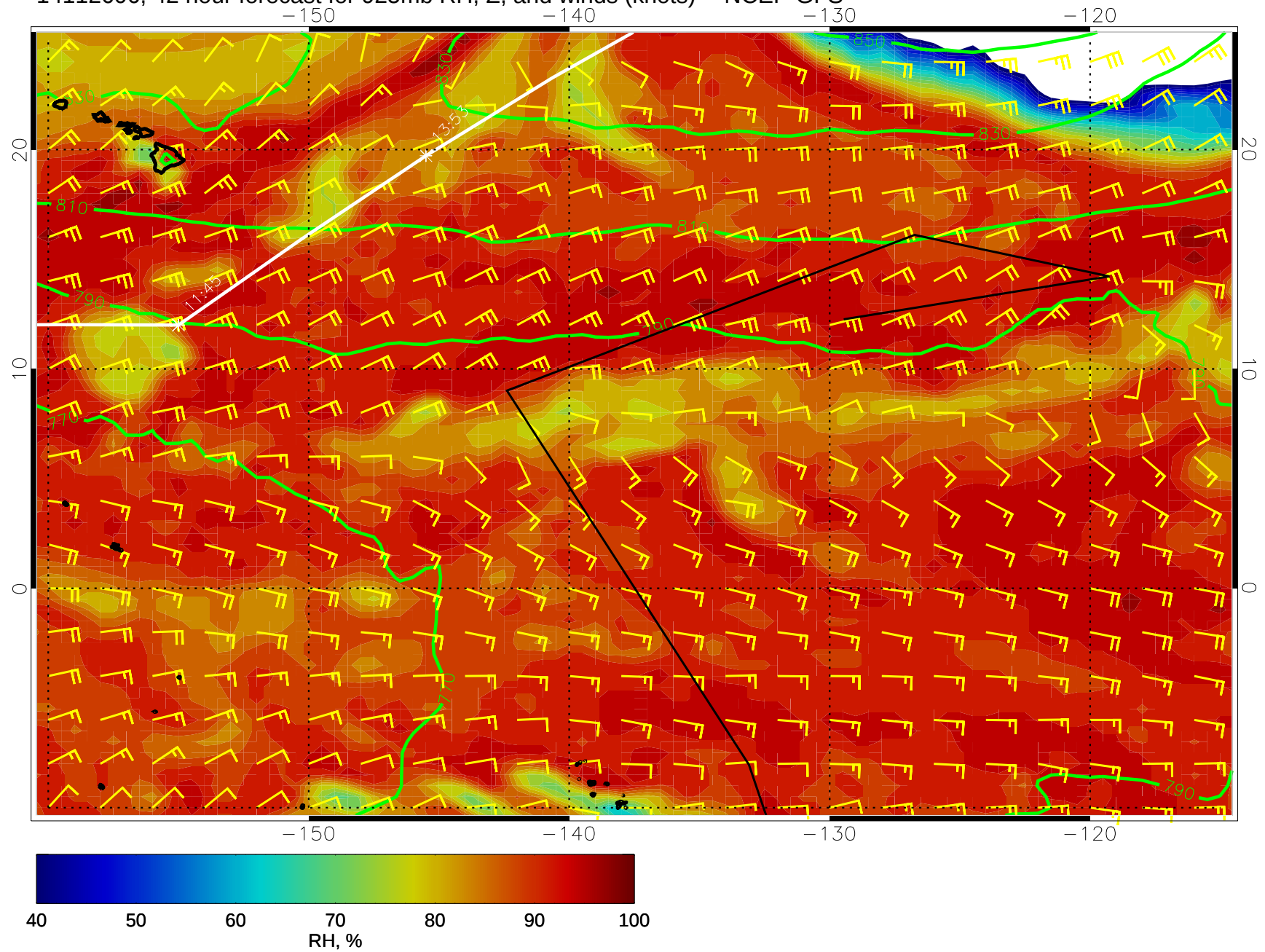
14112606, 42 hour forecast for 925mb RH, Z, and winds (knots) -- NCEP GFS
