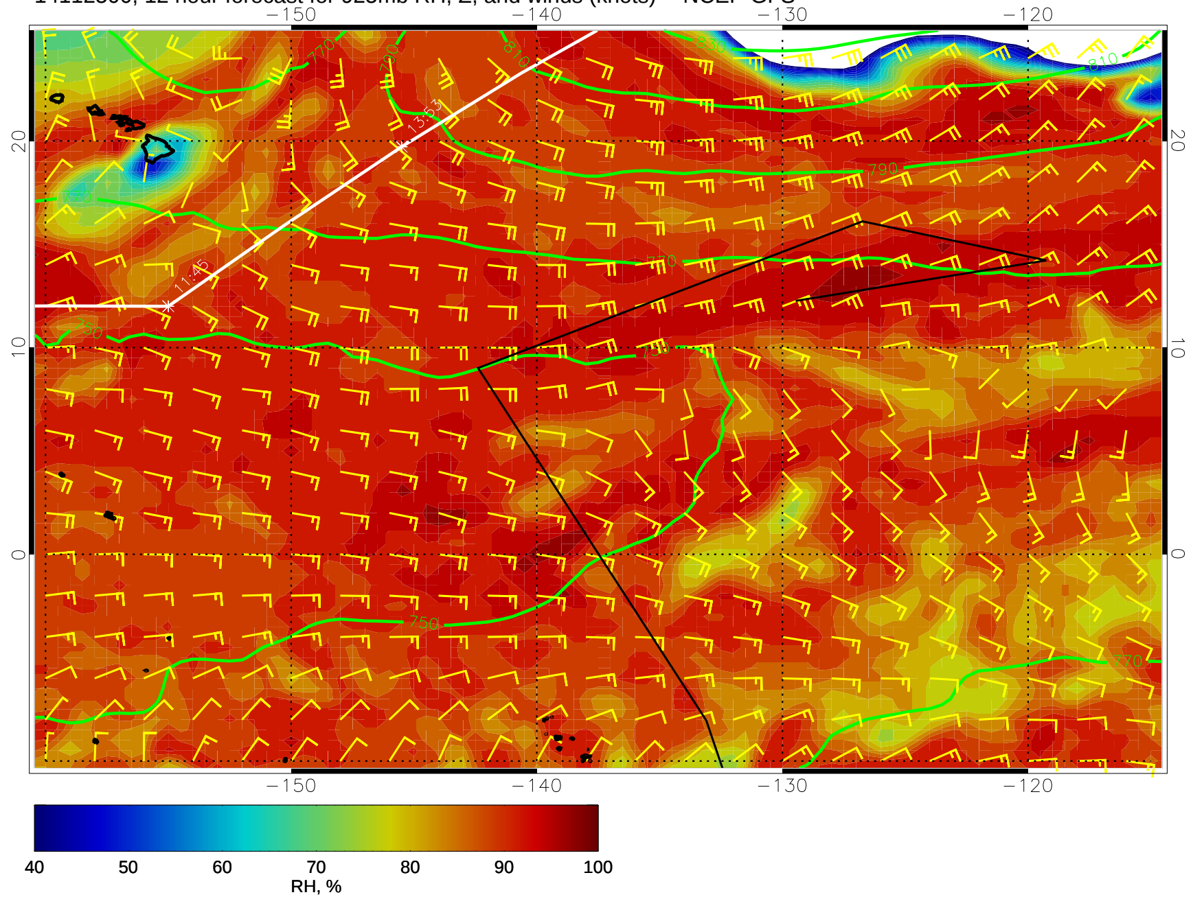
14112500, 12 hour forecast for 925mb RH, Z, and winds (knots) -- NCEP GFS
