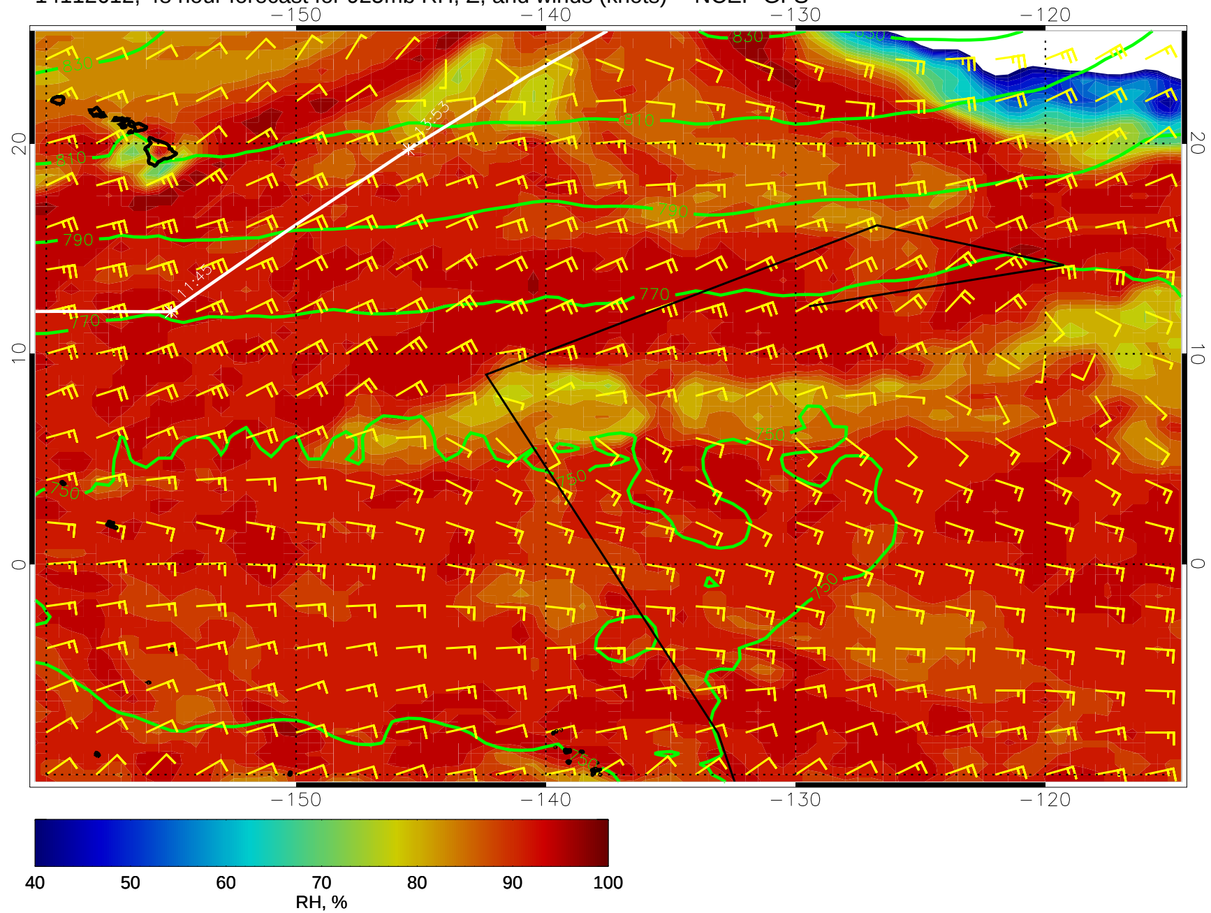
14112612, 48 hour forecast for 925mb RH, Z, and winds (knots) -- NCEP GFS
