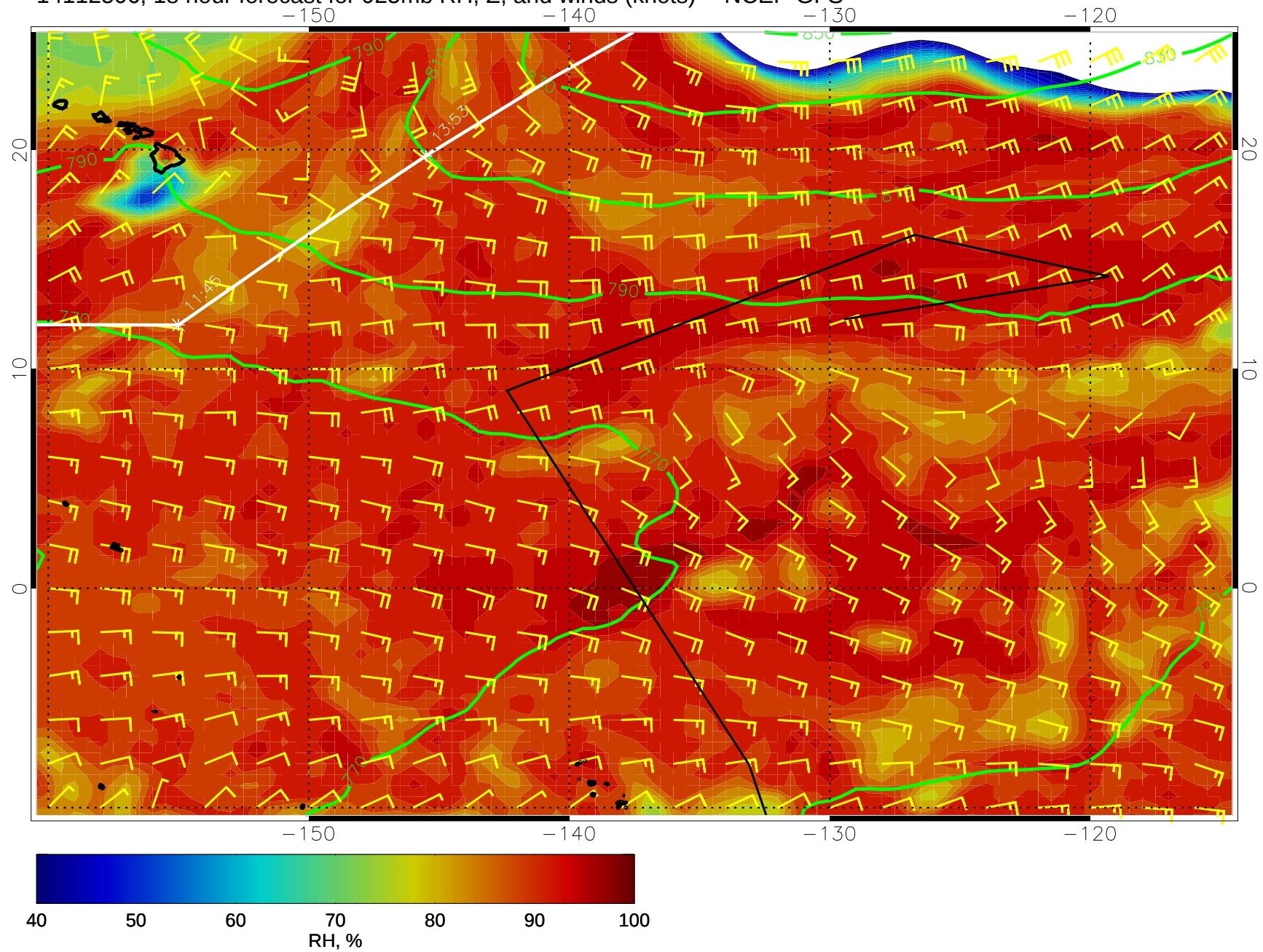
14112506, 18 hour forecast for 925mb RH, Z, and winds (knots) -- NCEP GFS
