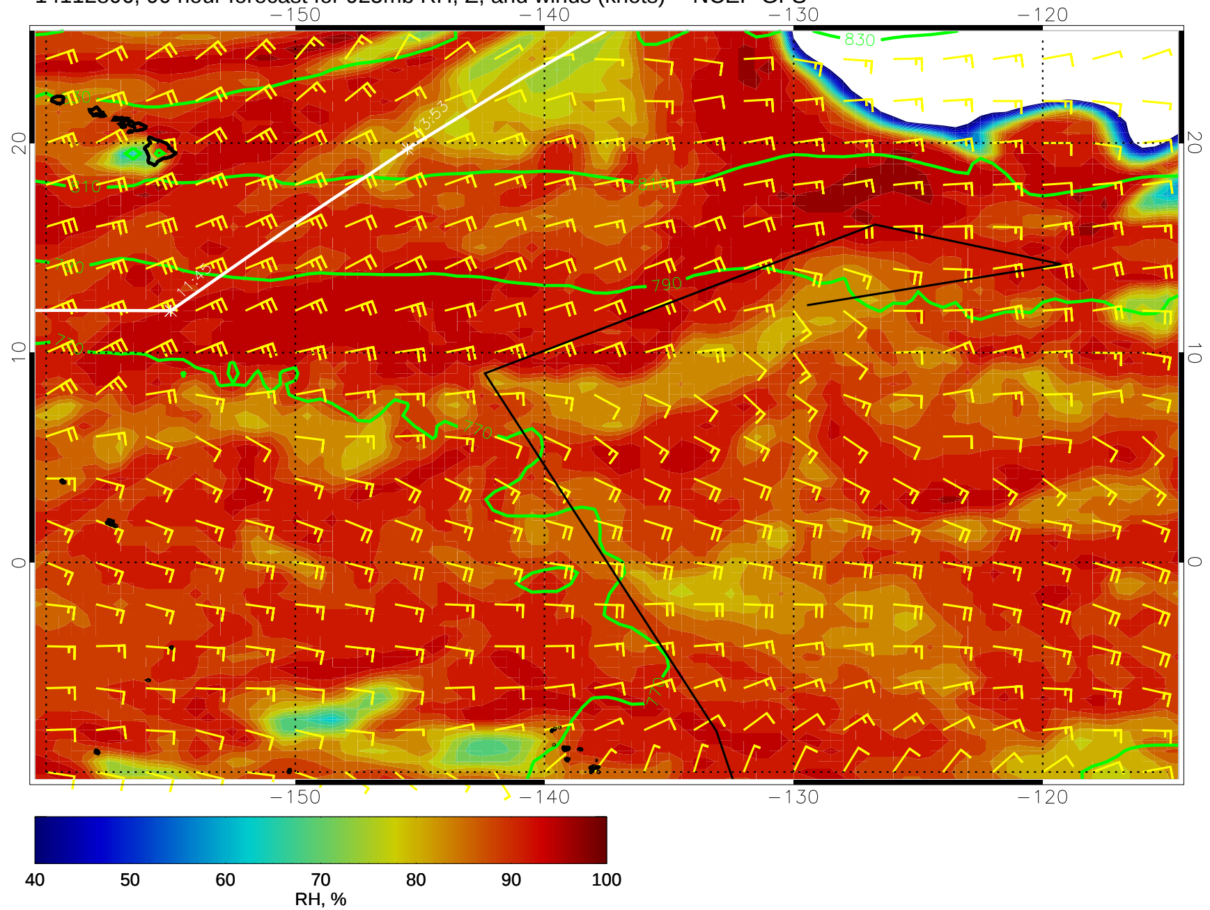
14112806, 90 hour forecast for 925mb RH, Z, and winds (knots) -- NCEP GFS
