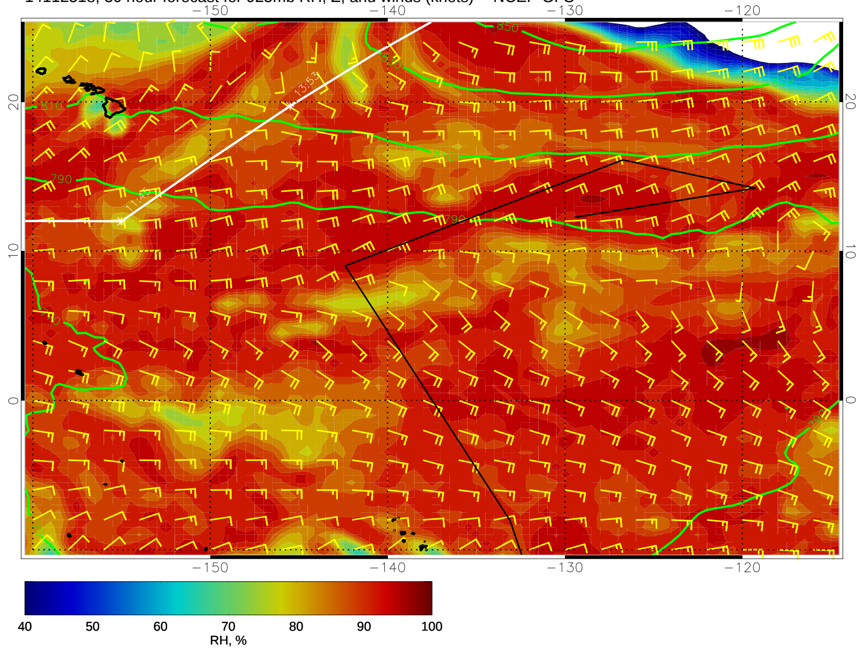
14112518, 30 hour forecast for 925mb RH, Z, and winds (knots) -- NCEP GFS
