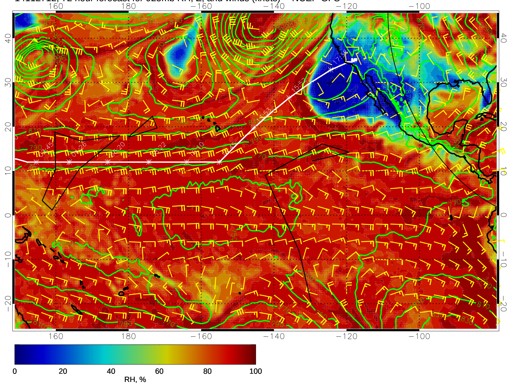
14112712, 72 hour forecast for 925mb RH, Z, and winds (knots) -- NCEP GFS
