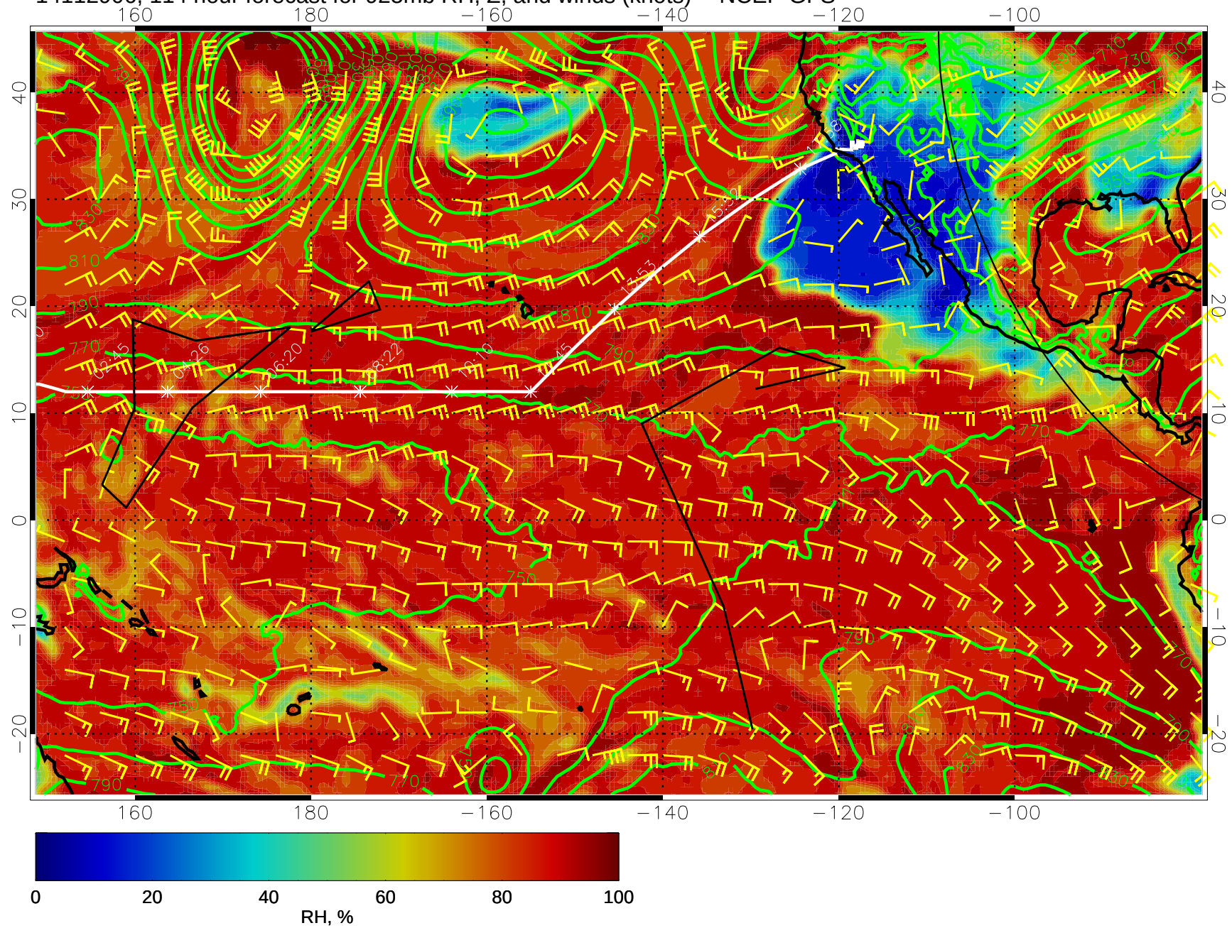
14112906, 114 hour forecast for 925mb RH, Z, and winds (knots) -- NCEP GFS
