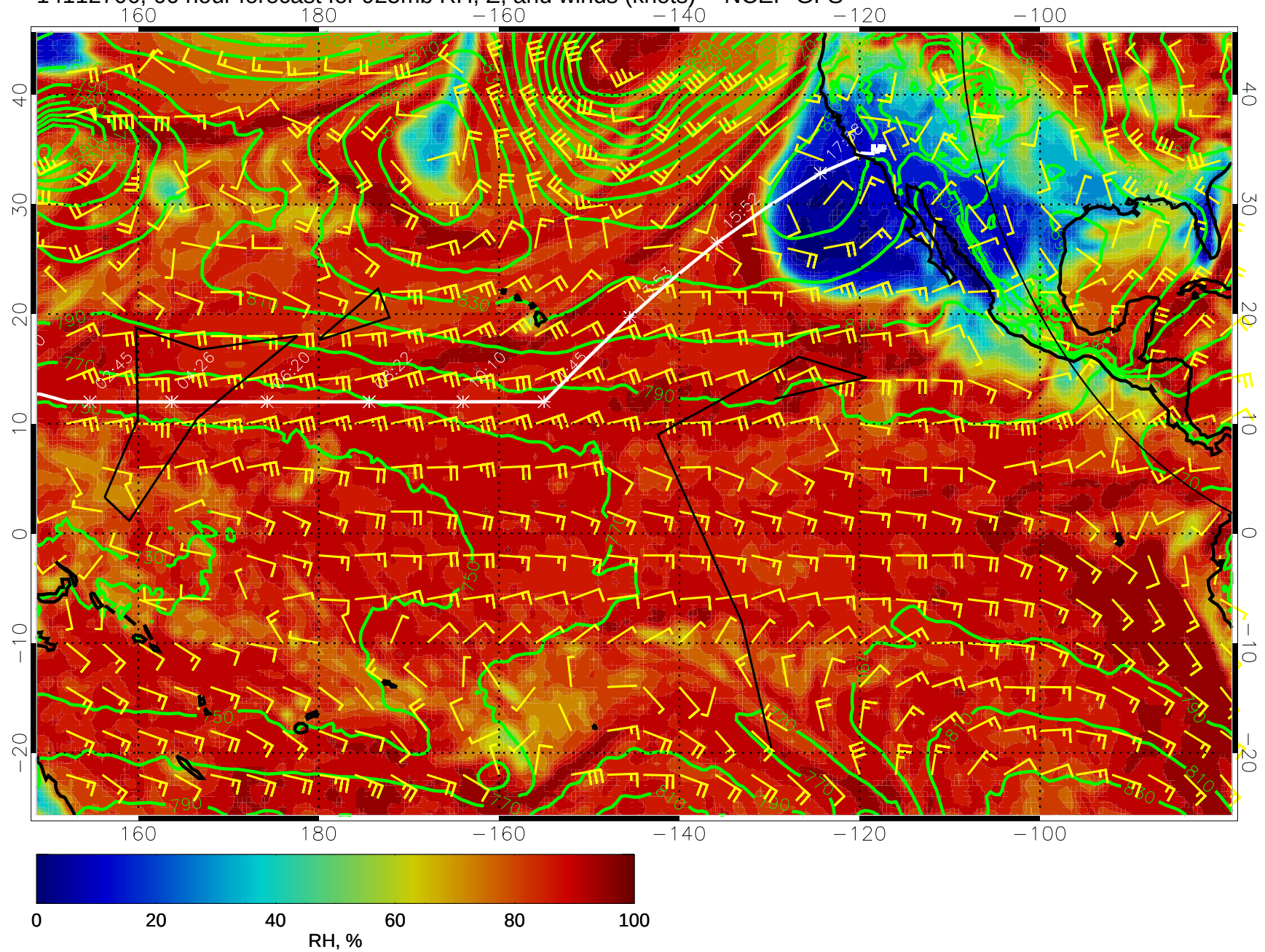
14112706, 66 hour forecast for 925mb RH, Z, and winds (knots) -- NCEP GFS
