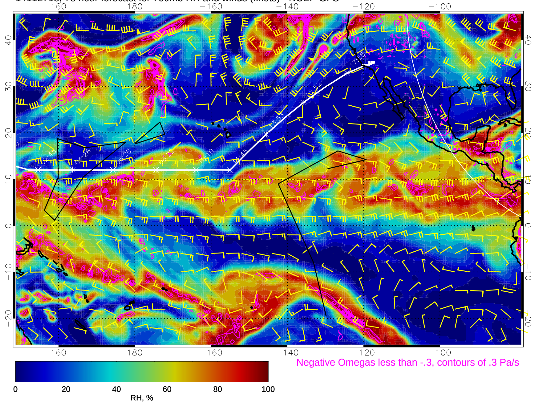
14112718, 78 hour forecast for 700mb RH and winds (knots) - NCEP GFS
