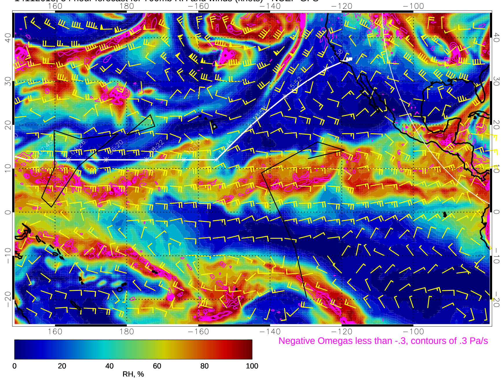
14112618, 54 hour forecast for 700mb RH and winds (knots) - NCEP GFS
