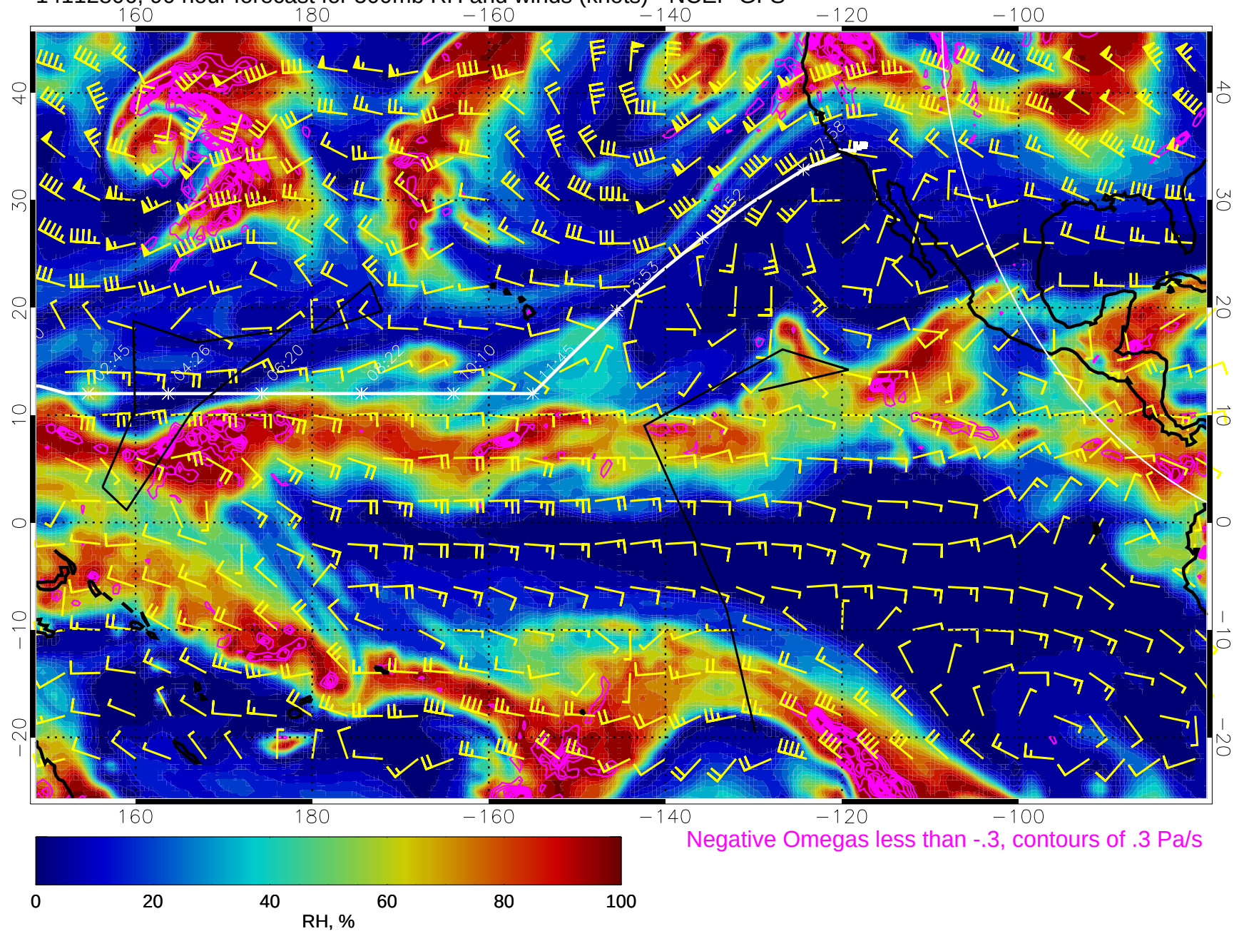
14112806, 90 hour forecast for 500mb RH and winds (knots) - NCEP GFS
