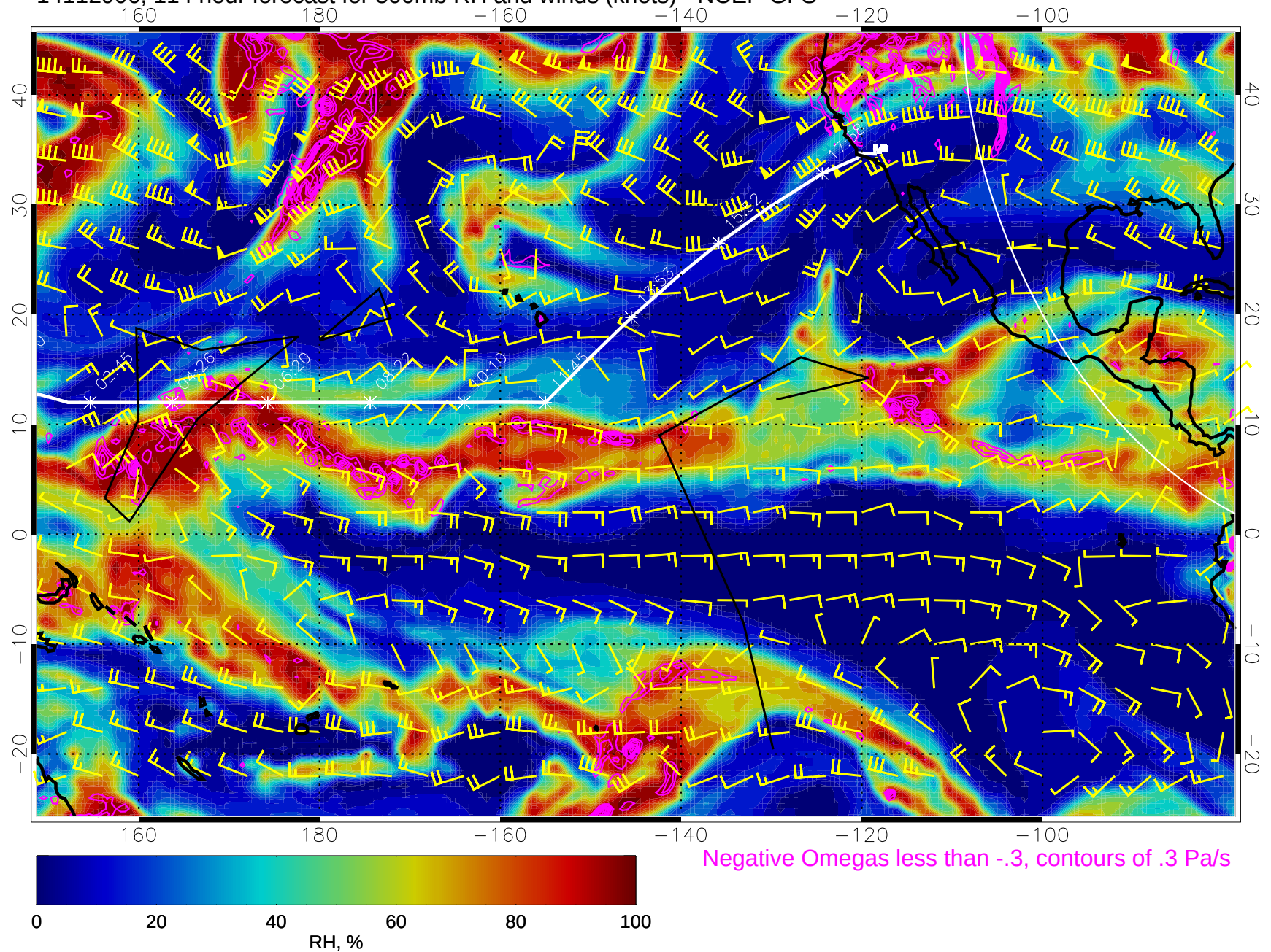
14112906, 114 hour forecast for 500mb RH and winds (knots) - NCEP GFS
