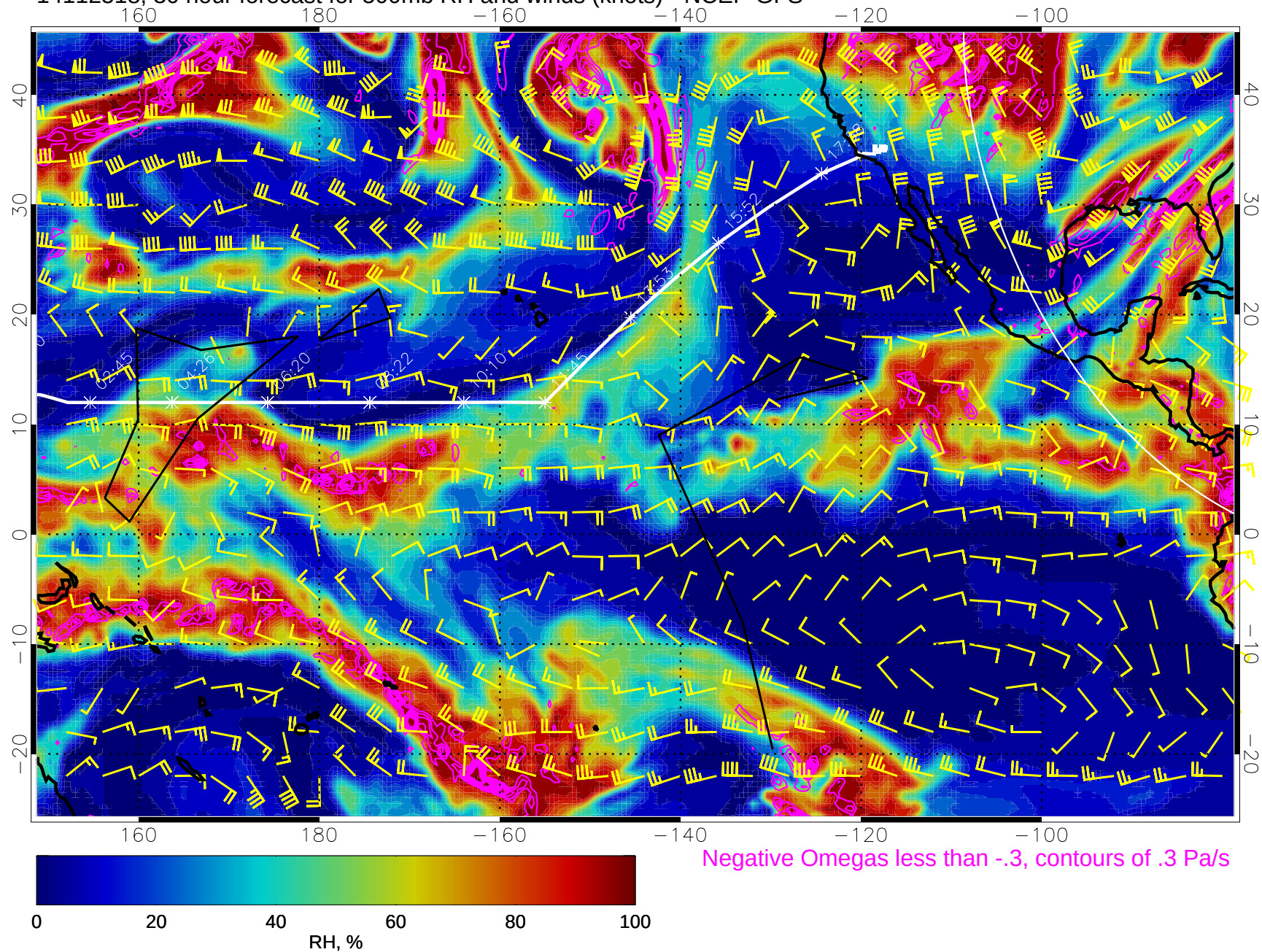
14112518, 30 hour forecast for 500mb RH and winds (knots) - NCEP GFS
