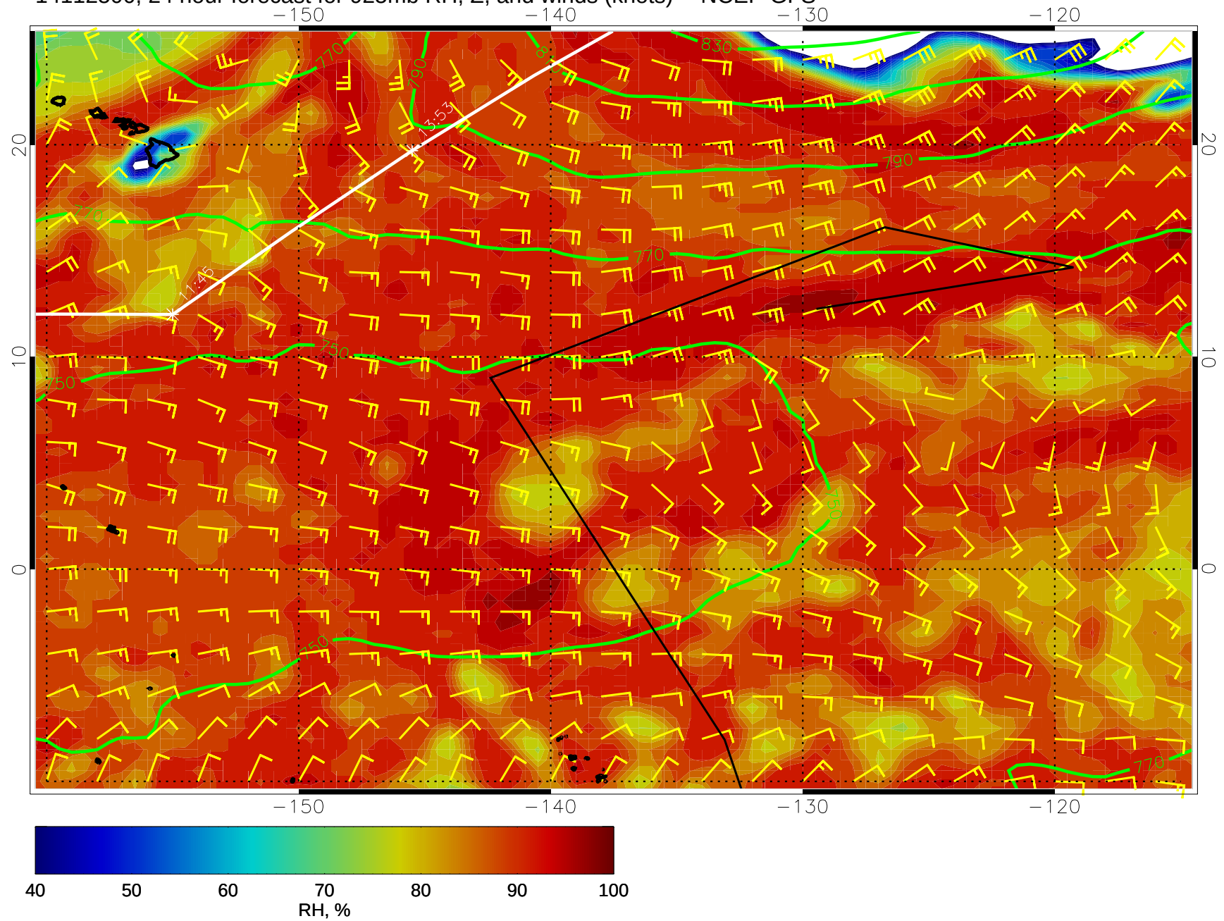
14112500, 24 hour forecast for 925mb RH, Z, and winds (knots) -- NCEP GFS
