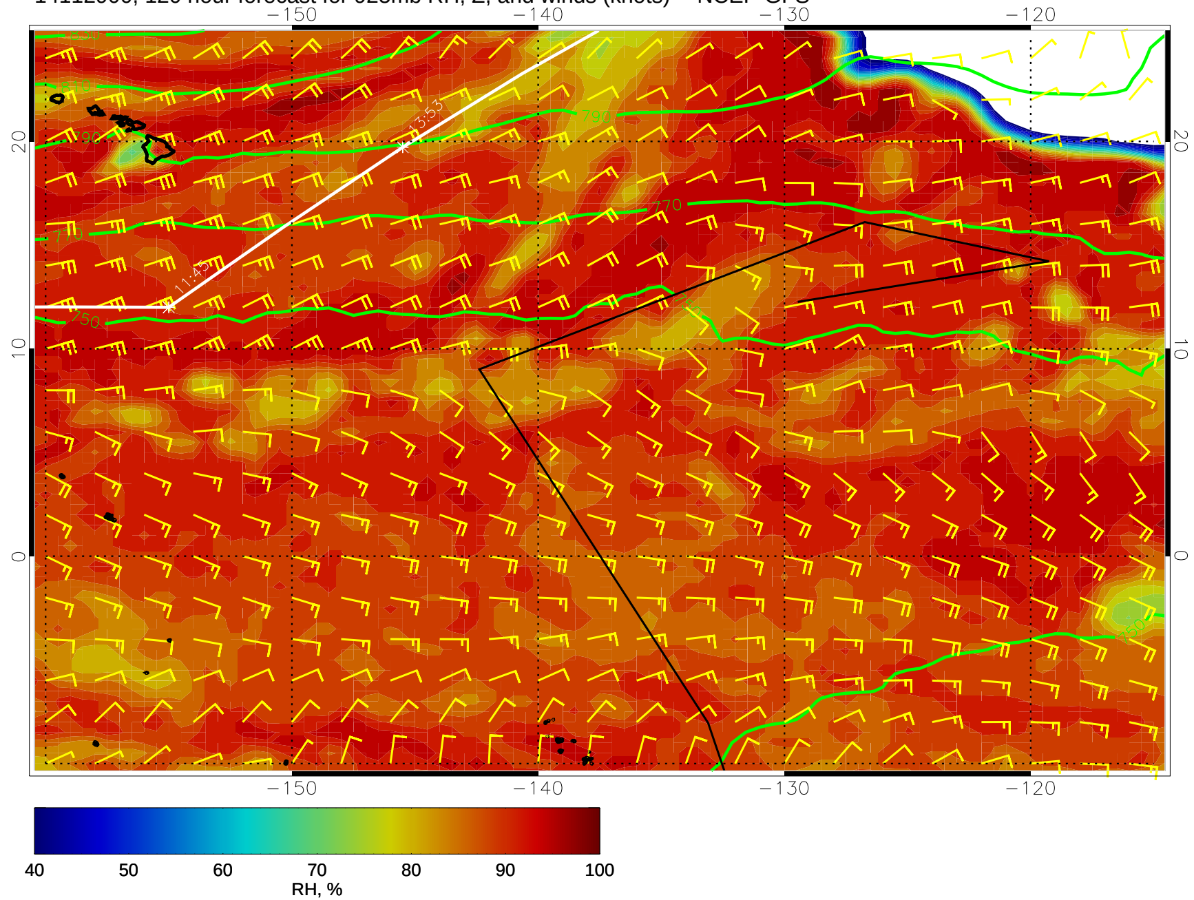
14112900, 120 hour forecast for 925mb RH, Z, and winds (knots) -- NCEP GFS
