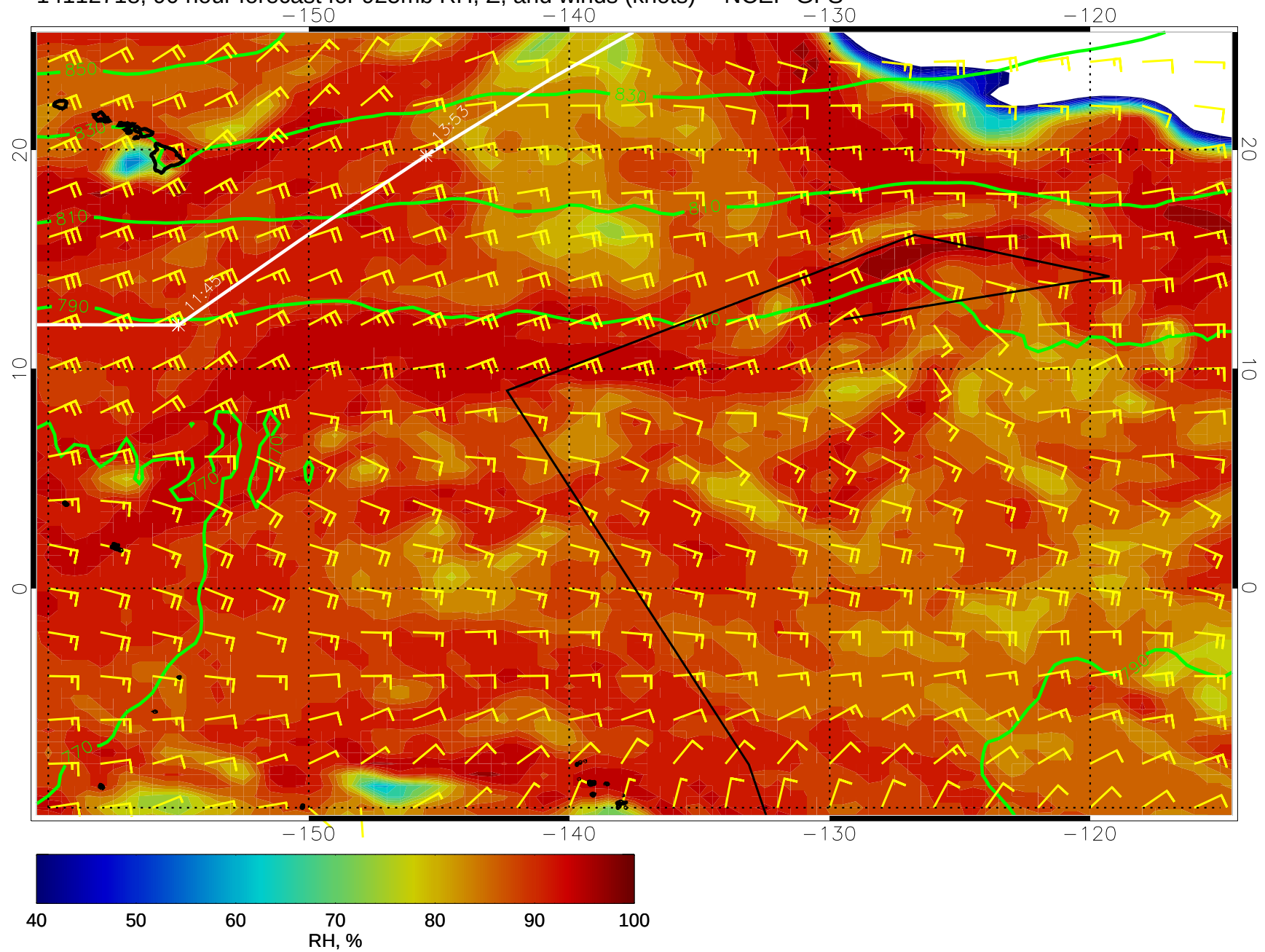
14112718, 90 hour forecast for 925mb RH, Z, and winds (knots) -- NCEP GFS
