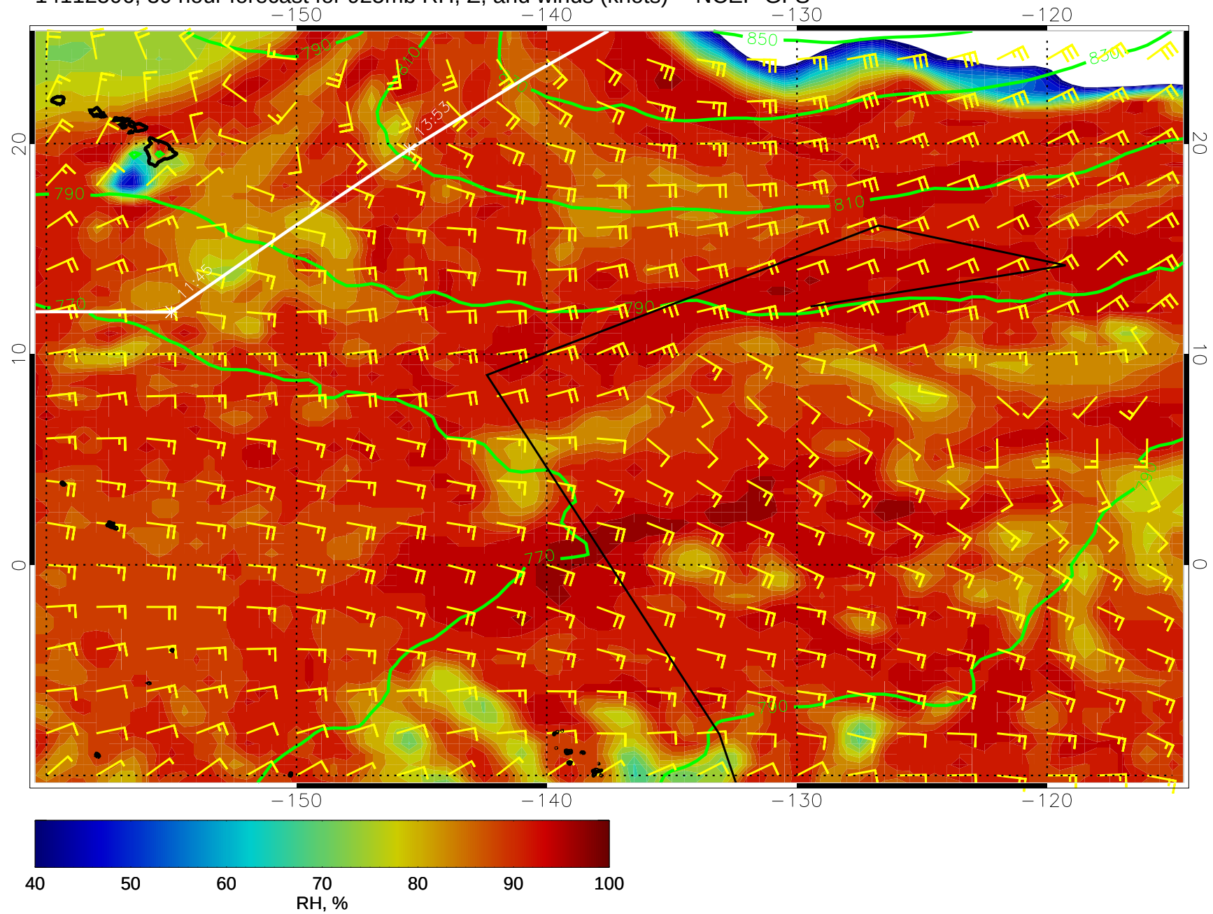
14112506, 30 hour forecast for 925mb RH, Z, and winds (knots) -- NCEP GFS
