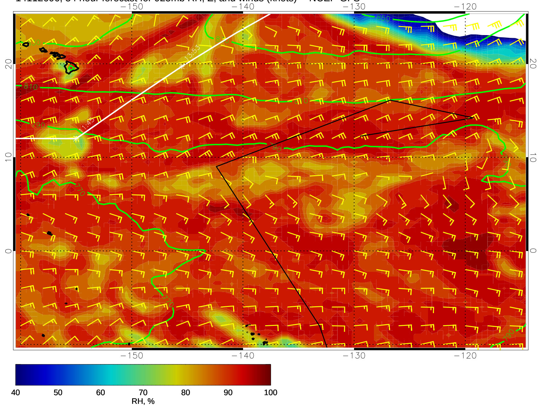
14112606, 54 hour forecast for 925mb RH, Z, and winds (knots) -- NCEP GFS
