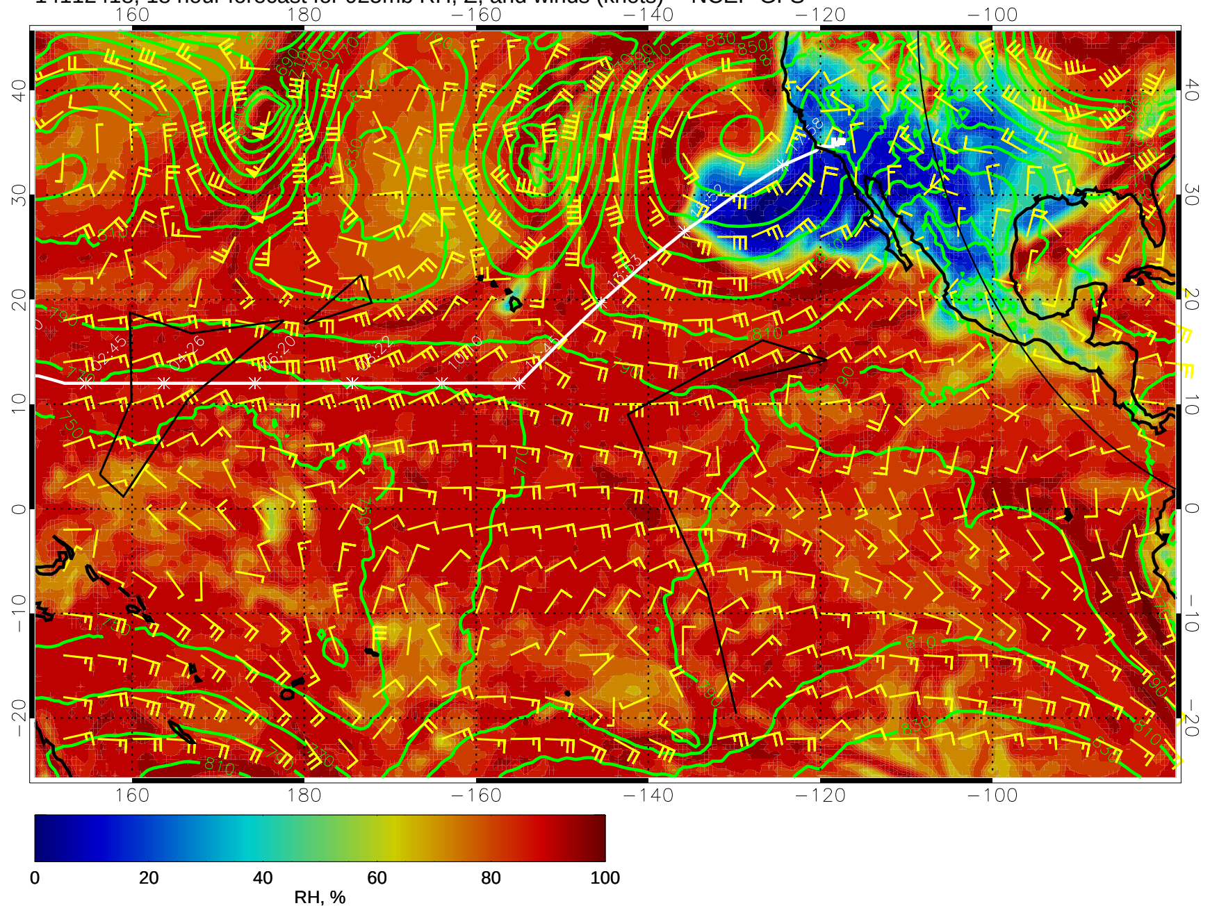
14112418, 18 hour forecast for 925mb RH, Z, and winds (knots) -- NCEP GFS
