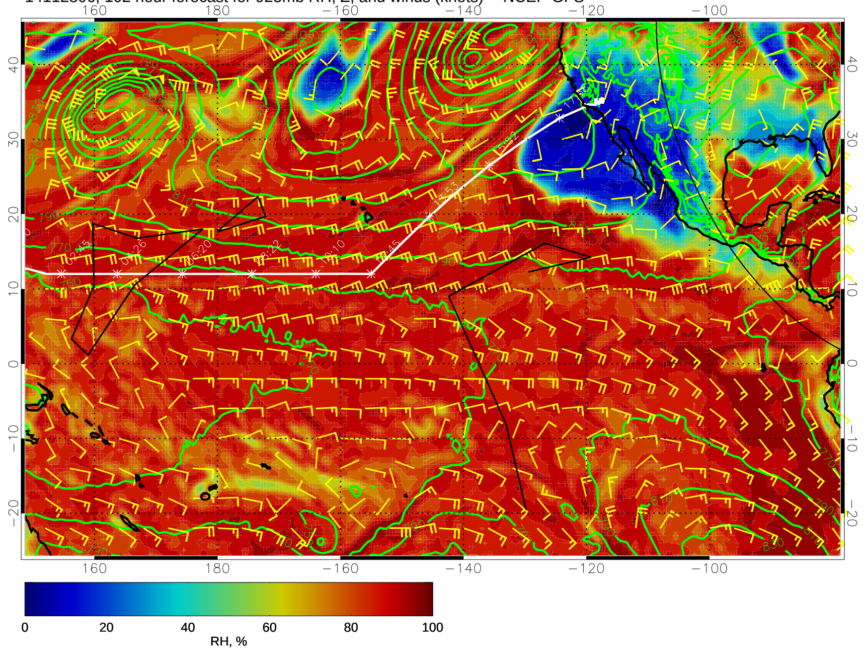
14112806, 102 hour forecast for 925mb RH, Z, and winds (knots) -- NCEP GFS
