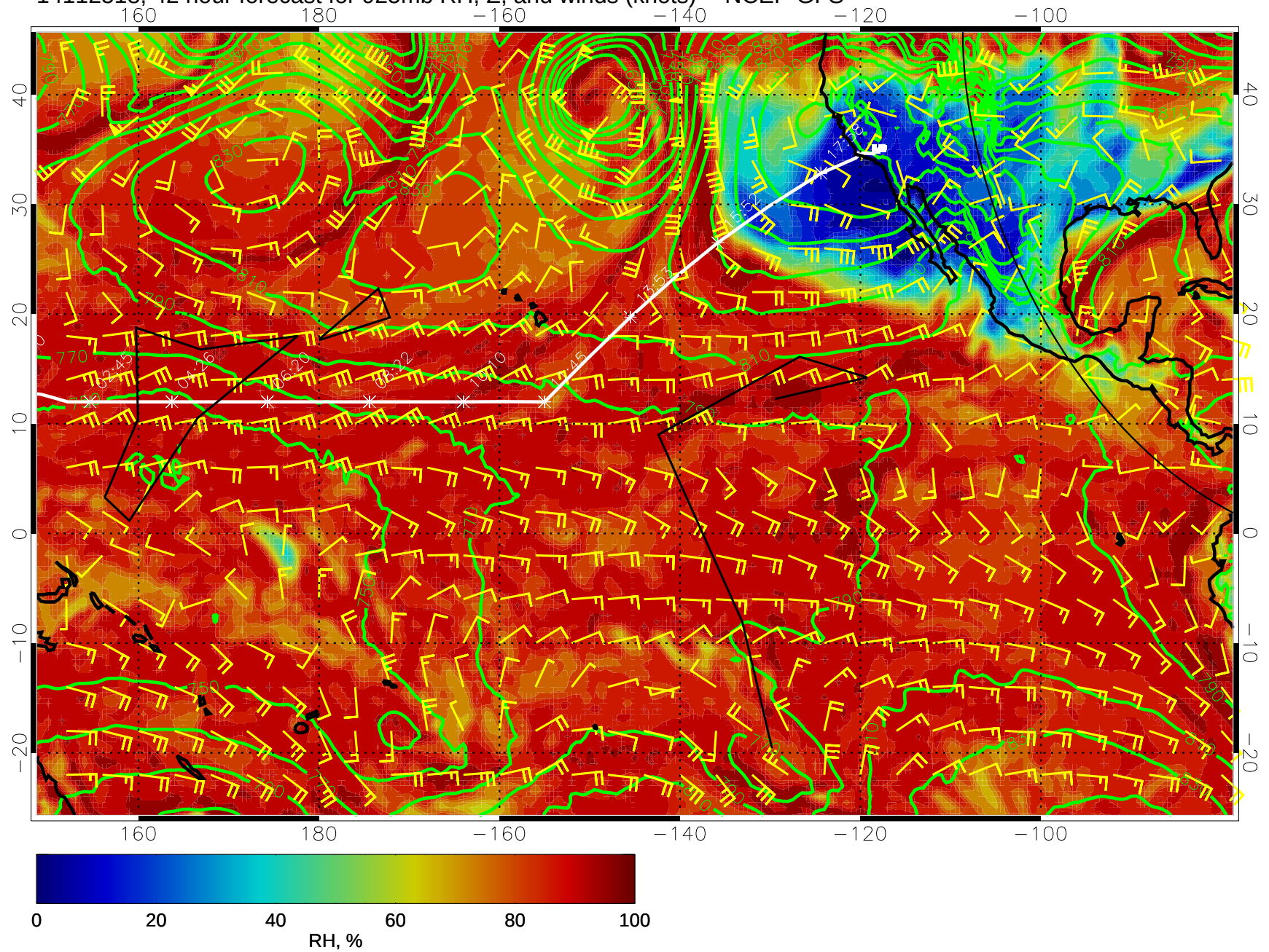
14112518, 42 hour forecast for 925mb RH, Z, and winds (knots) -- NCEP GFS
