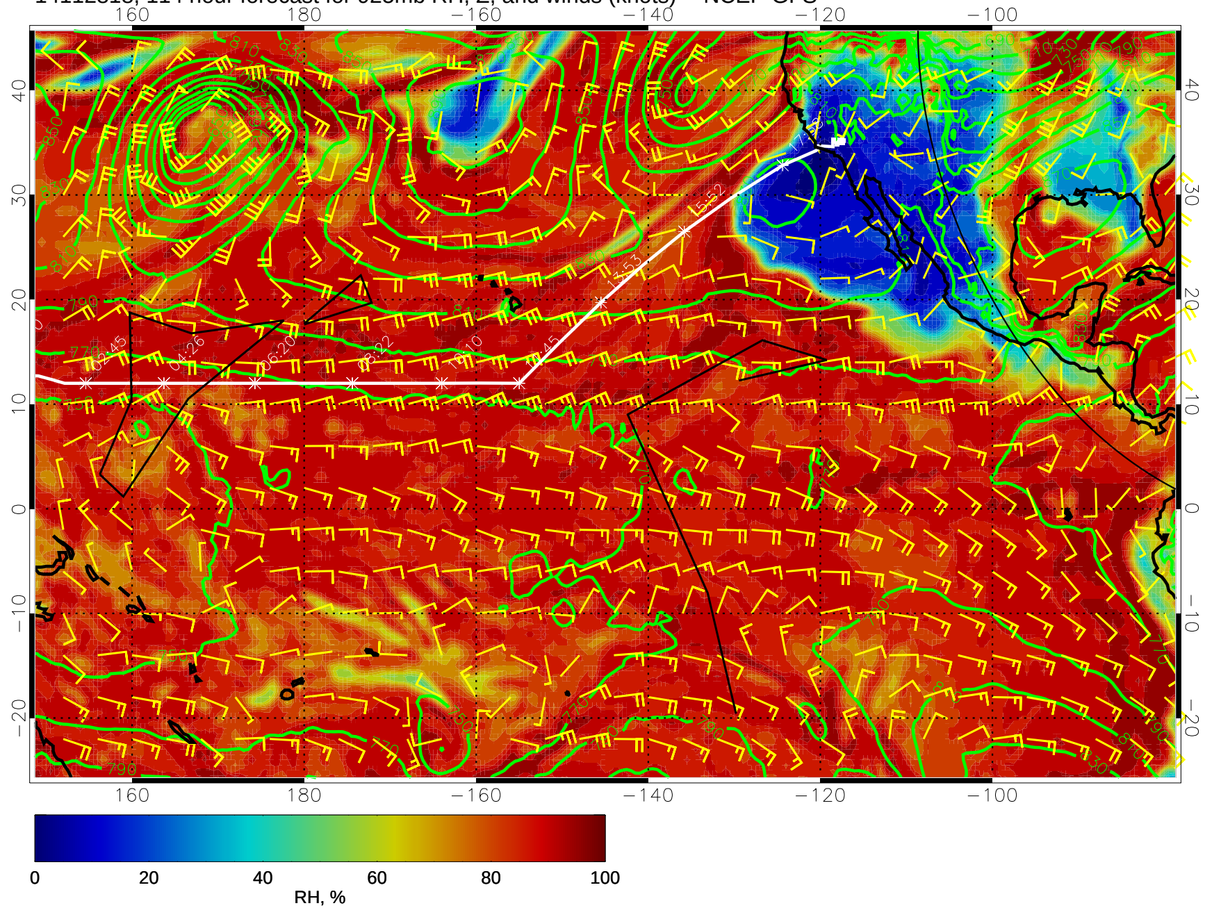
14112818, 114 hour forecast for 925mb RH, Z, and winds (knots) -- NCEP GFS
