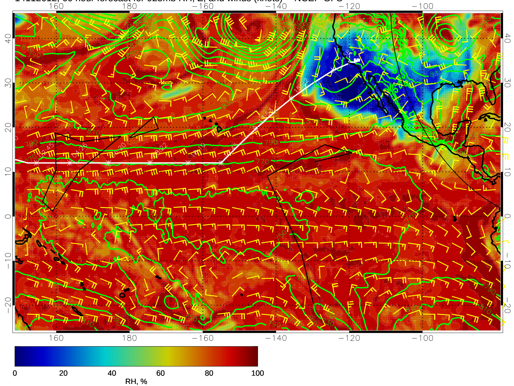
14112612, 60 hour forecast for 925mb RH, Z, and winds (knots) -- NCEP GFS
