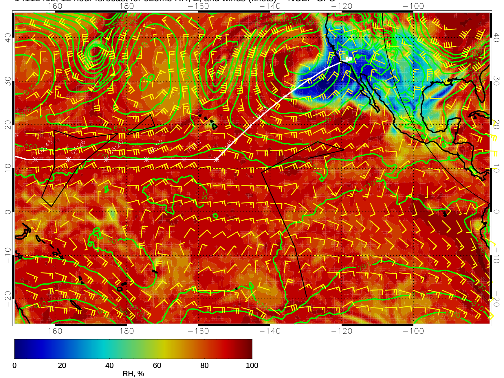
14112412, 12 hour forecast for 925mb RH, Z, and winds (knots) -- NCEP GFS
