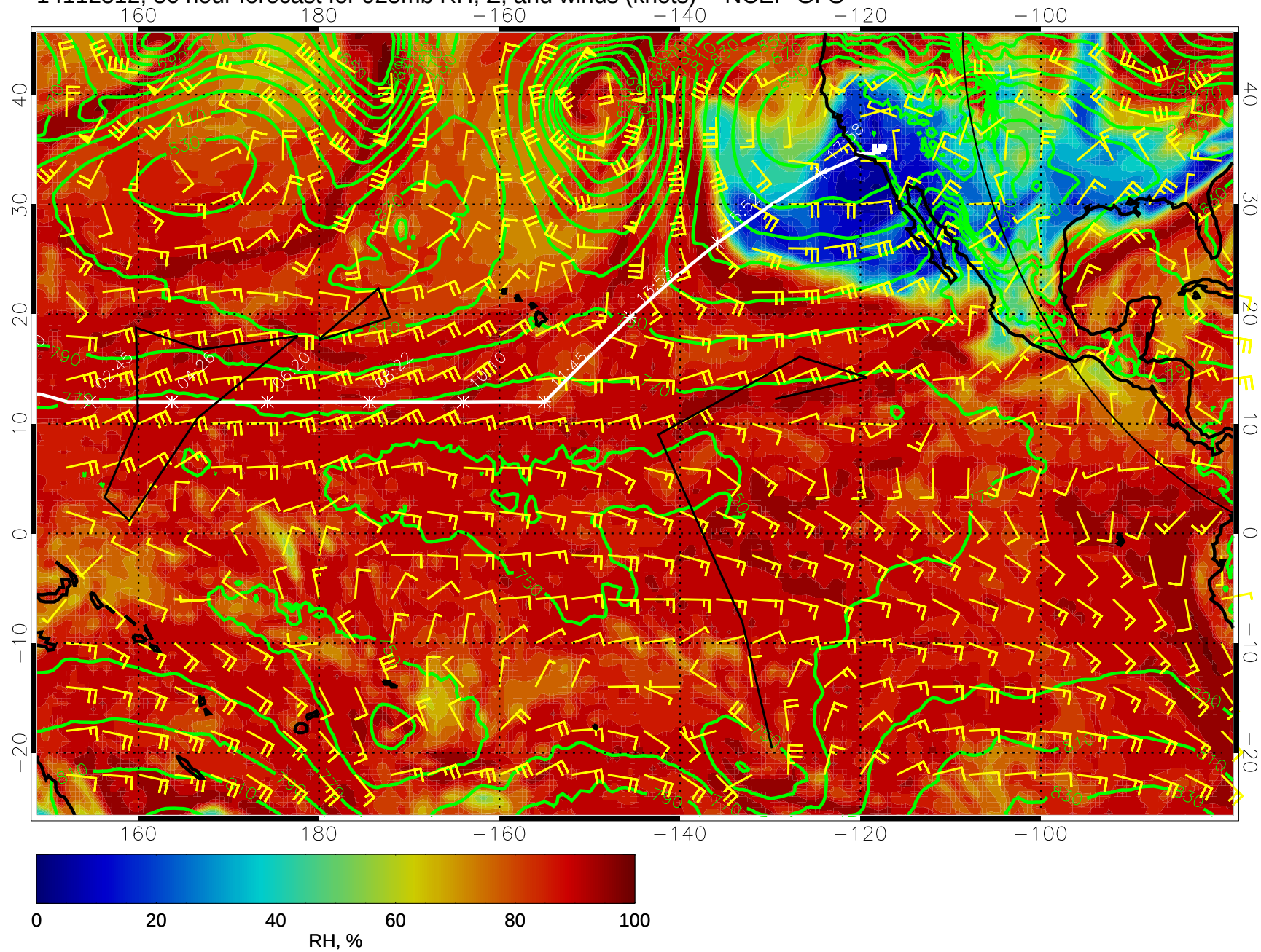
14112512, 36 hour forecast for 925mb RH, Z, and winds (knots) -- NCEP GFS
