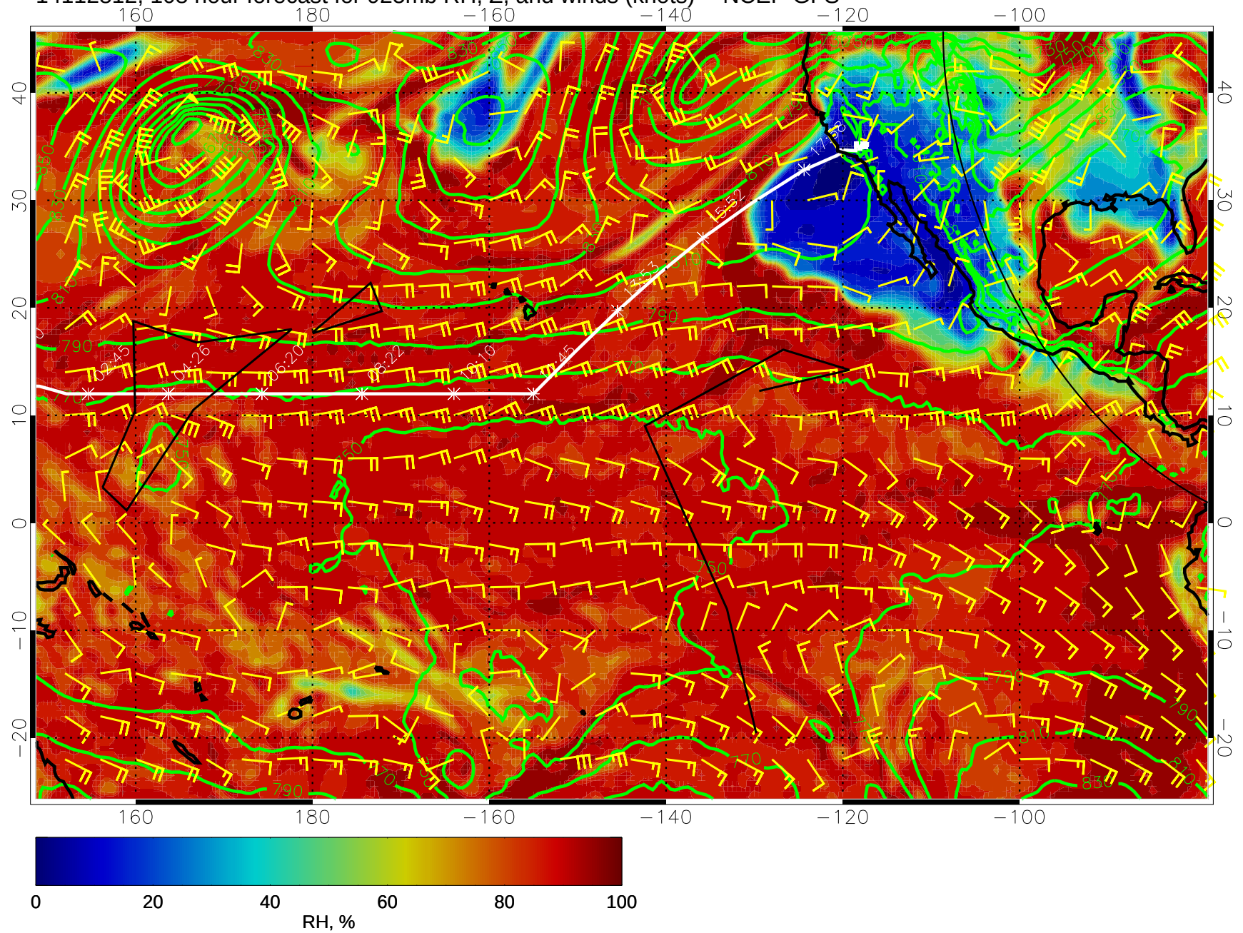
14112812, 108 hour forecast for 925mb RH, Z, and winds (knots) -- NCEP GFS
