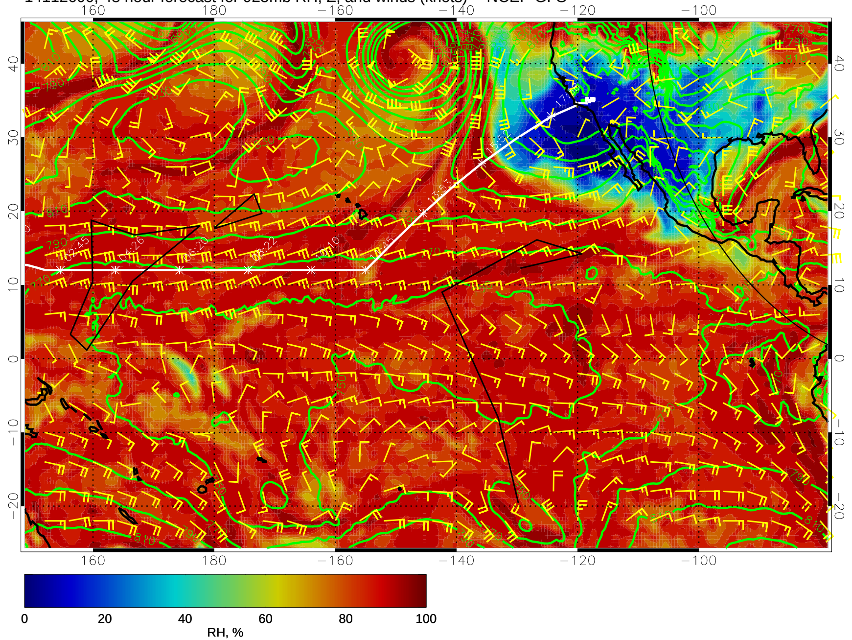
14112600, 48 hour forecast for 925mb RH, Z, and winds (knots) -- NCEP GFS
