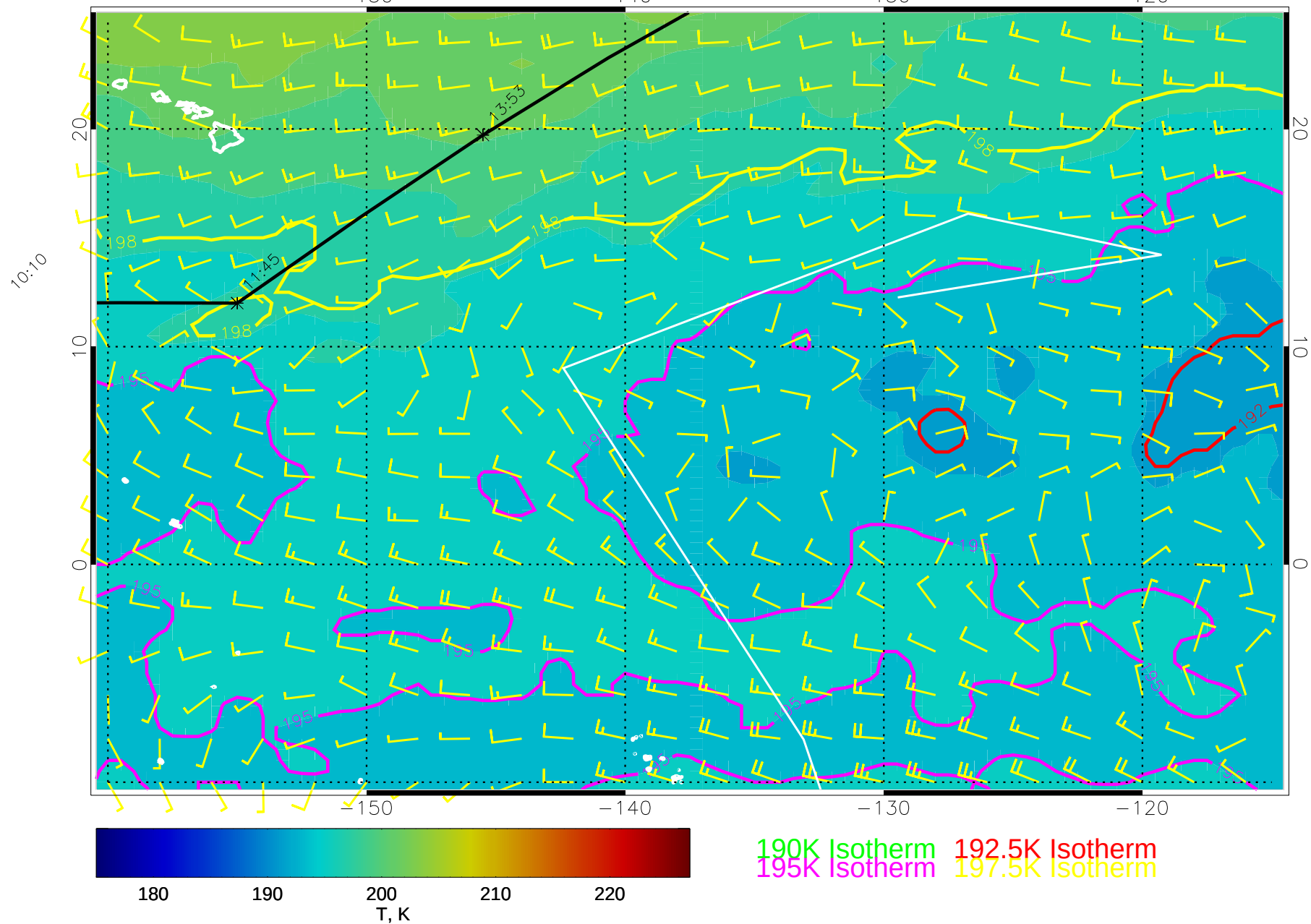
14112900, 120 hour forecast for 70mb T and winds (knots) -- NCEP GFS
