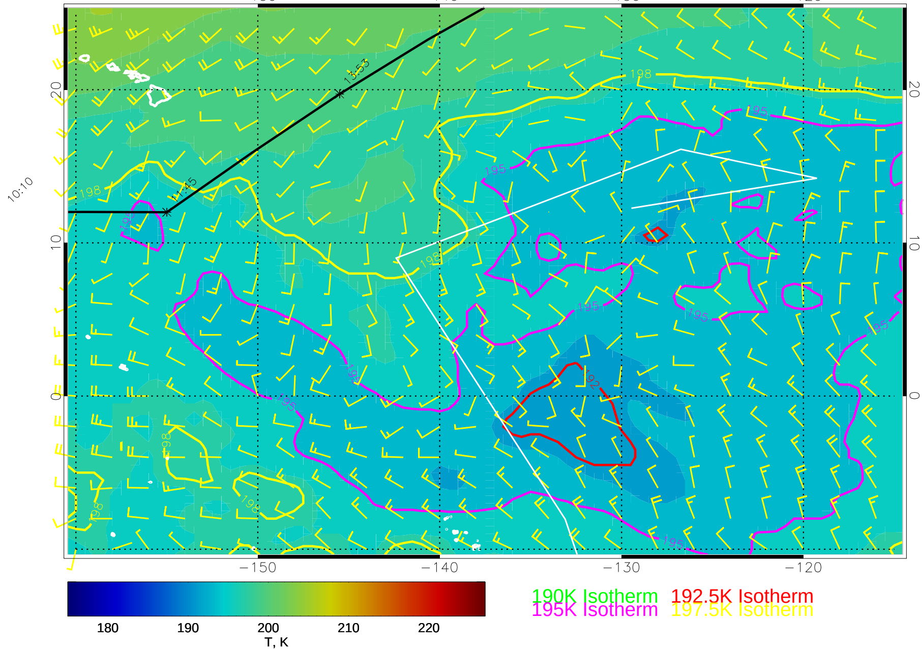
14112406, 6 hour forecast for 70mb T and winds (knots) -- NCEP GFS
