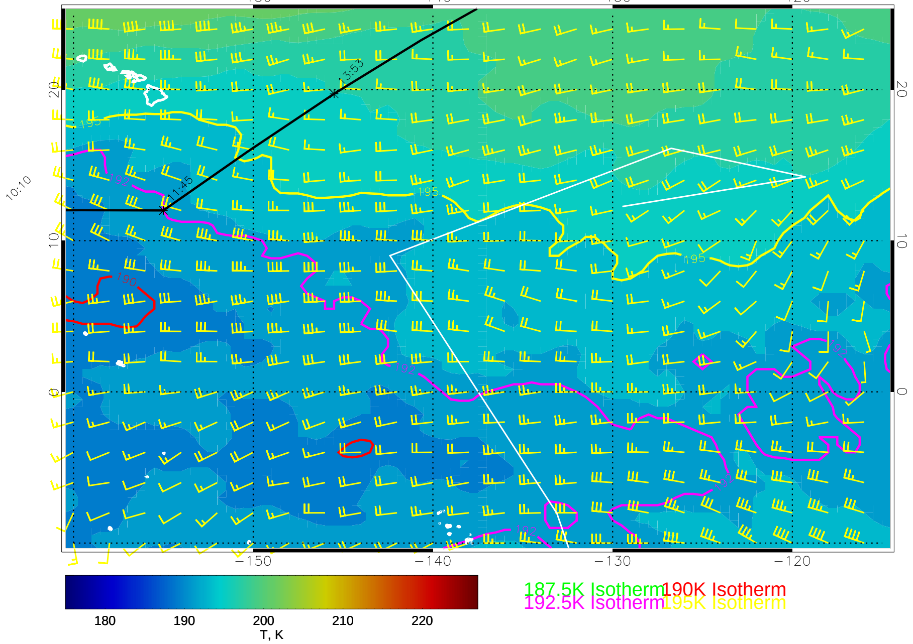
14112718, 90 hour forecast for 100mb T and winds (knots) -- NCEP GFS
